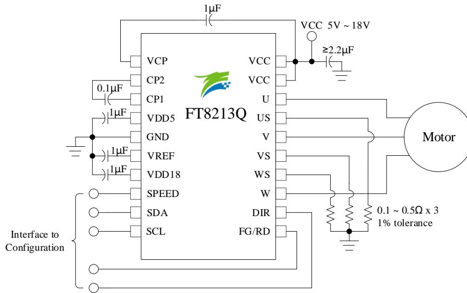
Figure 1-1 Typical Application Diagram of FT8213Q
