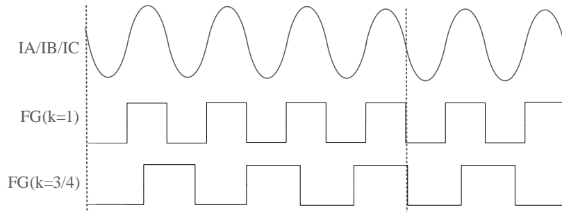
Figure 5-3 FG Output Waveform at k = 1 and k = 3/4
