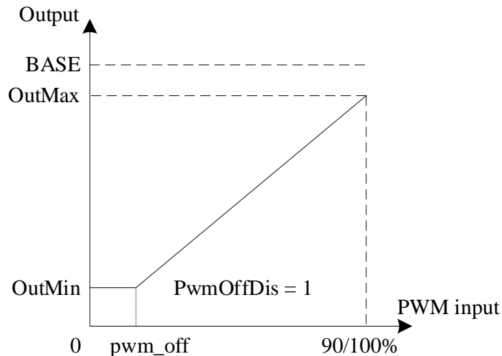
Figure 5-2 Output Curve at PwmOffDis = 1
