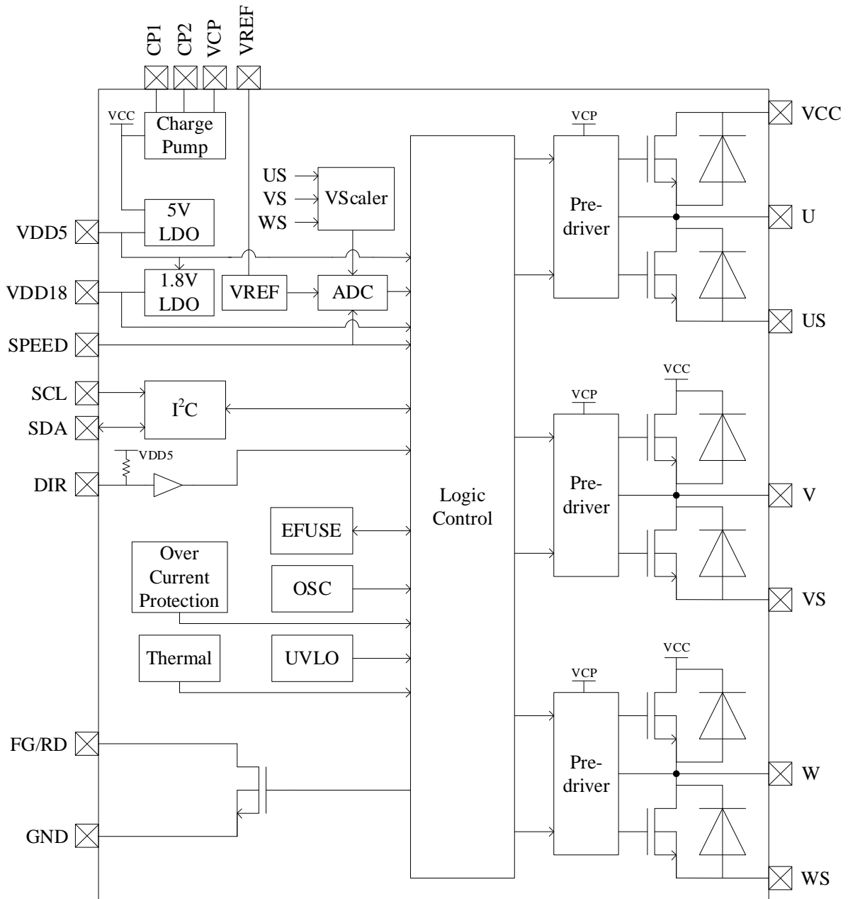
Figure 1-2 Functional Block Diagram of FT8213Q
