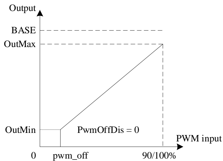
Figure 5-1 Output Curve at PwmOffDis = 0
