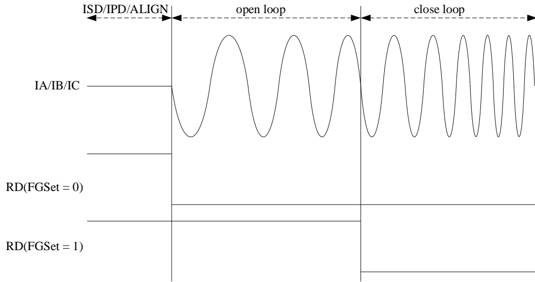
Figure 5-5 RD Output Waveform
