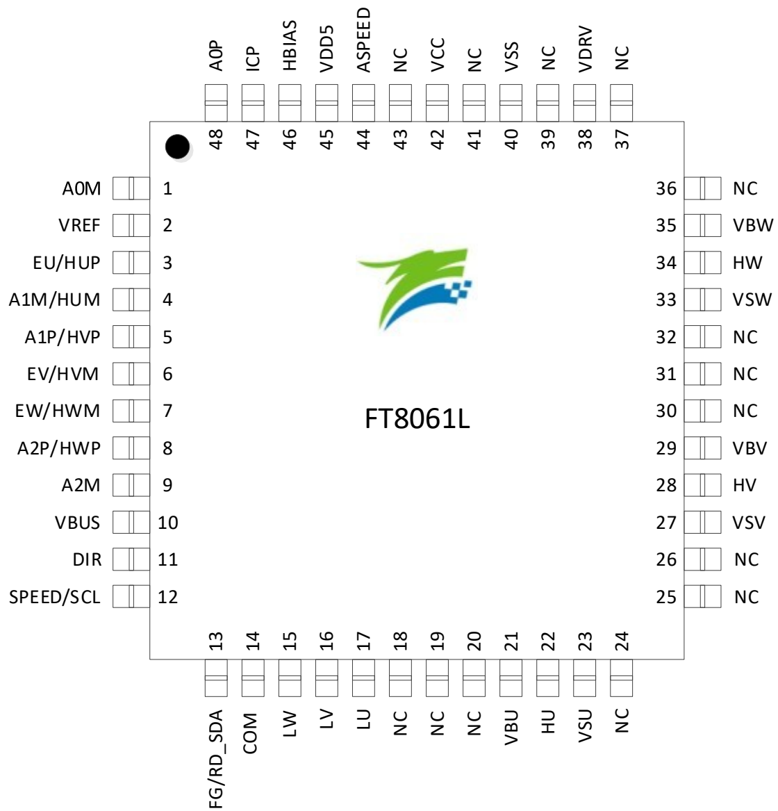
Figure 1-7 FT8061L LQFP48_7X7 Pinout Diagram
