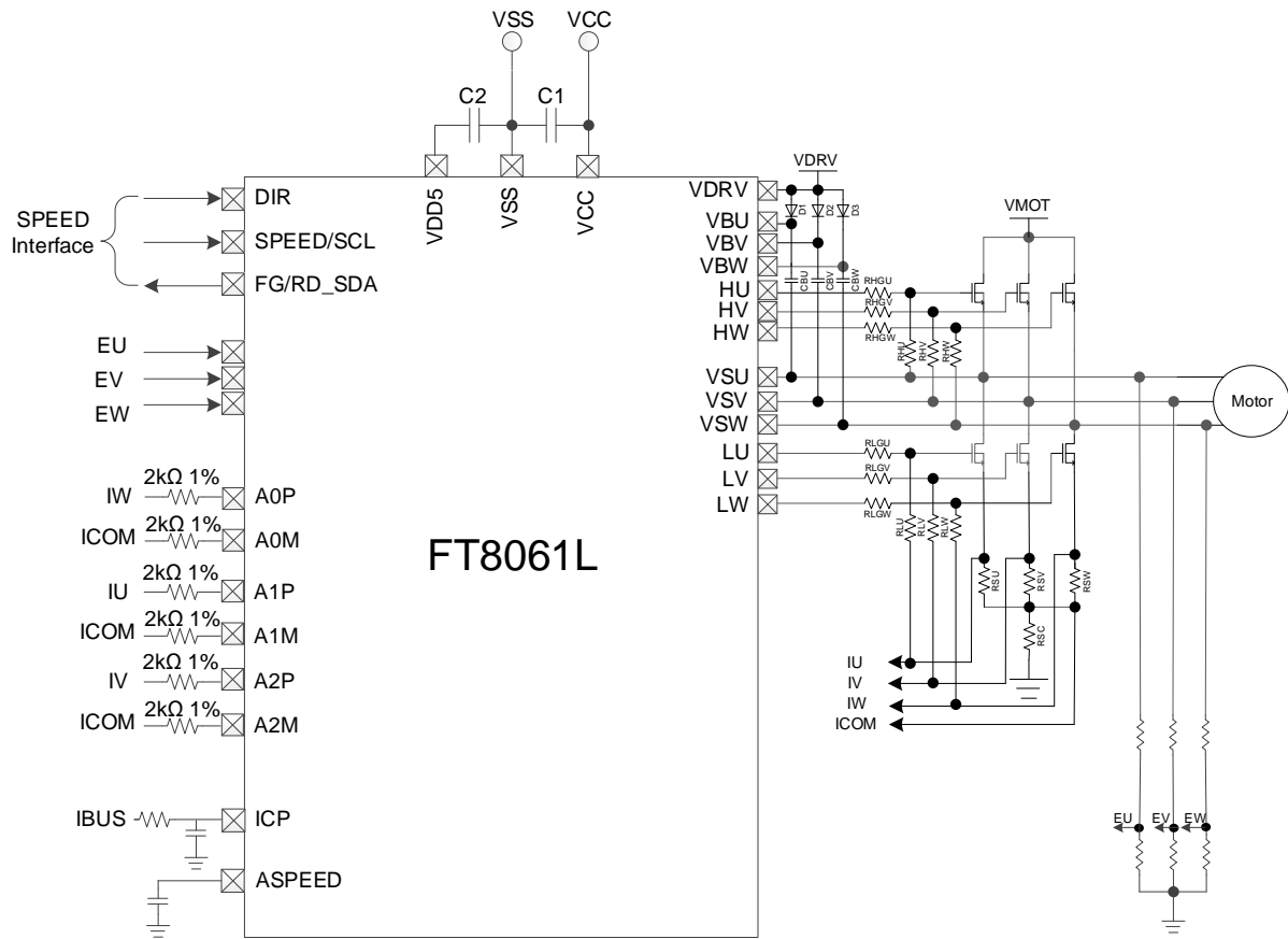
Figure 1-2 FT8061L in Sensorless FOC Mode with Dual/Triple-shunt Current Sampling
