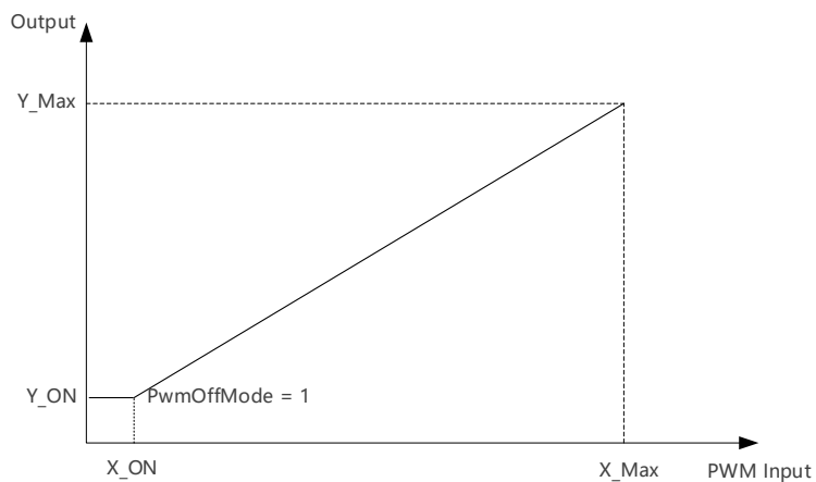
Figure 5-3 Output Curve in Speed-loop or Current-loop Mode (PwmOffMode = 1)
