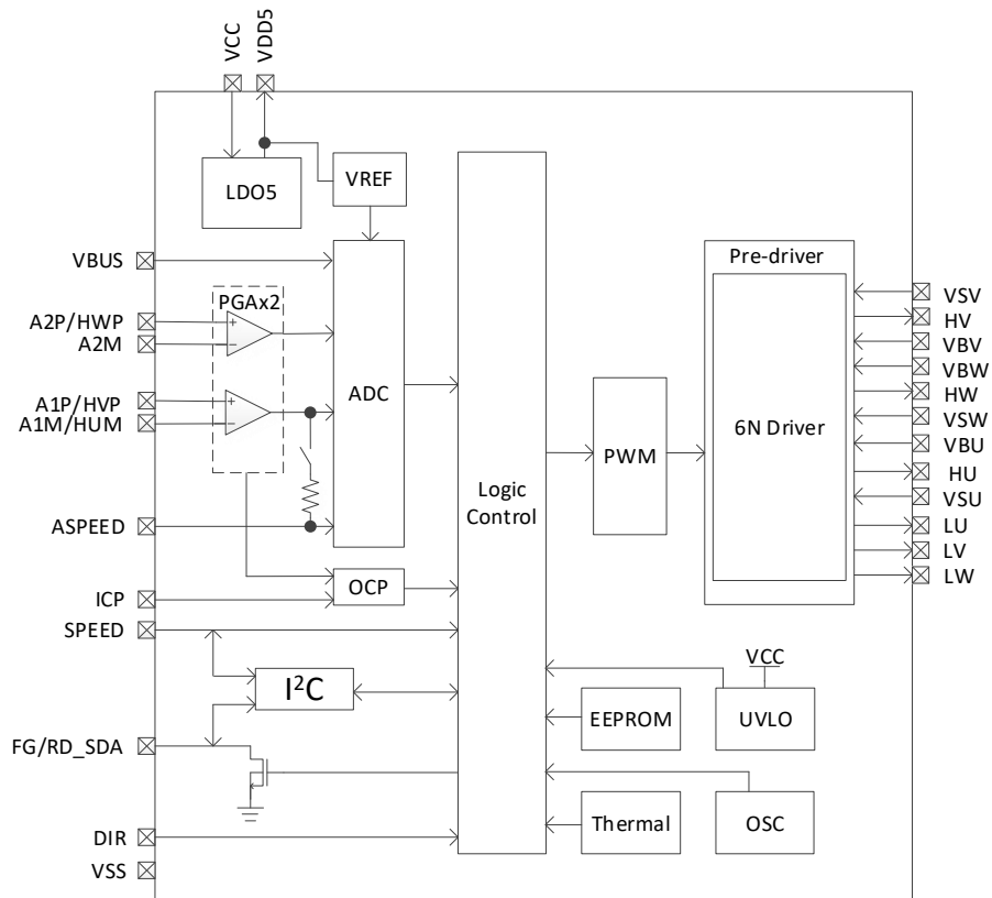
Figure 1-6 Functional Block Diagram of FT8061T
