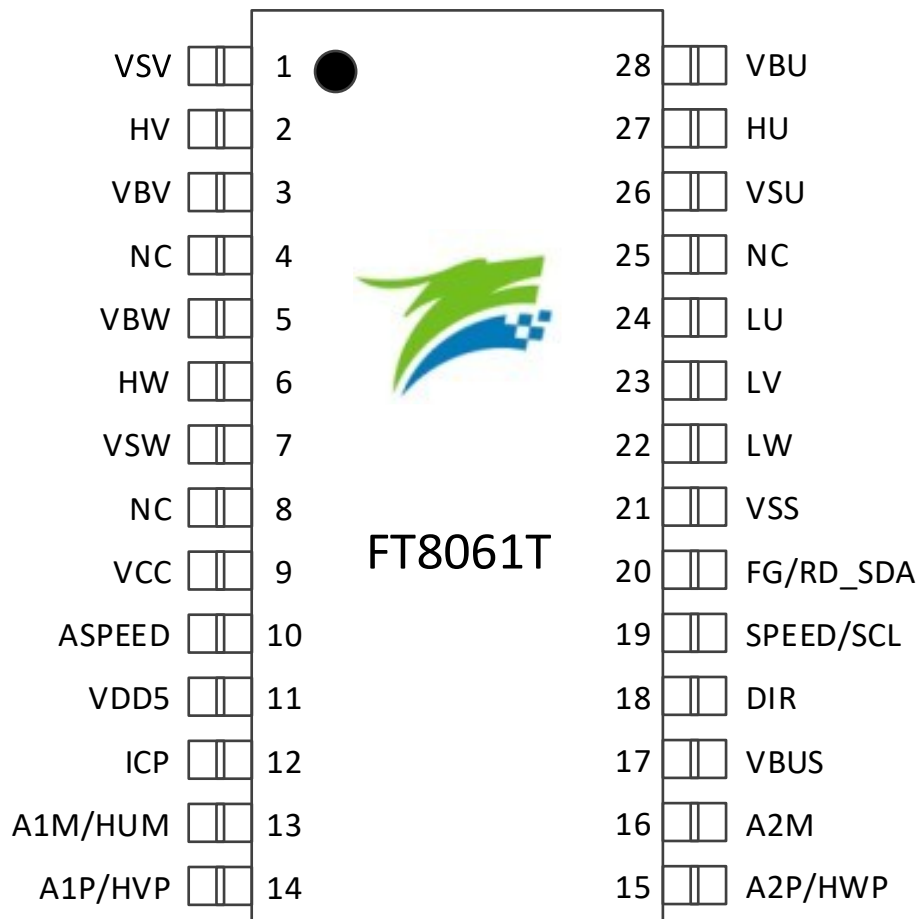
Figure 1-8 FT8061T TSSOP28_9.7X4.4 Pinout Diagram
