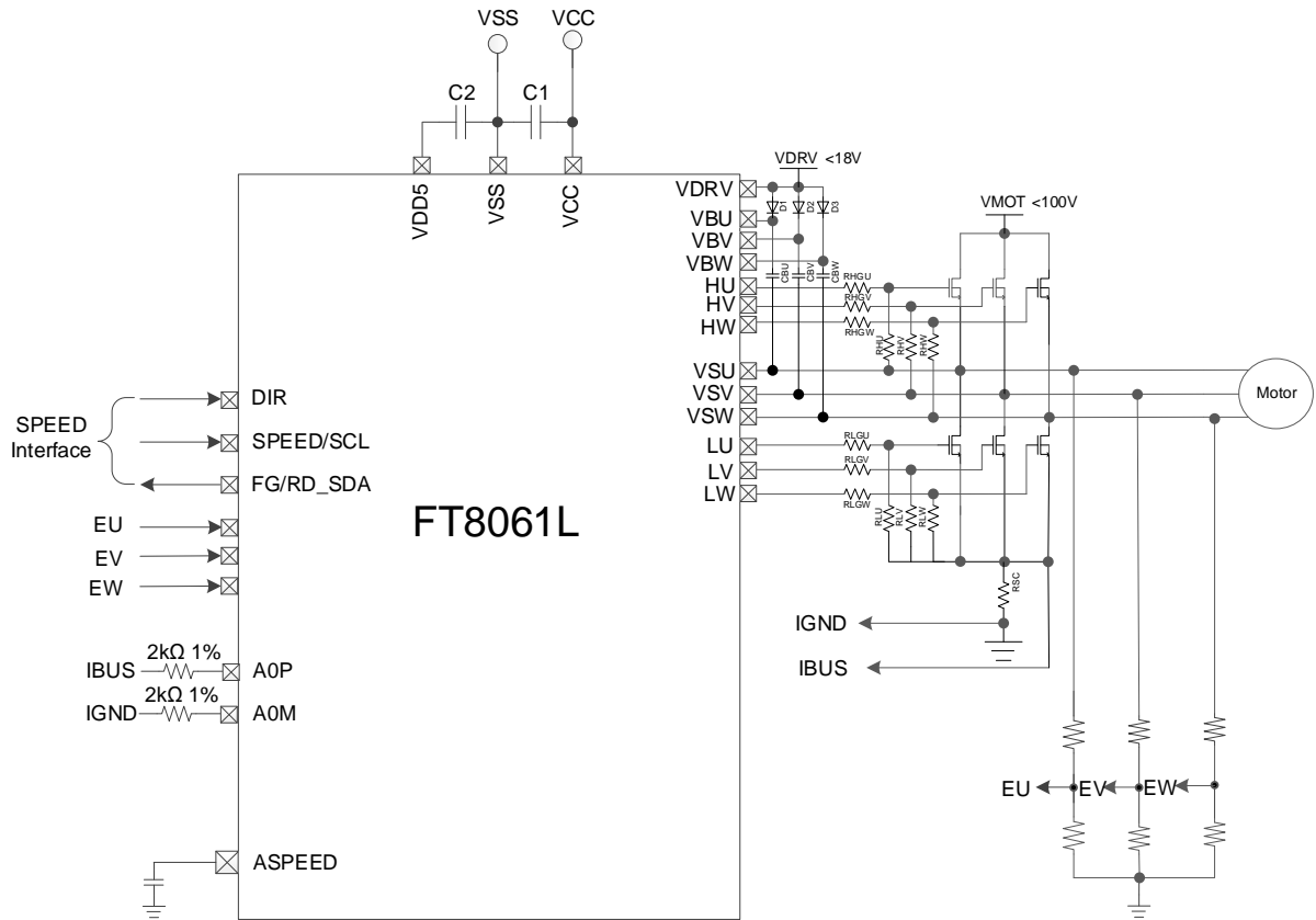
Figure 1-3 FT8061L in Sensorless FOC Mode with Single-shunt Current Sampling
