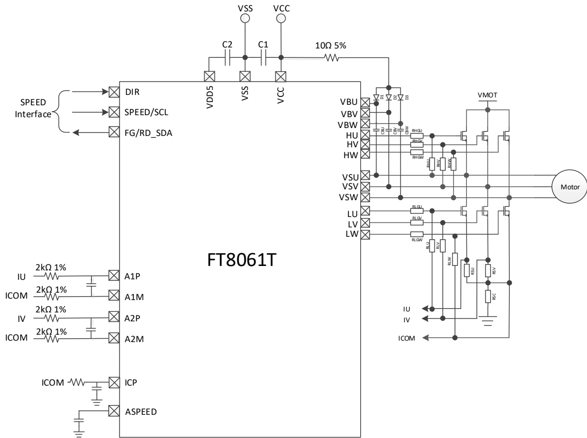
Figure 1-4 FT8061T in Sensorless FOC Mode with Dual-shunt Current Sampling
