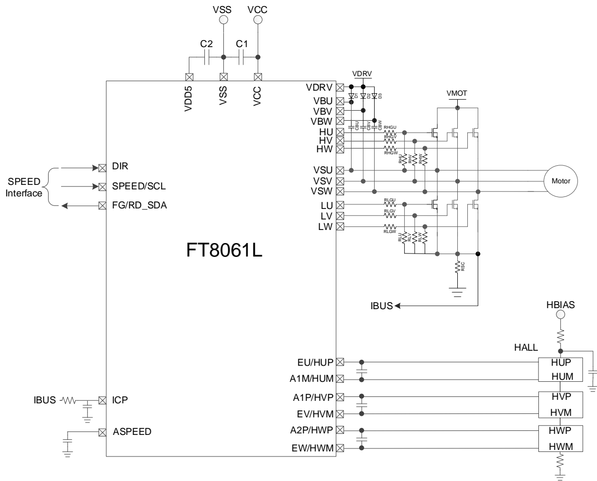
Figure 1-1 FT8061L in Sensor-based SVPWM Mode
