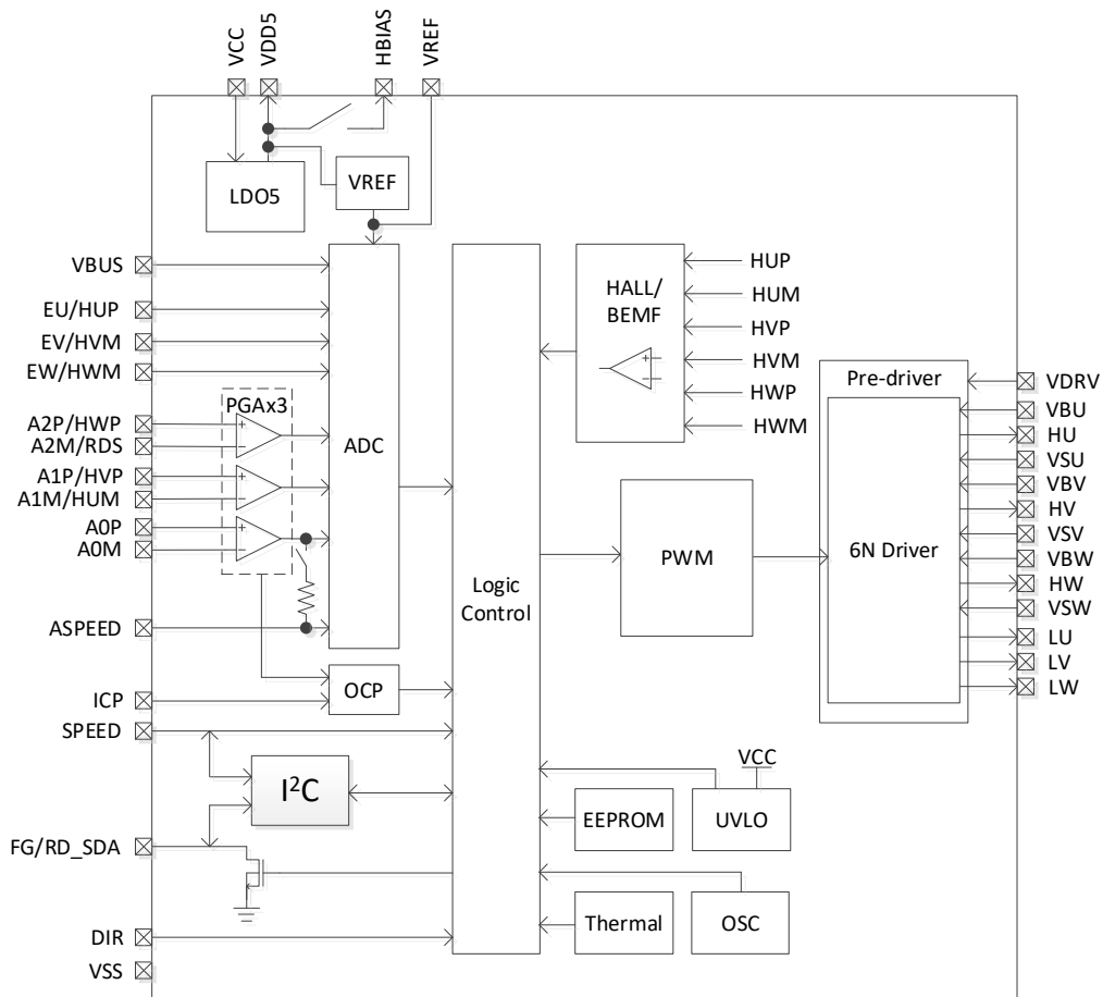
Figure 1-5 Functional Block Diagram of FT8061L
