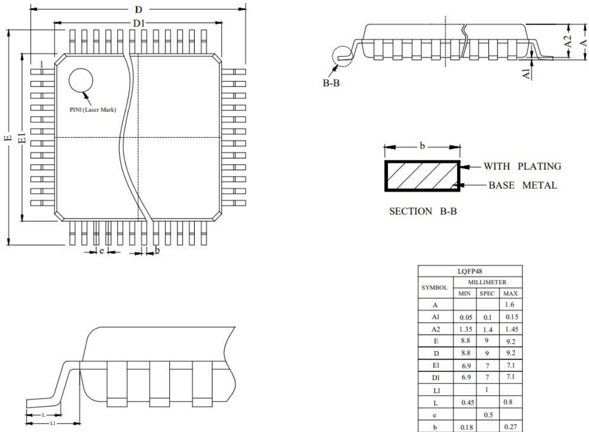
Figure 2-1 FT8061L LQFP48_7X7 Package Drawings and Dimensions
