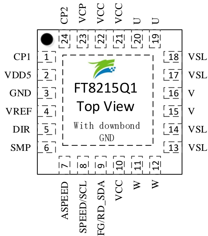
Figure 1-4 Pinout Diagram of FT8215Q1 QFN24
