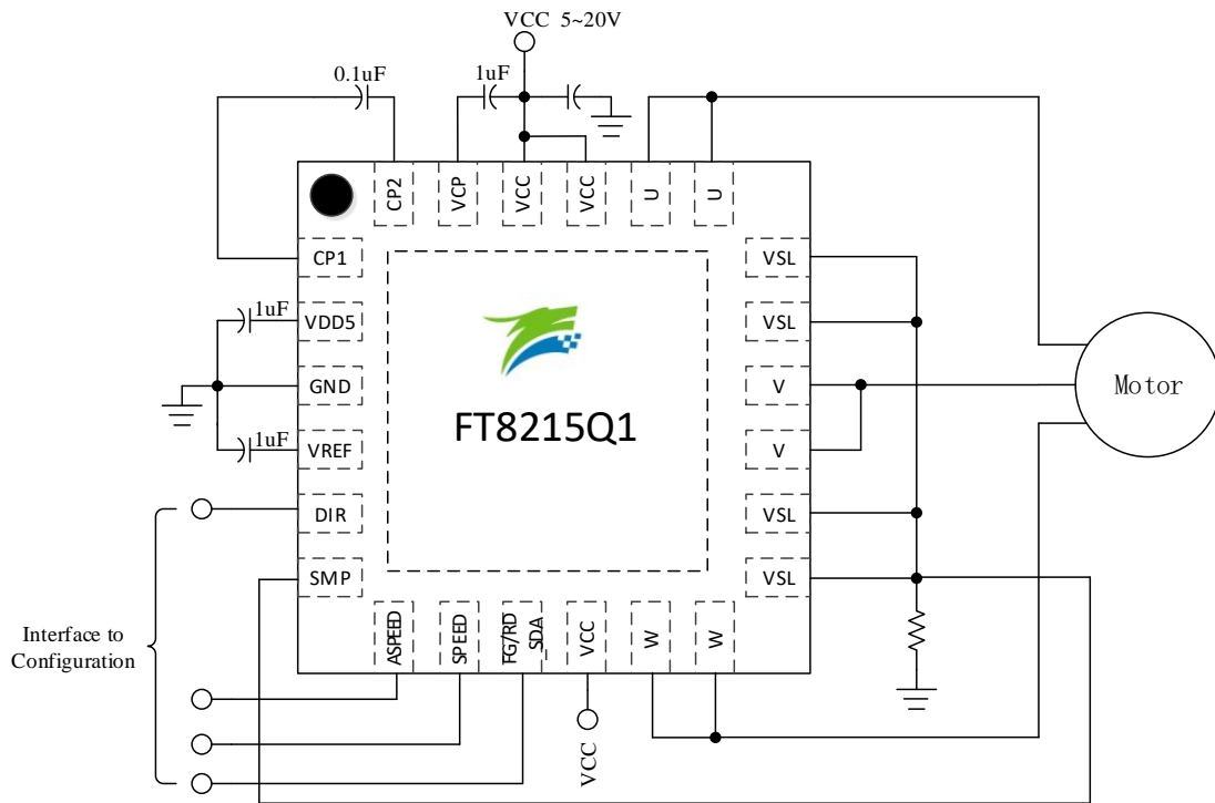
Figure 1-1 Typical Application Diagram of FT8215Q1 (Single-shunt Current Sampling)
