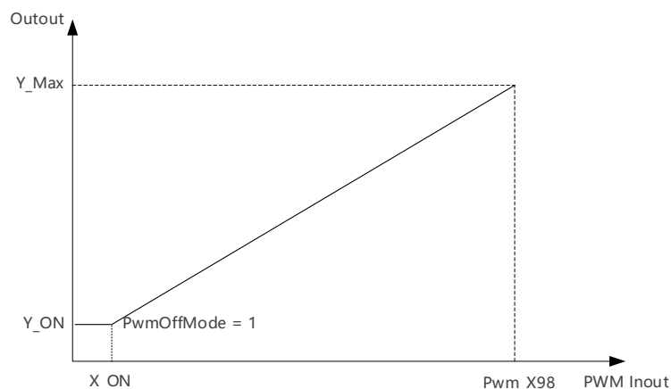
Figure 5-4 Output Curve in Speed/Current Control Mode (PwmOffMode = 1)
