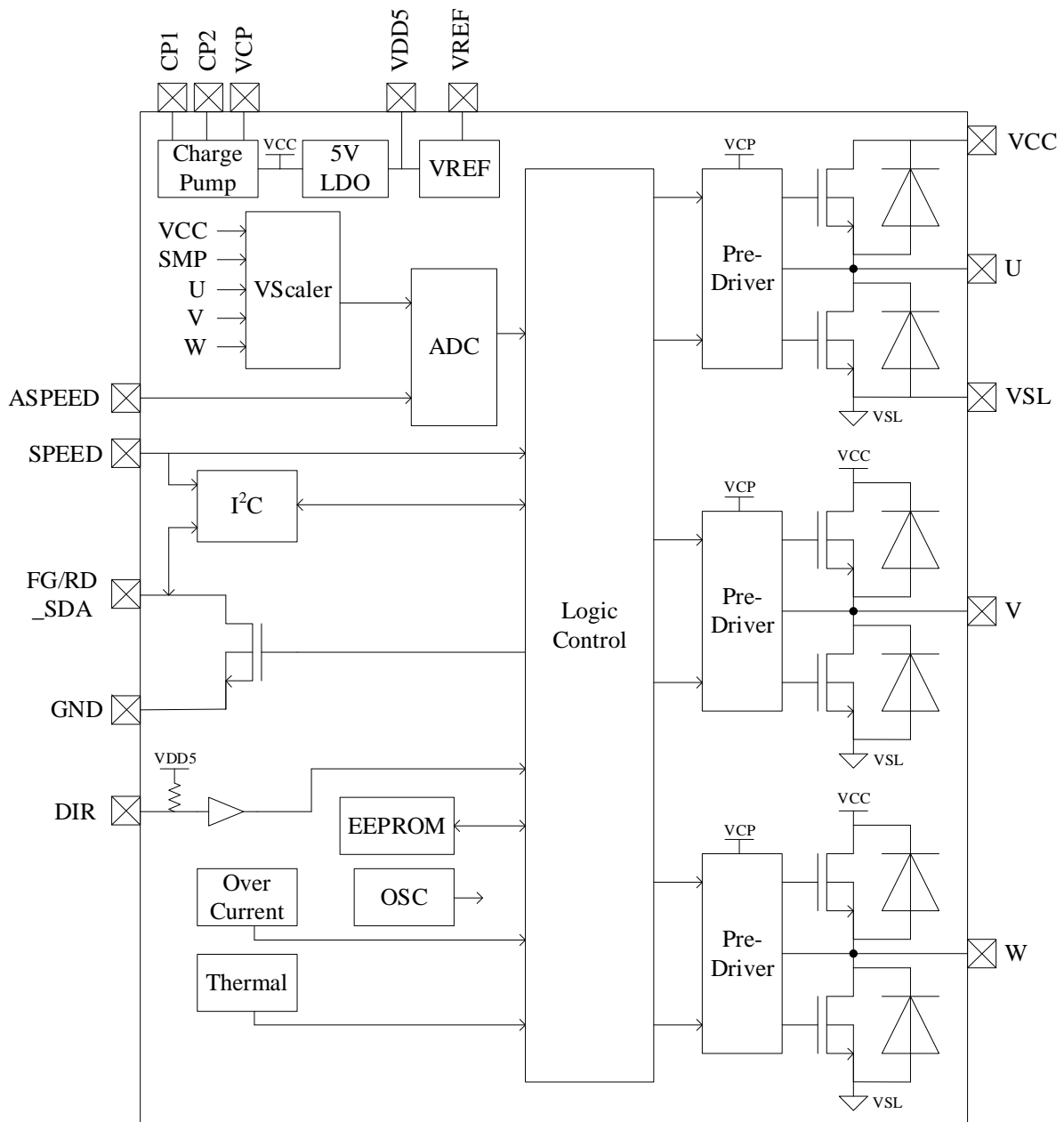
Figure 1-3 Functional Block Diagram of FT8215Q1
