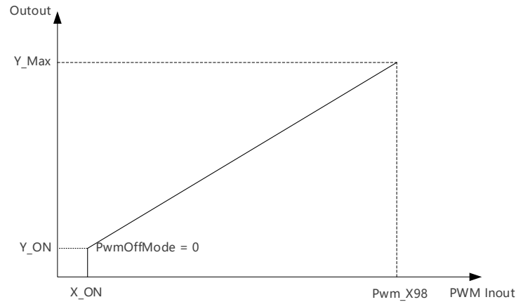
Figure 5-3 Output Curve in Speed/Current Control Mode (PwmOffMode = 0)
