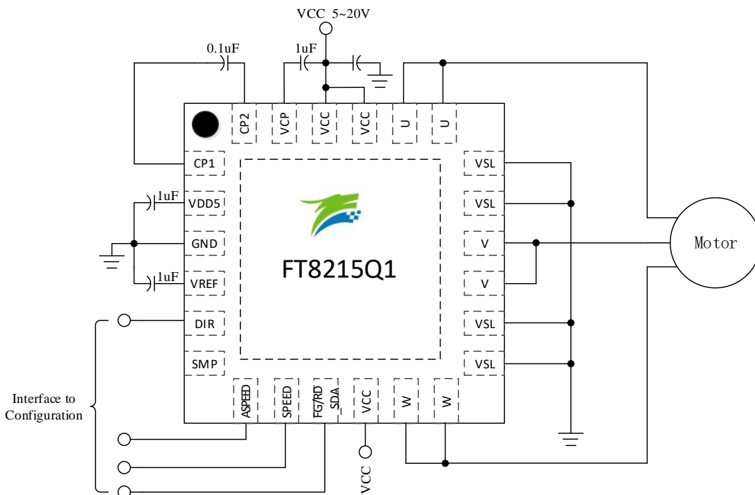
Figure 1-2 Typical Application Diagram of FT8215Q1 (Dual/Triple-shunt Current Sampling)
