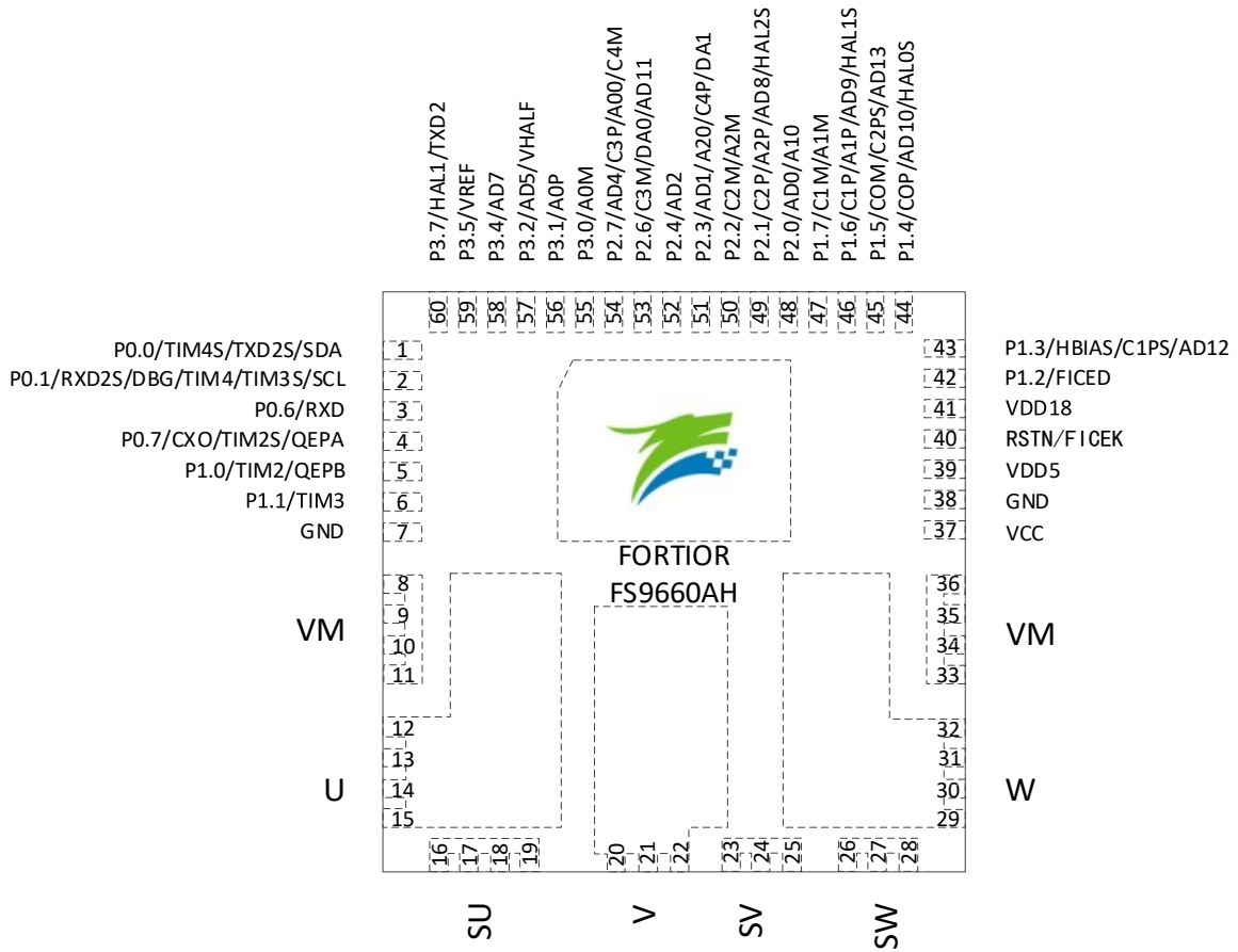
Figure2-1 FS9660AH QHFBP8080-60L Pinout Diagram
