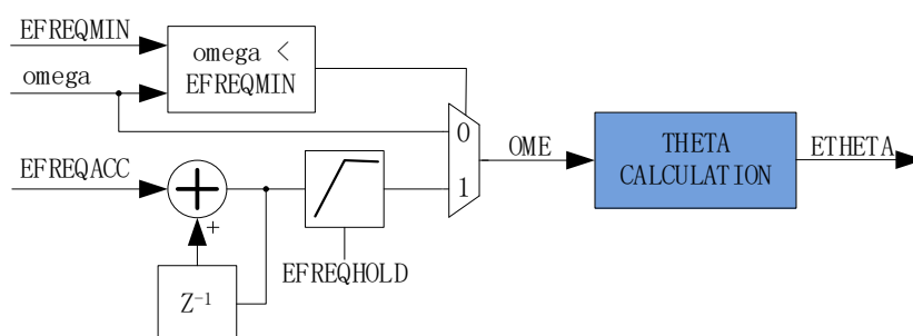
Figure 12-14 Schematic Block Diagram of Forced Angle of Estimator
