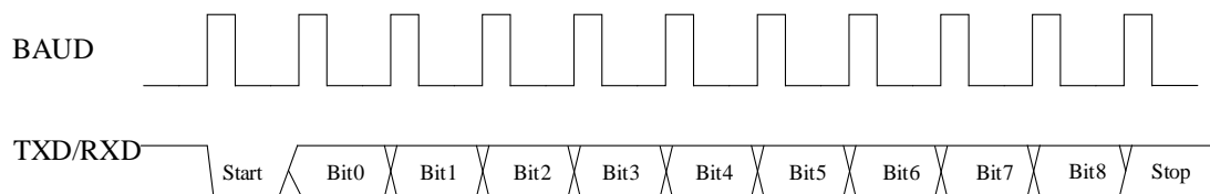
Figure 9-4 UART Communication Timing Diagram
