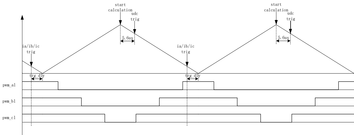
Figure 12-12 Dual/Triple-Shunt Alternating Current Sampling Mode
