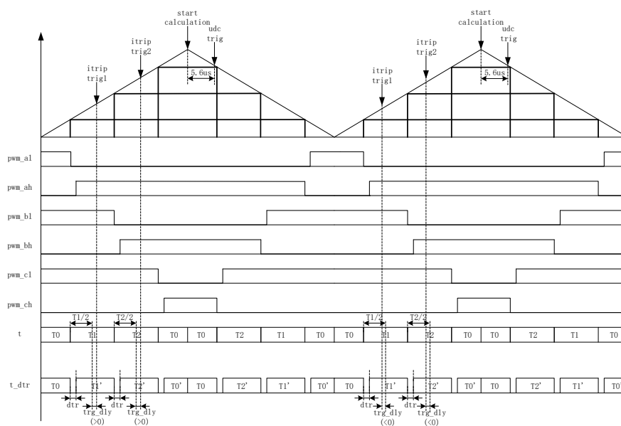
Figure 12-9 Single-shunt Current Sampling Timing Diagram
