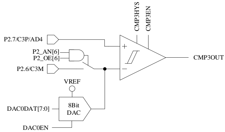
Figure 27-2 Single-comparator Input Mode
