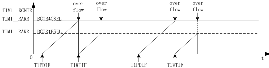
Figure13-4 Waveform of Reload Timer
