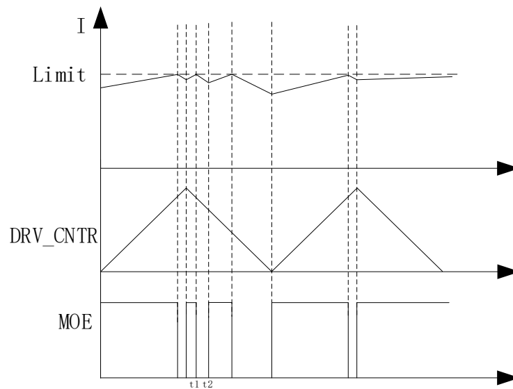
Figure 27-6 Cycle-by-Cycle Current Limiting Waveform ( t_2 - t_1 = 5\mu\text{s} ) when \text{EVT\_FILTER}[\text{MOEMD}] = 11
