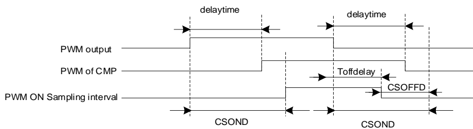
Figure14-11 PWM ON Sampling mode
