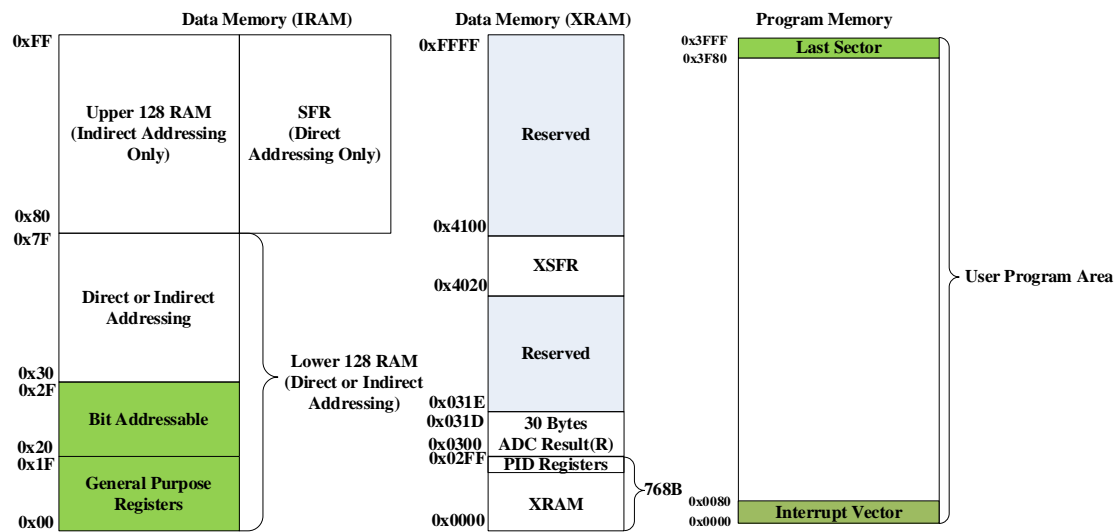
Figure 1-2 Memory Organization
