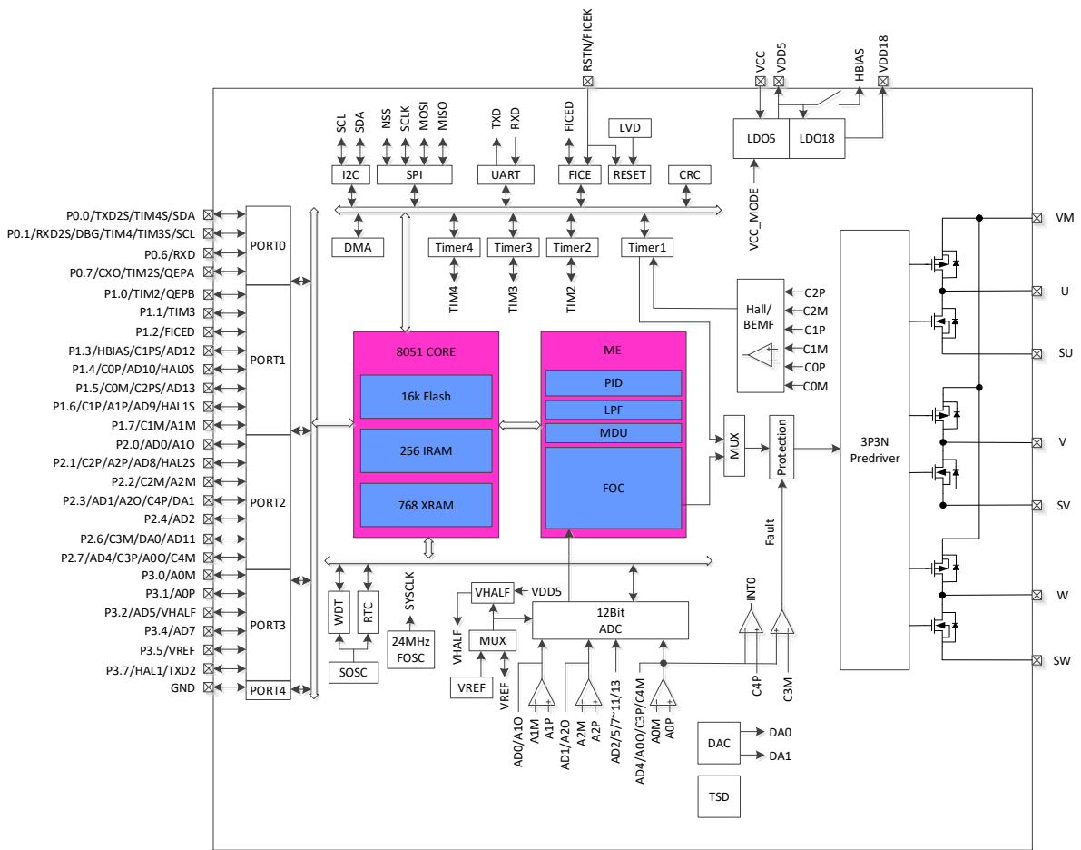
Figure 1-1 Functional Block Diagram of FS9660AH
