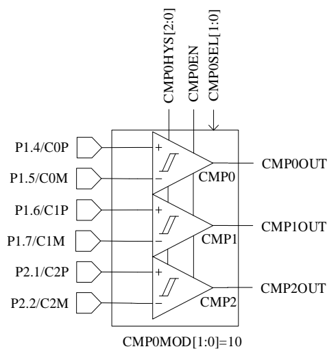
Figure 27-11 CMPG Mode with Three Differential Comparators
