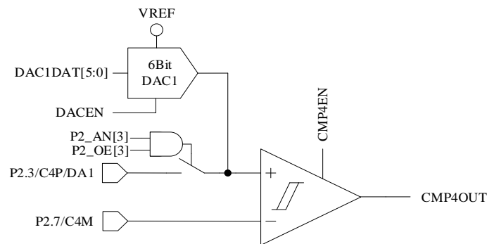
Figure 27-7 Schematic Diagram of CMP4 Module
