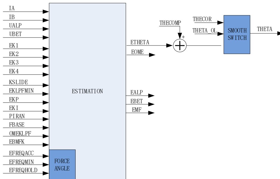
Figure 12-13 Schematic Block Diagram of Estimator
