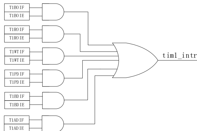
Figure13-10 Timer1 Interrupt Sources
