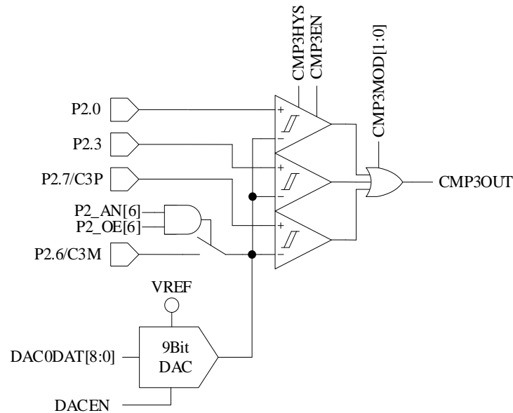
Figure 27-1 CMP3 Input and Output Pins
