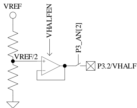
Figure 25-1 Diagram of VHALF Module Input and Output
