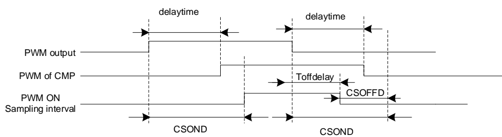
Figure 27-13 PWM ON Sampling Mode
