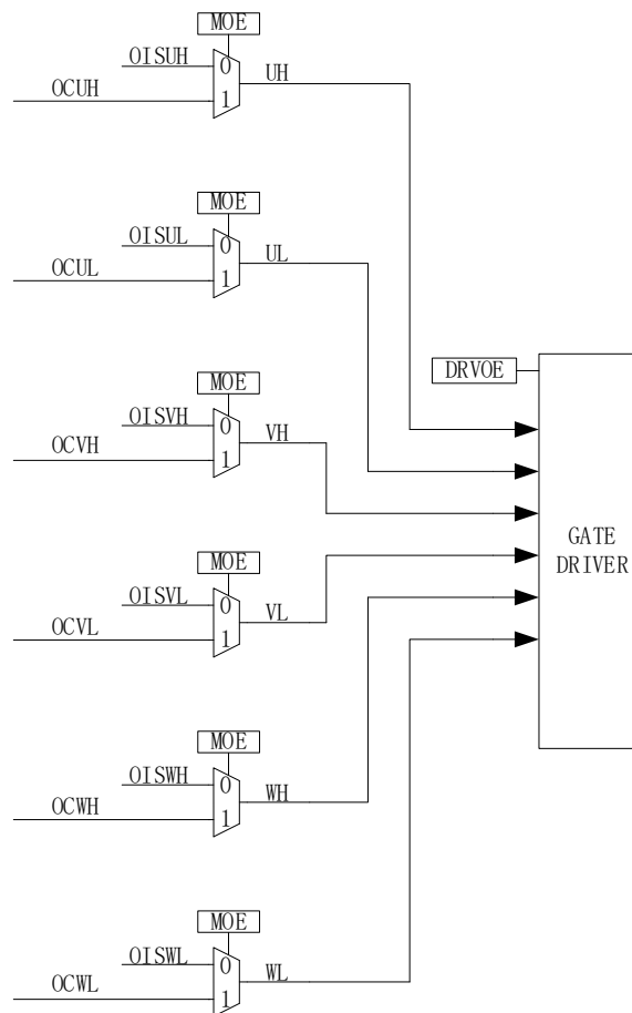
Figure 17-8 Block Diagram of Rear Stage of Output Control Module
