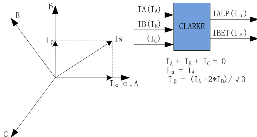
Figure 12-3 Clarke Transformation
