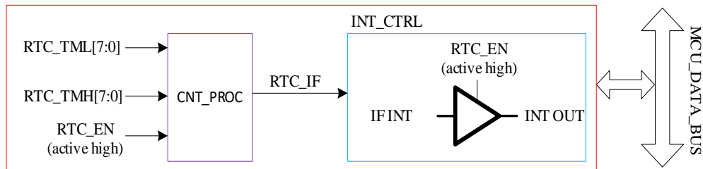
Figure19-1 RTC Functional Block Diagram
