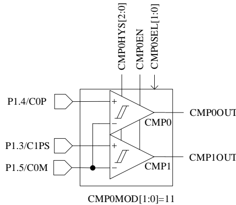
Figure 27-12 CMPG Mode with Two Comparators
