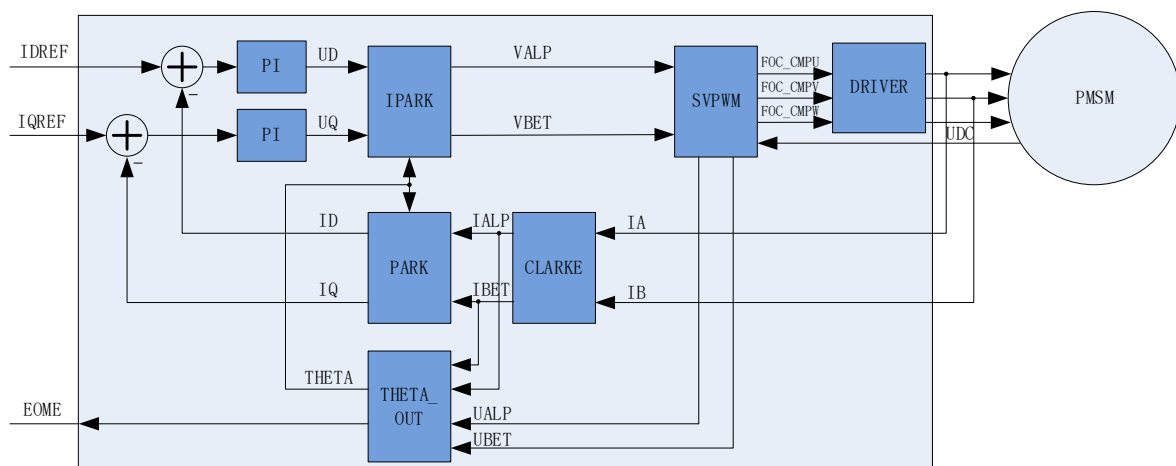
Figure 12-1 Schematic Diagram of FOC
