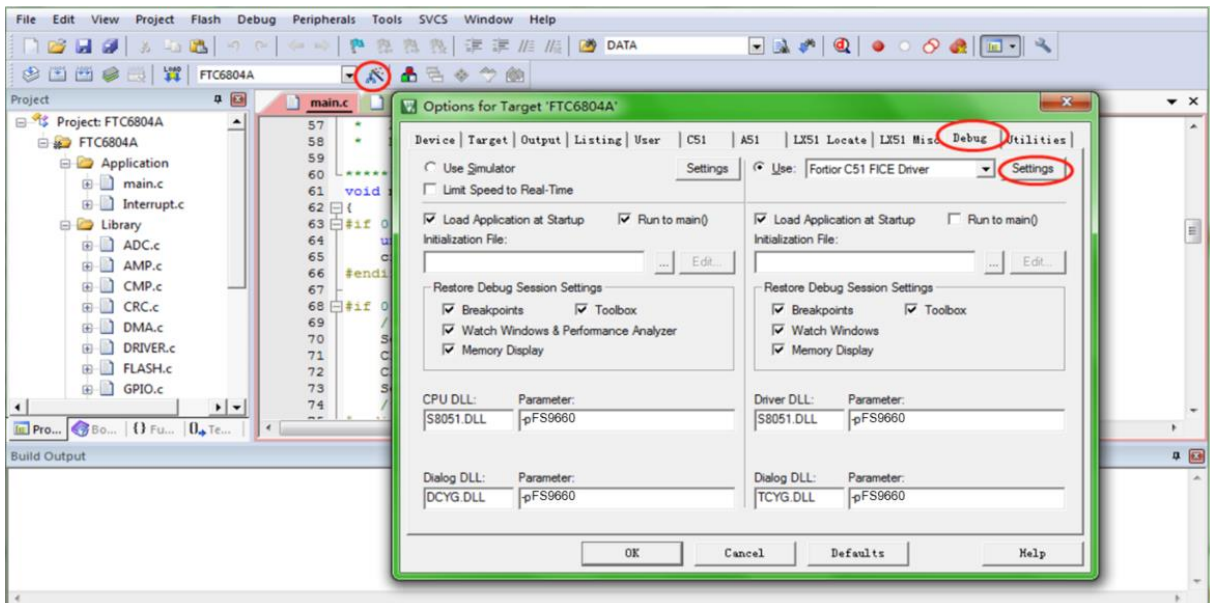
Figure 32-1 Code Protection Configurations
