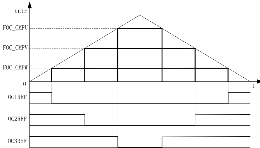
Figure 17-3 PWM Generation Diagram
