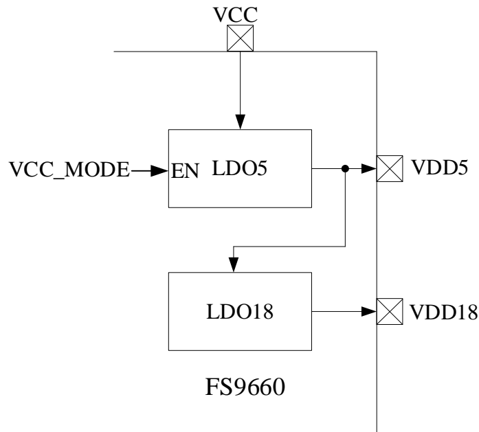
Figure 28-1 Functional Block Diagram of Power Supply
