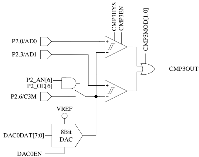
Figure 27-3 Dual-comparator Input Mode
