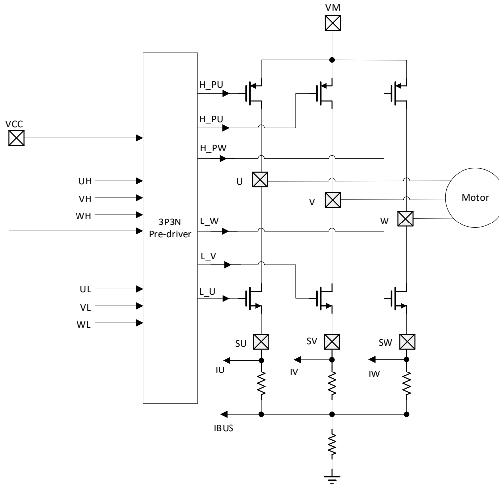
Figure 17-1 Block Diagram of Pre-driver Module
