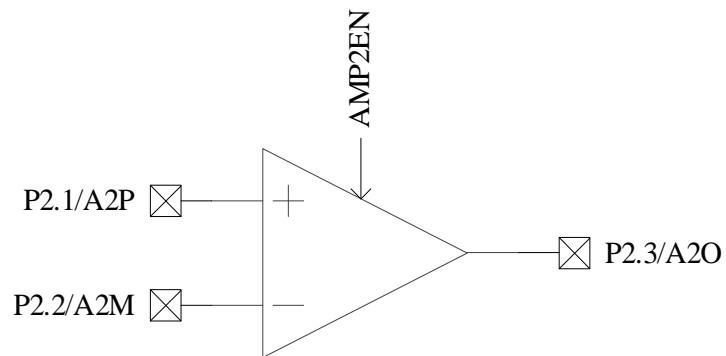
Figure 26-5 Diagram of AMP2 Input and Output
