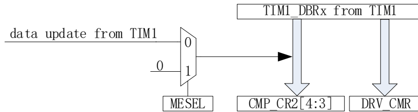
Figure 17-5 Timer1 Automatically Controls DRV_CMx and CMP_CR2[4:3]
