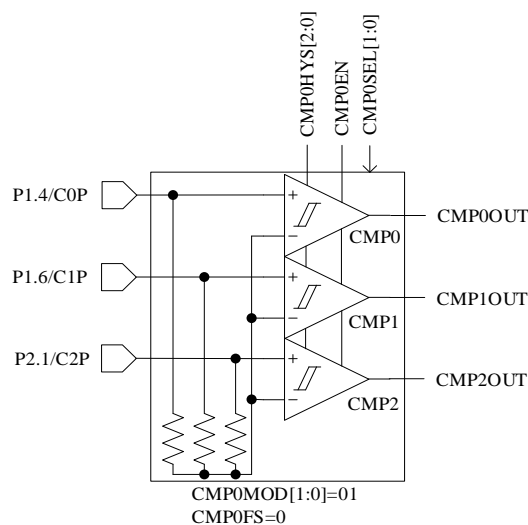
Figure 27-9 CMPG Mode with Built-in Three Comparators and Resistors (without Function Switching)
