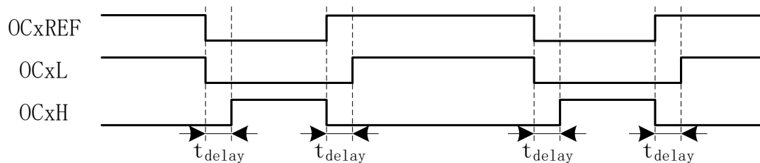
Figure 17-4 Complementary Output with Deadtime Insertion
