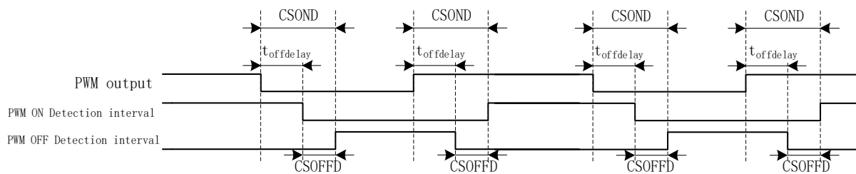
Figure13-7 Timing Diagram of Sampling
