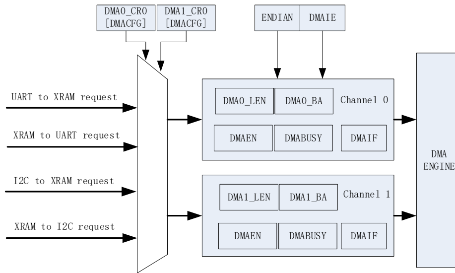
Figure 23-1 Functional Block Diagram of DMA
