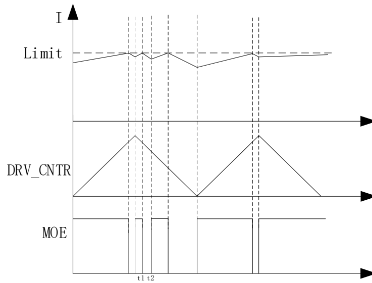
Figure 27-5 Cycle-by-Cycle Current Limiting Waveform ( t_2 - t_1 = 10\mu\text{s} ) when \text{EVT\_FILTER}[\text{MOEMD}] = 10
