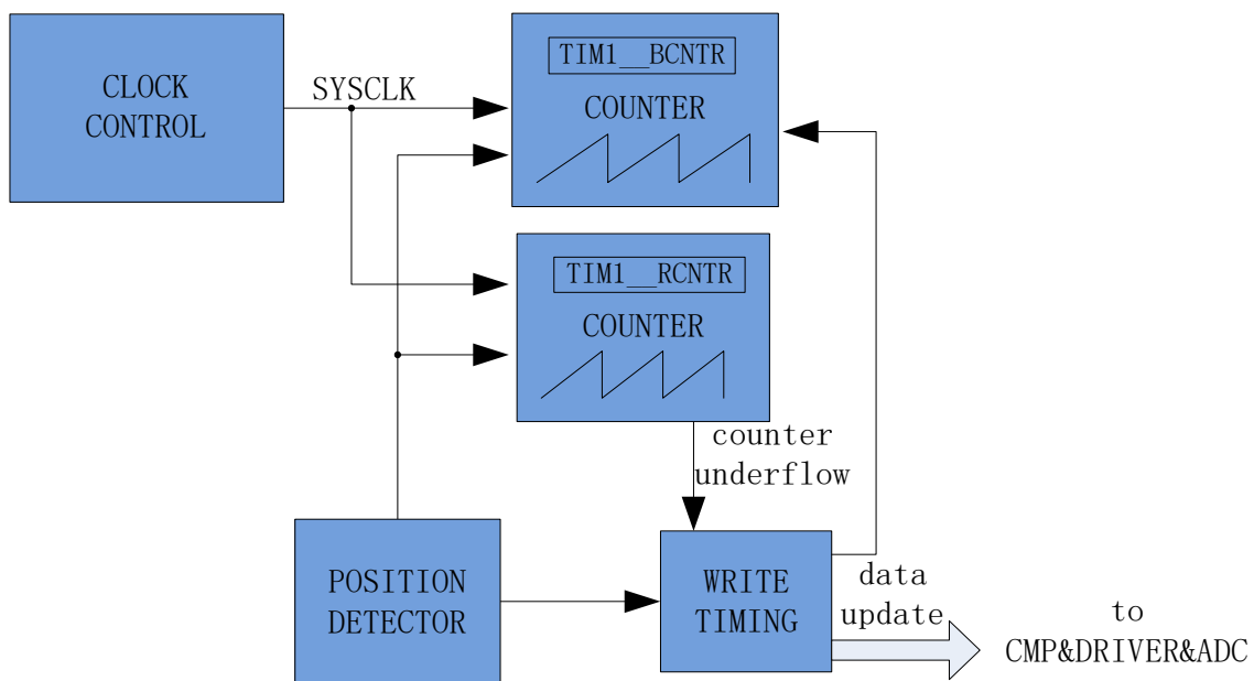
Figure13-1 Internal Structure of Timer1
