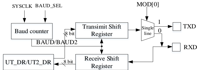
Figure 9-3 UART Block Diagram
