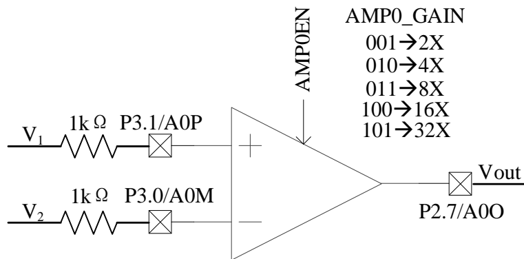
Figure 26-3 Diagram of AMP0 PGA Differential Input Mode
