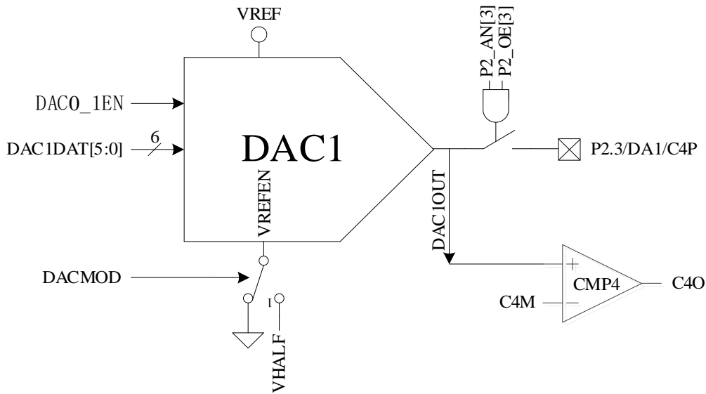
Figure 22-2 Functional Block Diagram of DAC1
