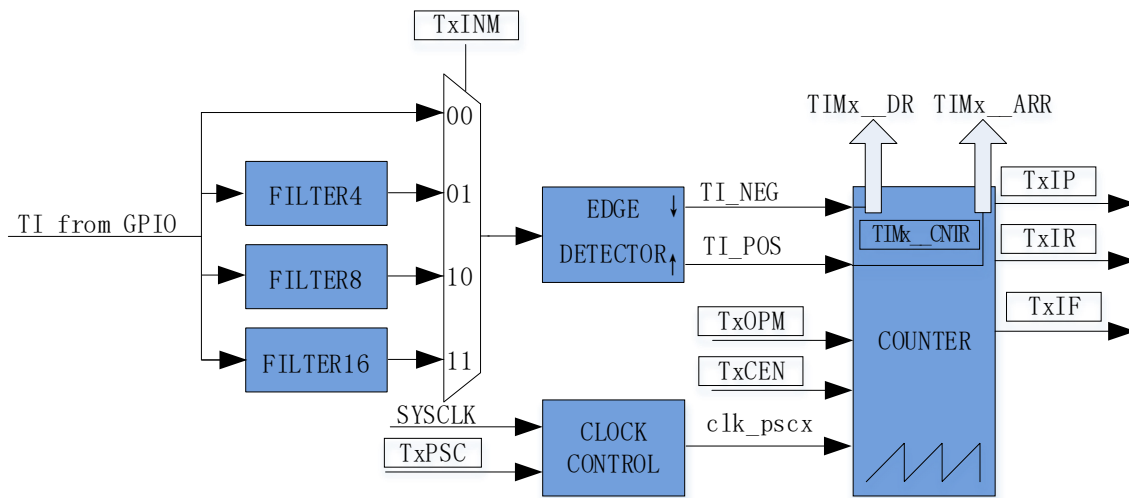
Figure 15-5 Schematic Block Diagram of Input Capture Mode
