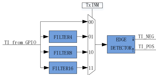
Figure15-3 Block Diagram of Input Signal Filtering and Edge Detection
