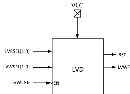
Figure 28-3 LVD Module
