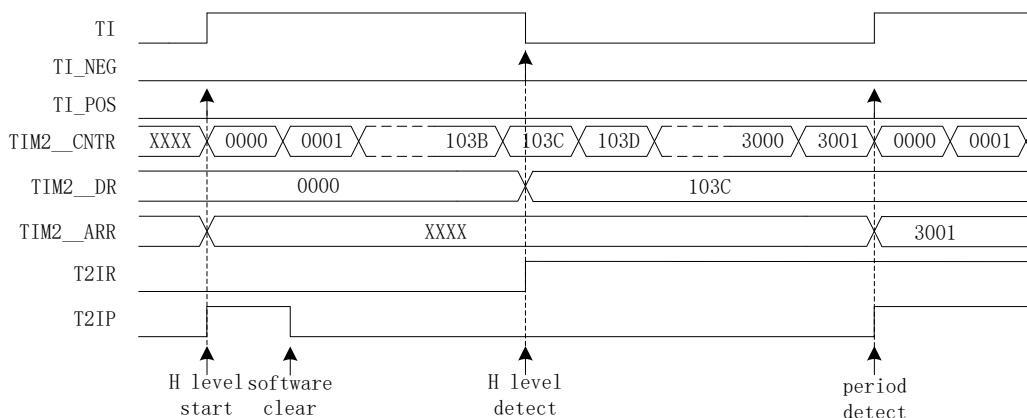
Figure14-6 Timing Diagram of Input Capture Mode ( TIM2\_CR0[T2CES] = 0 )
