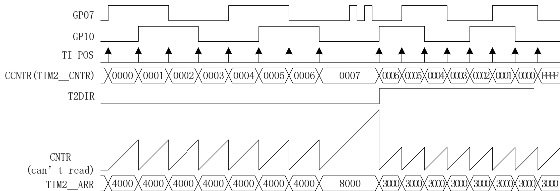
Figure14-10 Timing Diagram of QEP & RSD Mode
