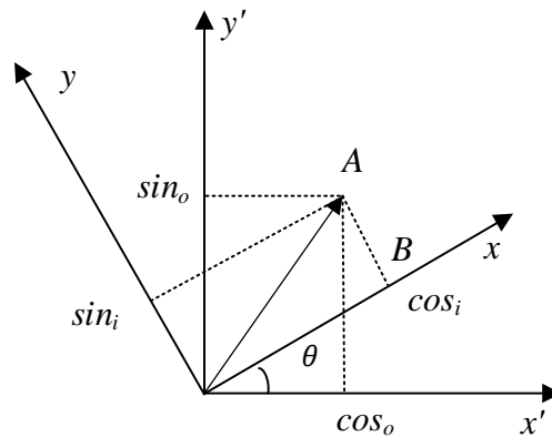
Figure 10-1 Coordinate Transformation
