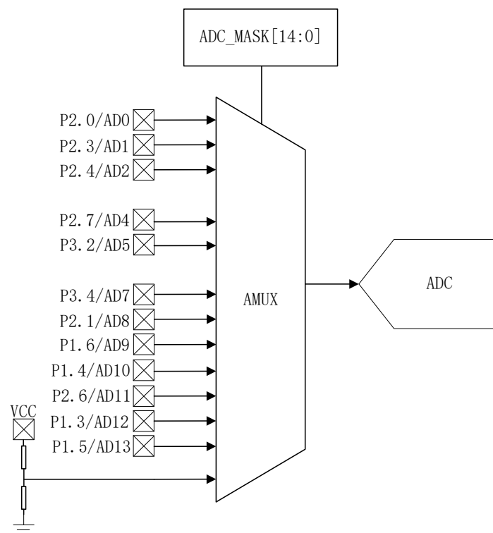
Figure21-1 ADC Multiplexer Block Diagram
