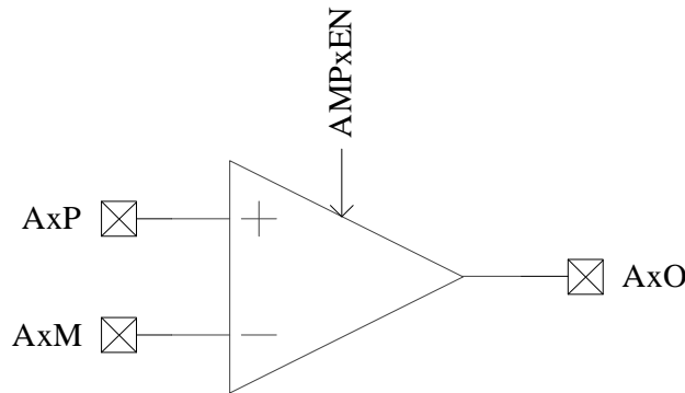
Figure 26-1 Schematic Diagram of Operational Amplifier Module
