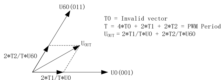
Figure 12-6 Voltage Vector Synthesis
