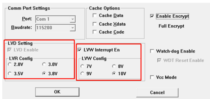
Figure 28-4 Configuration of LV Warning Threshold, LV Interrupt and LV Reset Threshold
