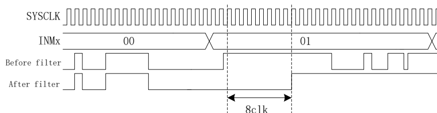
Figure13-8 Timing Diagram of Filtering Module
