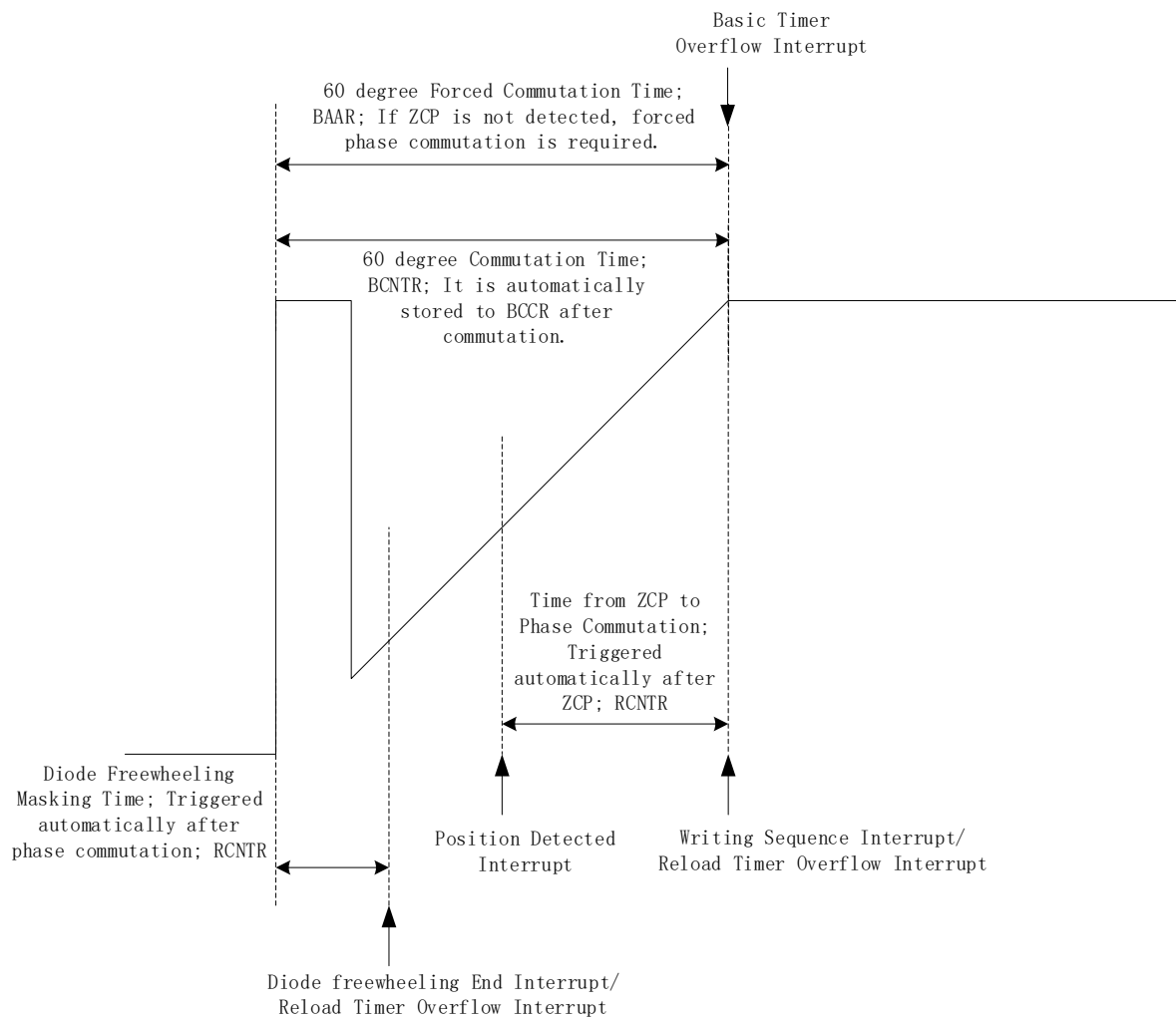
Figure13-12 Square Wave Control Working Principle
