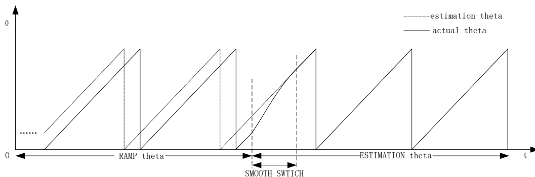
Figure 12-15 Angle Smooth Switching Waveform
