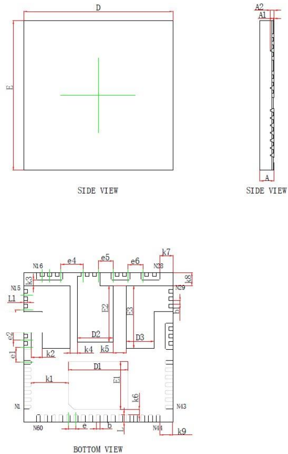
Figure 3-1 Package Dimensions of QHF8080-60L_8x8
