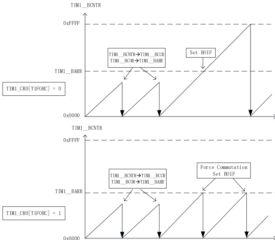
Figure13-3 Waveform of Basic Timer
