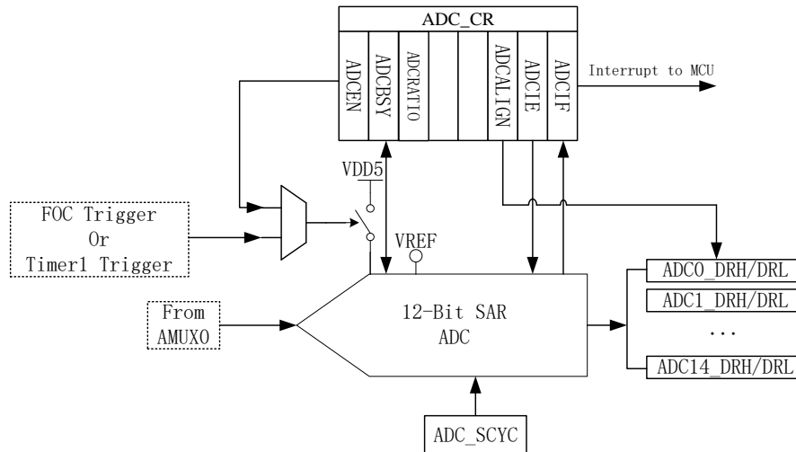
Figure21-2 ADC Functional Block Diagram
