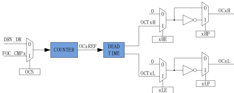
Figure 17-2 Block Diagram of Output Control Module Pre-stage
