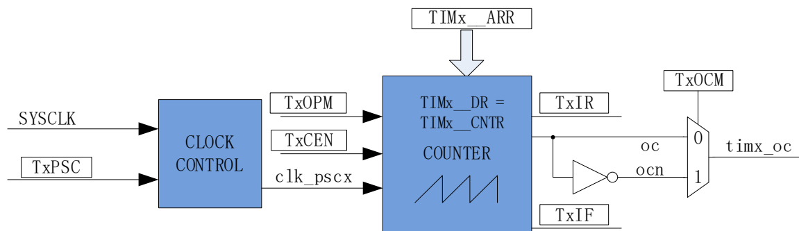
Figure15-1 Schematic Block Diagram of Output Mode
