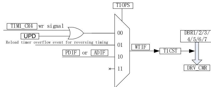
Figure13-9 Block Diagram of Write Timing
