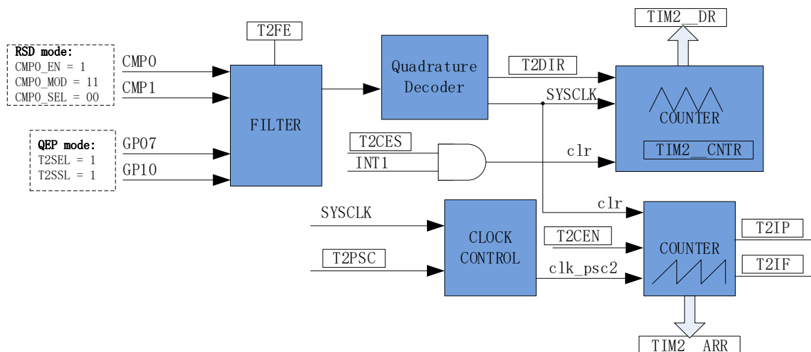
Figure14-9 Schematic Block Diagram of QEP & RSD Mode
