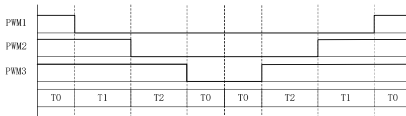
Figure 12-7 Continuous SVPWM Output Waveform
