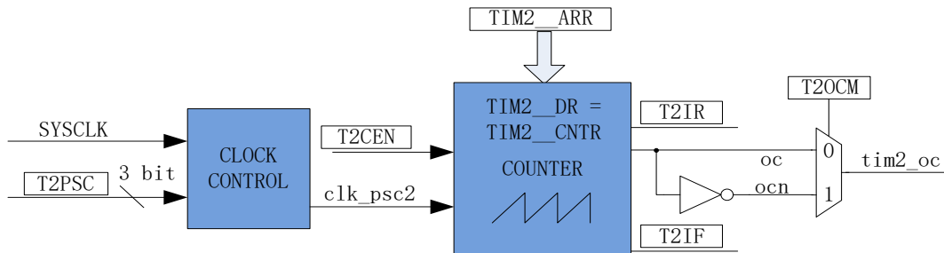
Figure14-1 Schematic Block Diagram of Output Mode
