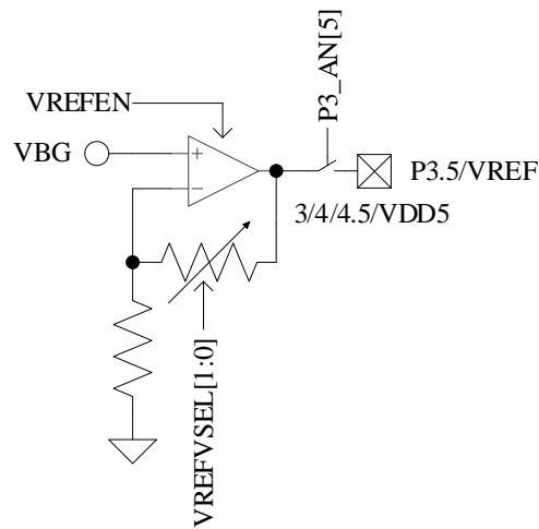
Figure 24-1 Diagram of VREF Module Input and Output
