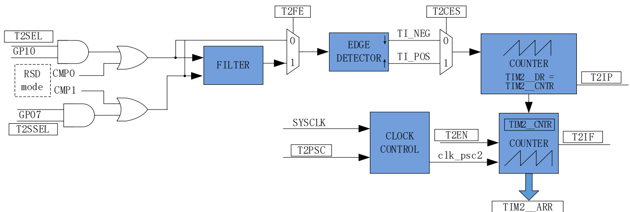
Figure14-7 Schematic Block Diagram of Input Counter Mode
