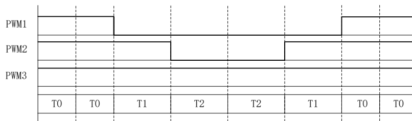
Figure 12-8 Discontinuous SVPWM Output Waveform
