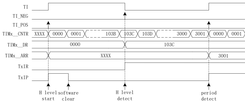
Figure 15-6 Timing Diagram of Input Capture Mode ( TIMx\_CR0[TxOCM] = 0 )
