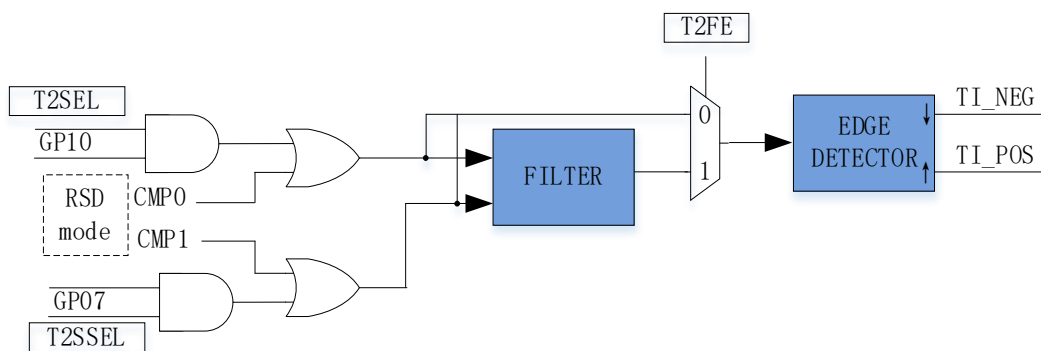
Figure14-3 Block Diagram of Input Signal Filtering and Edge Detection
