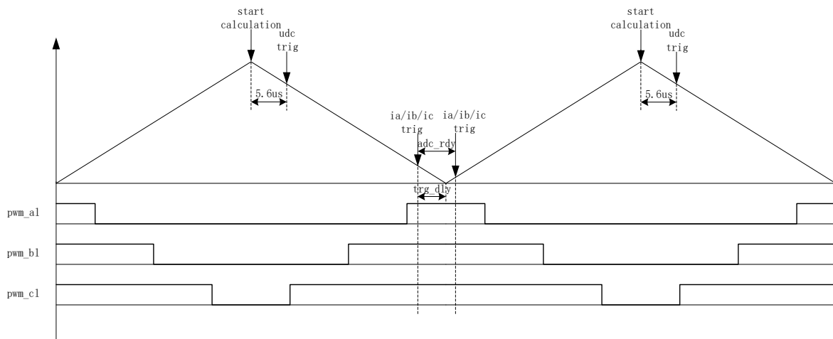
Figure 12-11 Dual/Triple-shunt Sequential Current Sampling Mode
