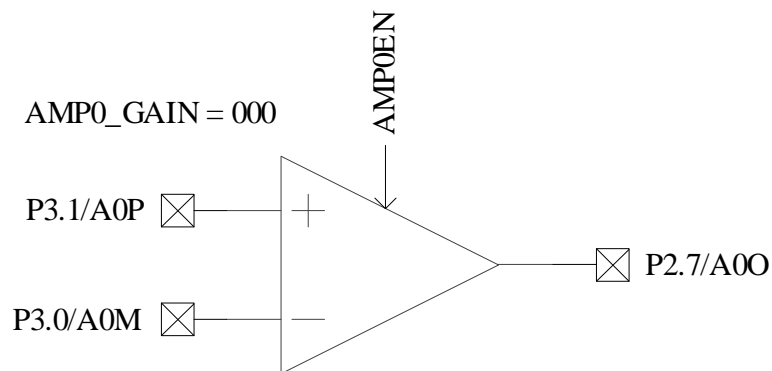
Figure 26-2 Diagram of Bus Current Operational Amplifier AMP0
