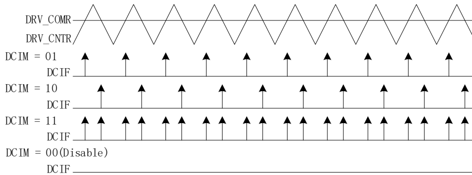
Figure 17-9 Compare Match Interrupt of Driver
