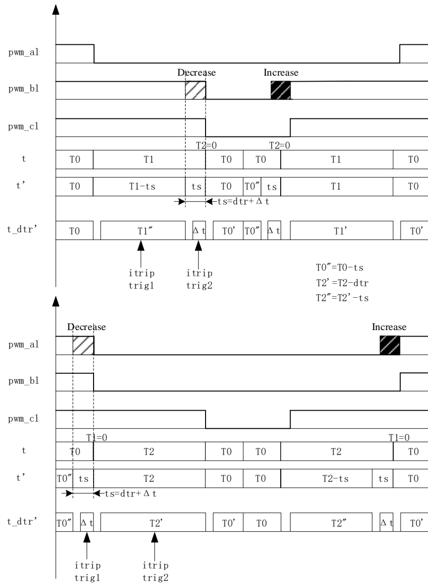
Figure 12-10 PWM Wave Shift in Single-shunt Current Sampling Mode
