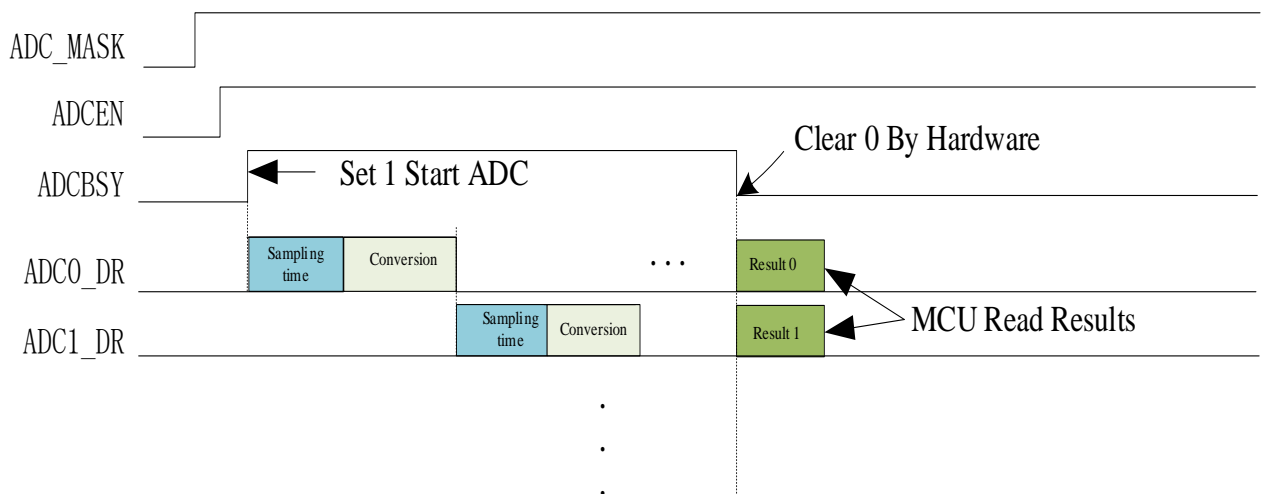
Figure21-3 Timing Diagram of ADC Sequential Sampling Mode
