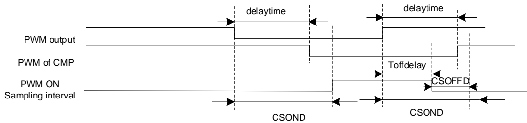
Figure 27-14 PWM OFF Sampling Mode
