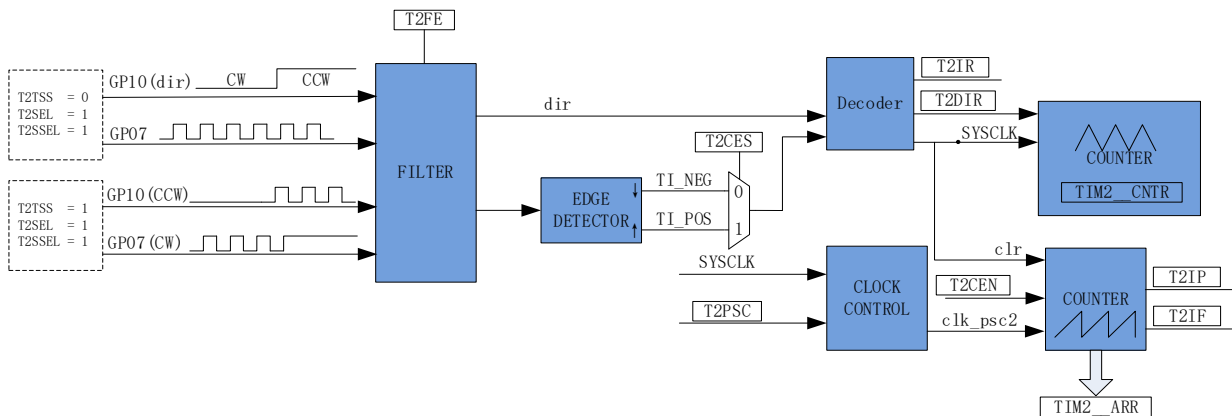
Figure14-12 Schematic Block Diagram of Step Mode
