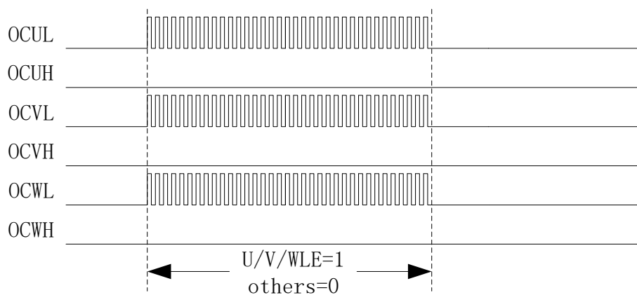
Figure 17-6 Waveform Diagram of Pre-charging
