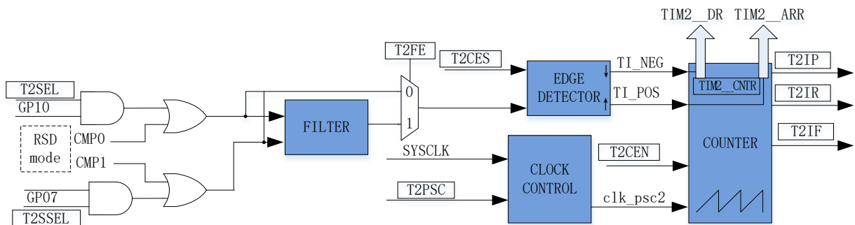
Figure14-5 Schematic Block Diagram of Input Capture Mode
