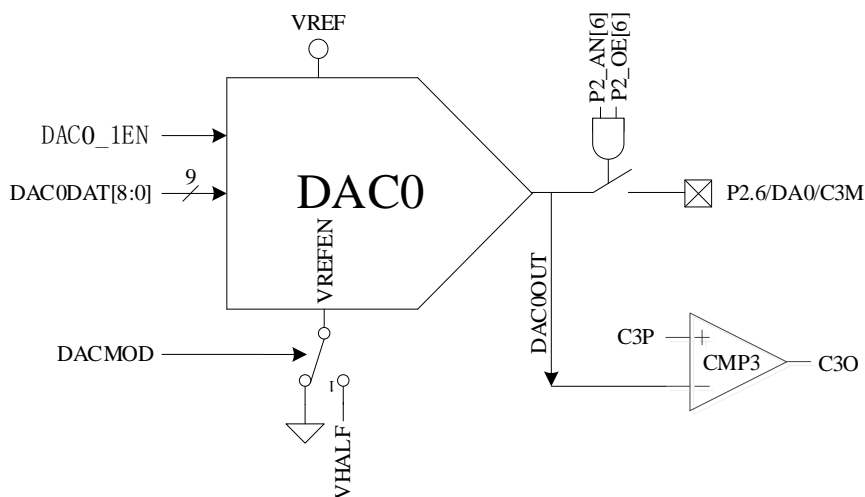
Figure 22-1 Functional Block Diagram of DAC0
