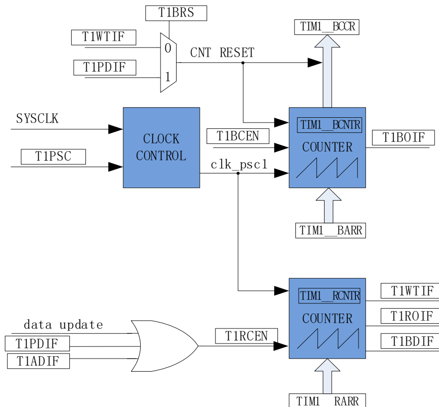
Figure13-2 Timer Counting Units
