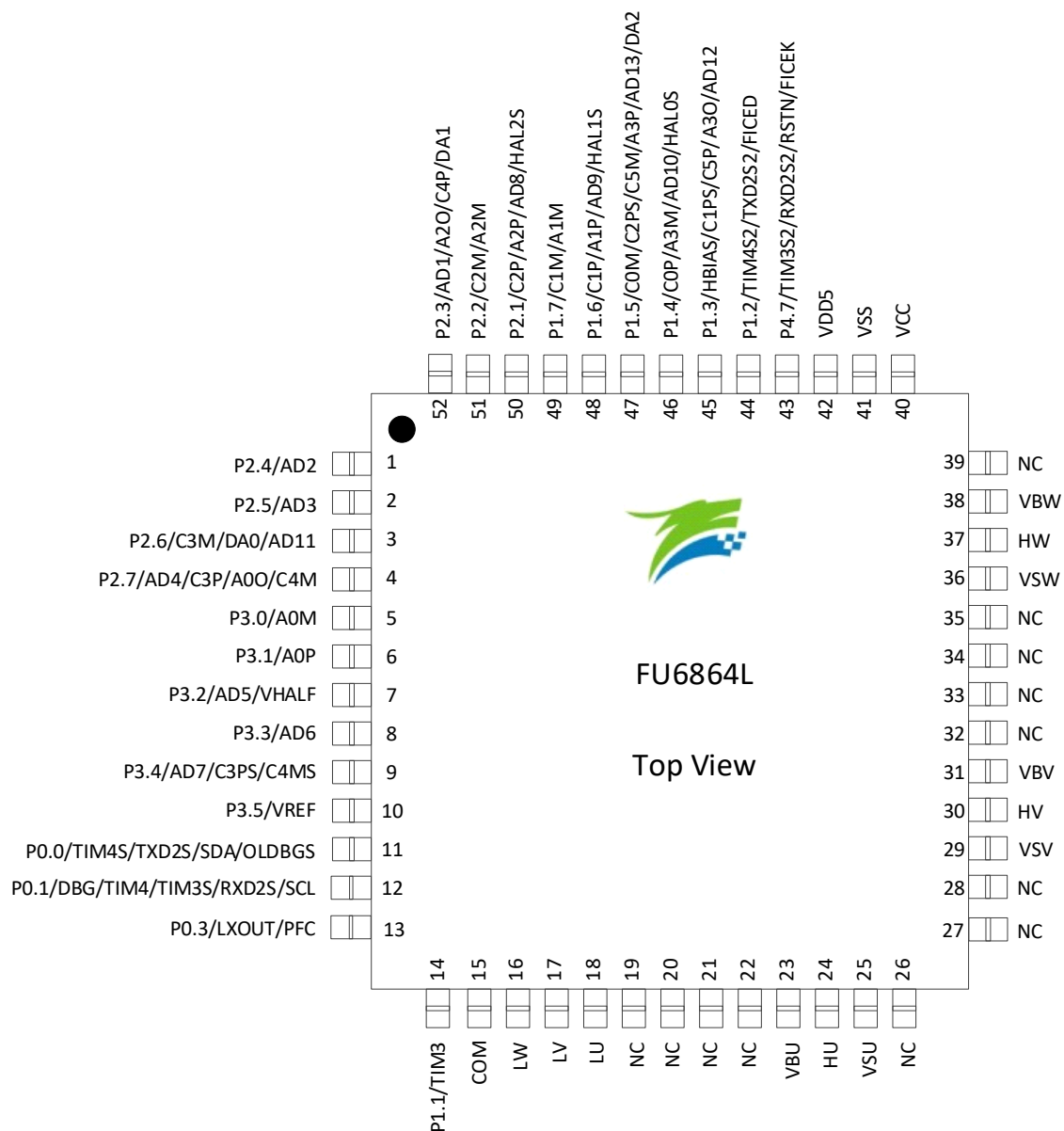
Figure 2-5 FU6864L LQFP52 Pinout Diagram
