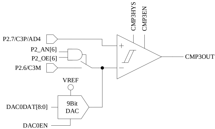
Figure 29-2 Single-comparator Input Mode
