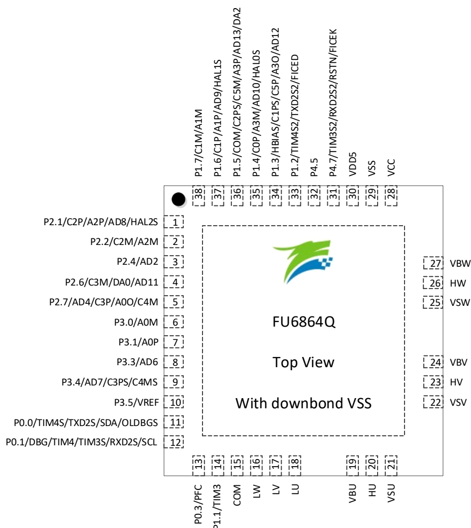
Figure 2-4 FU6864Q QFN48-38 Pinout Diagram
