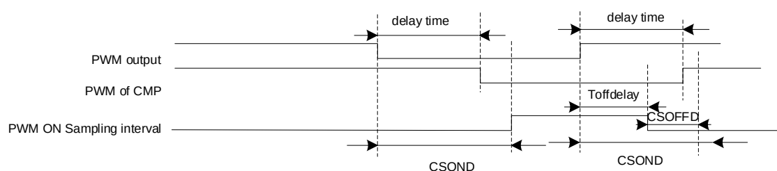
Figure 29-15 PWM OFF Sampling Mode
