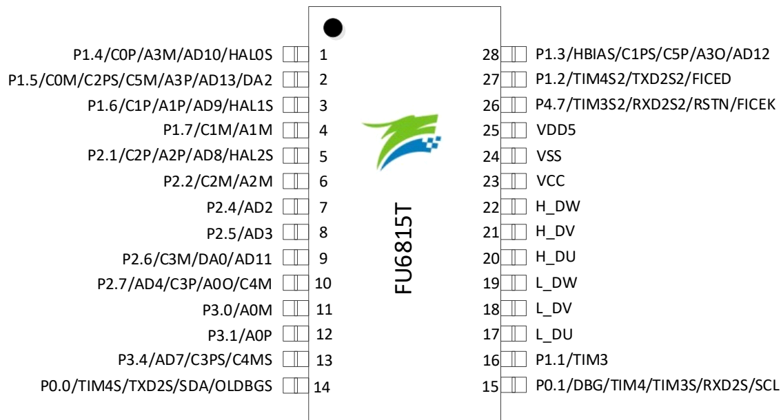
Figure 2-2 FU6815T TSSOP28 Pinout Diagram
