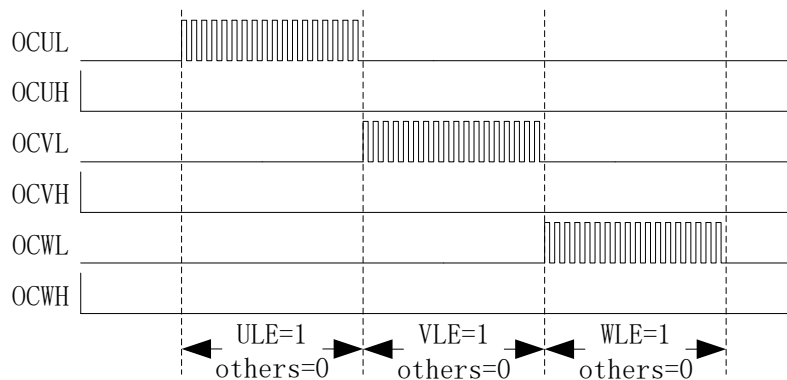
Figure 18-7 Pre-charge Waveform
