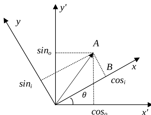
Figure 11-1 Coordinate Transformation
