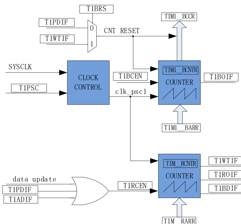
Figure 14-2 Timebase Unit
