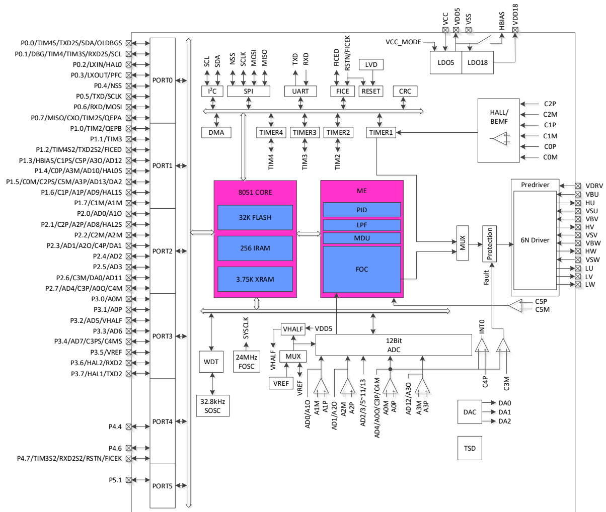
Figure 1-3 Functional Block Diagram of FU6865Q
