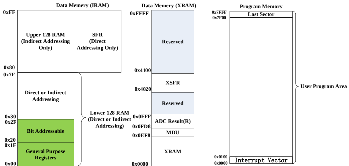
Figure 1-6 Memory Organization
