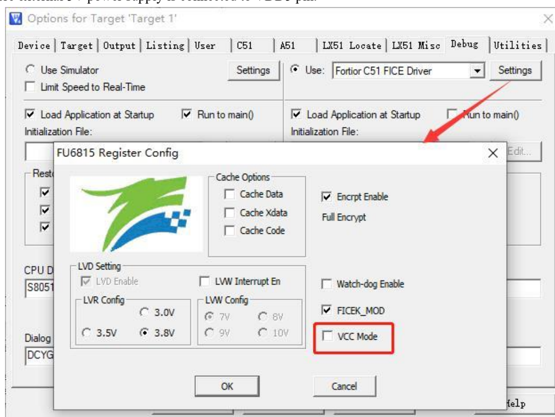
Figure 30-2 VCC_MODE Configurations
