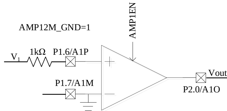
Figure 28-9 AMP1 Operating in PGA Single-ended Input Mode
