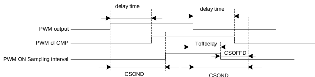
Figure 29-14 PWM ON Sampling Mode
