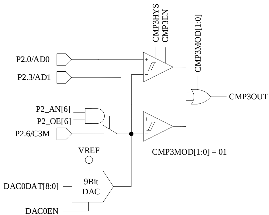
Figure 29-3 Dual-comparator Input Mode
