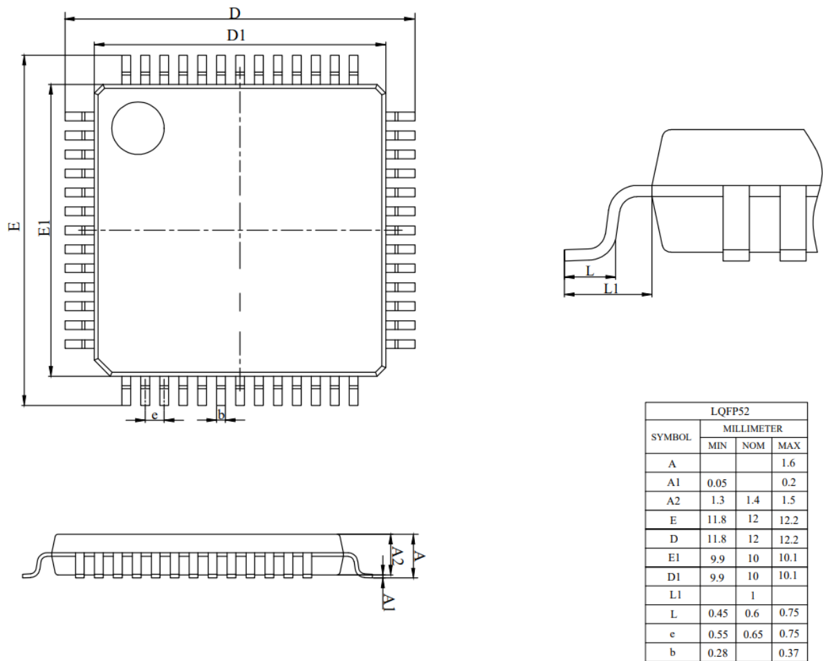
Figure 3-5 LQFP52_10X10 Package Drawings and Dimensions
