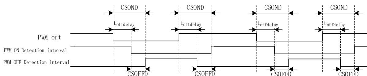
Figure 14-7 Timing Diagram of Sampling
