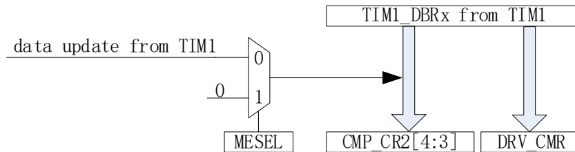
Figure 18-6 Timer1 Automatic Control of DRV_CM[R and CMP_CR2[4:3]
