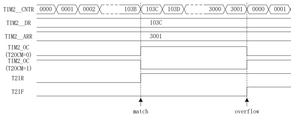
Figure 15-2 Output Mode Waveform
