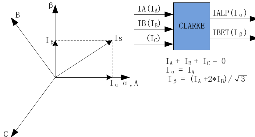
Figure 13-4 Clarke Transform
