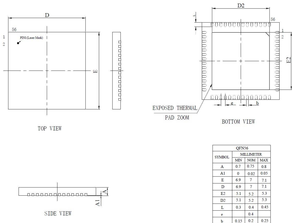
Figure 3-3 QFN56_7X7 Package Drawings and Dimensions
