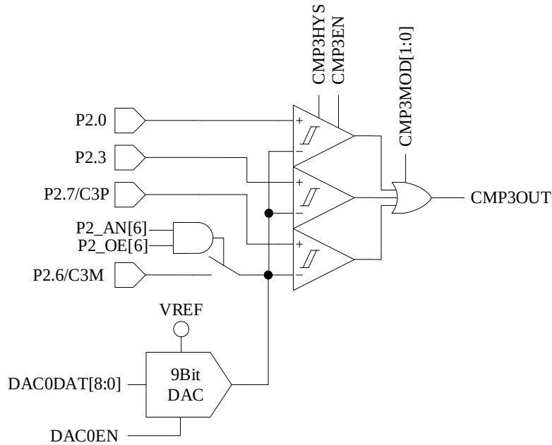
Figure 29-4 Triple-comparator Input Mode
