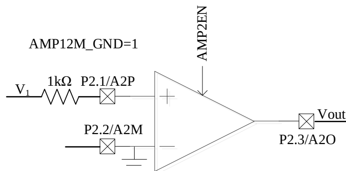
Figure 28-10 AMP2 Operating in PGA Single-ended Input Mode
