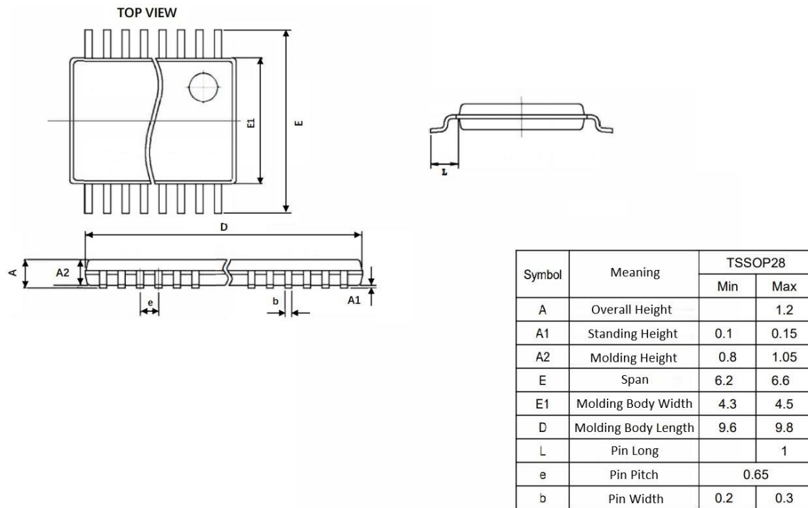
Figure 3-2 TSSOP28 9.7X4.4 Package Drawings and Dimensions
