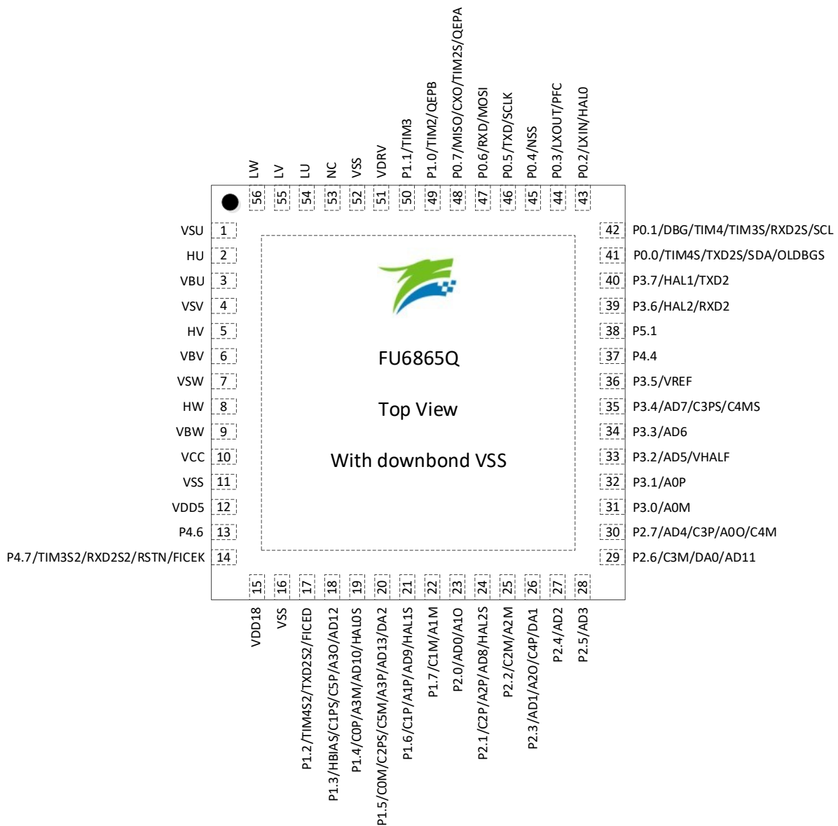
Figure 2-3 FU6865Q QFN56 Pinout Diagram
