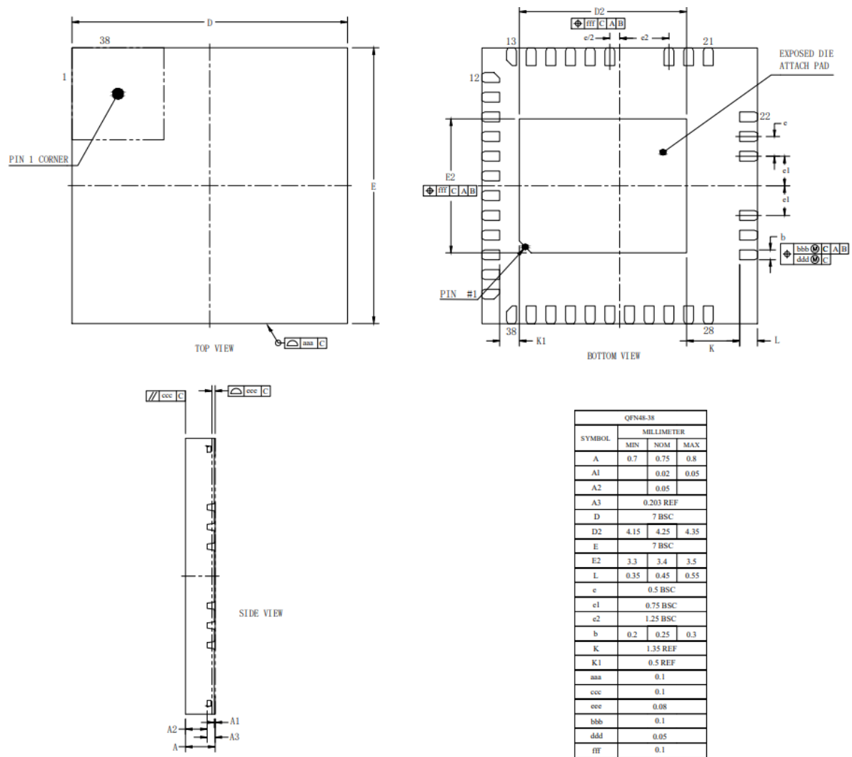
Figure 3-4 QFN48-38_7X7 Package Drawings and Dimensions
