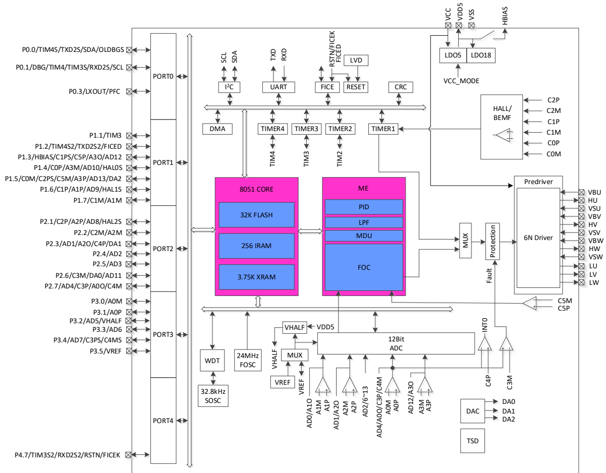
Figure 1-5 Functional Block Diagram of FU6864L
