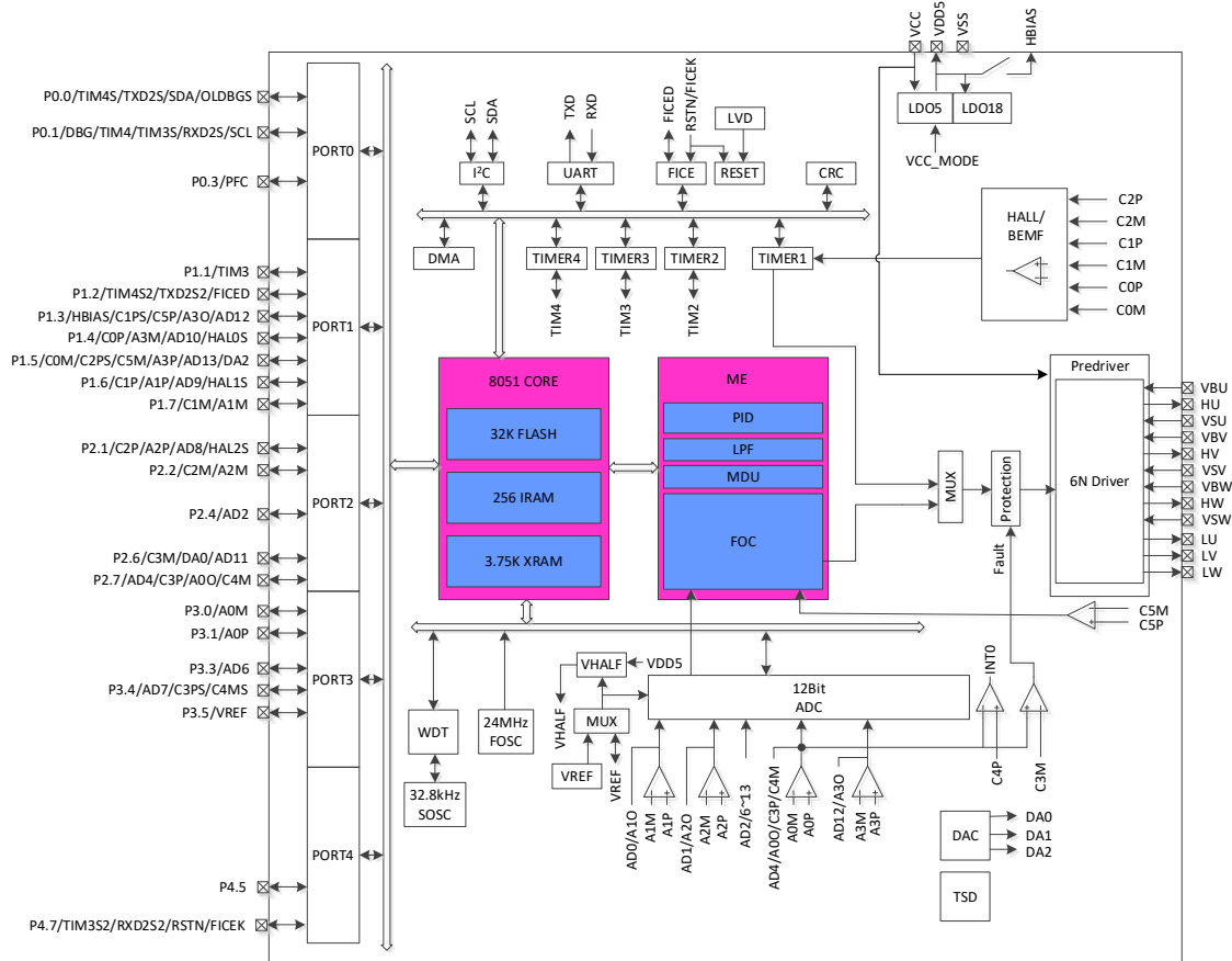
Figure 1-4 Functional Block Diagram of FU6864Q
