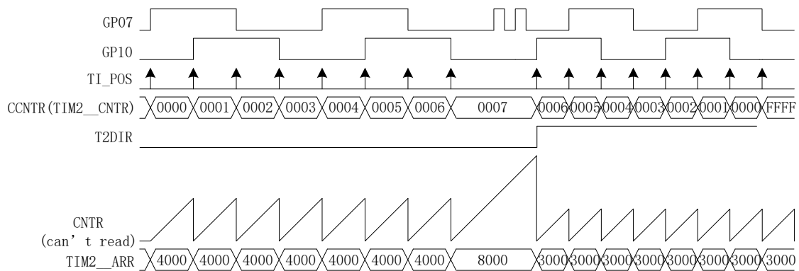
Figure 15-10 Timing Diagram of QEP&RSD Mode
