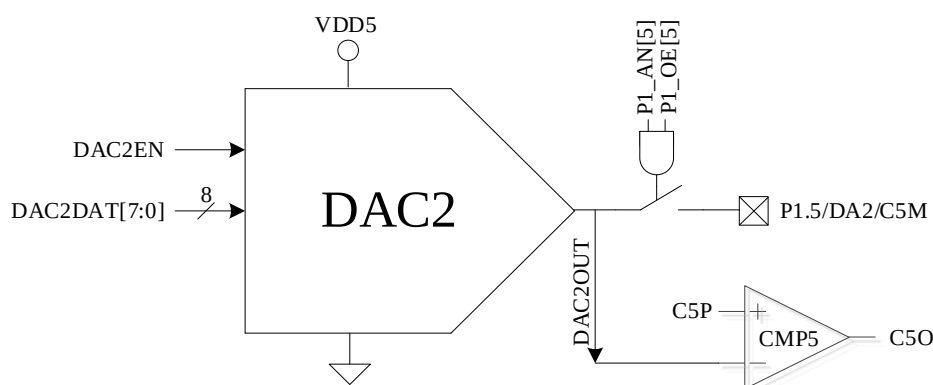
Figure 24-3 DAC2 Functional Block Diagram
