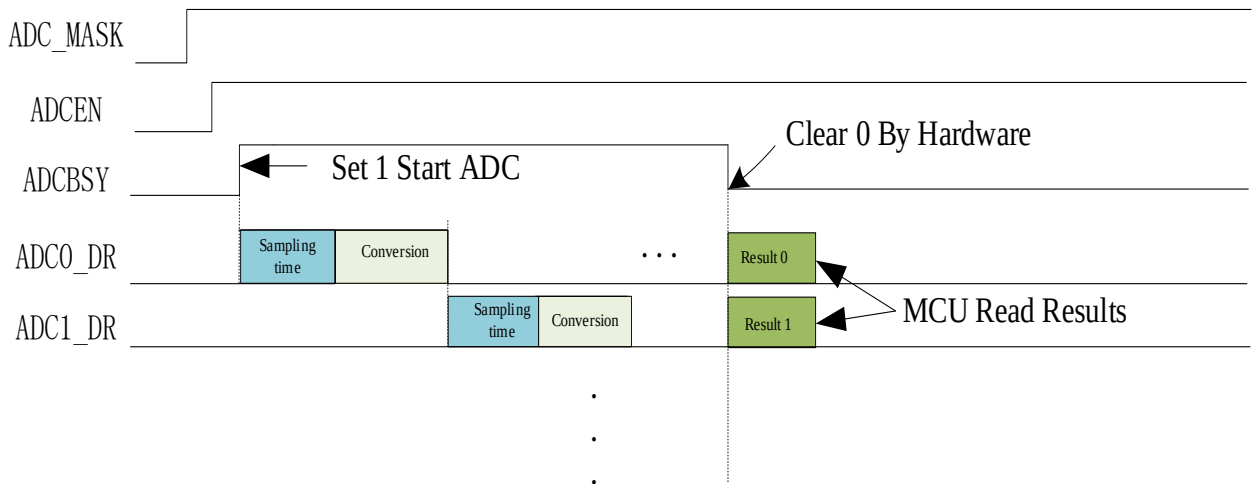
Figure 23-3 ADC Sequential Sampling Timing
