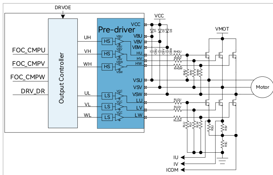
Figure 17-1 Block Diagram of FU6572 / FU6562 Driver Module
