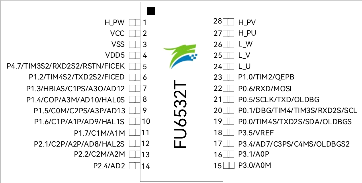
Figure 2-13 Pinout Diagram of FU6532T TSSOP28
