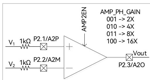
Figure 27-7 AMP2 Operating in PGA Differential Input Mode
