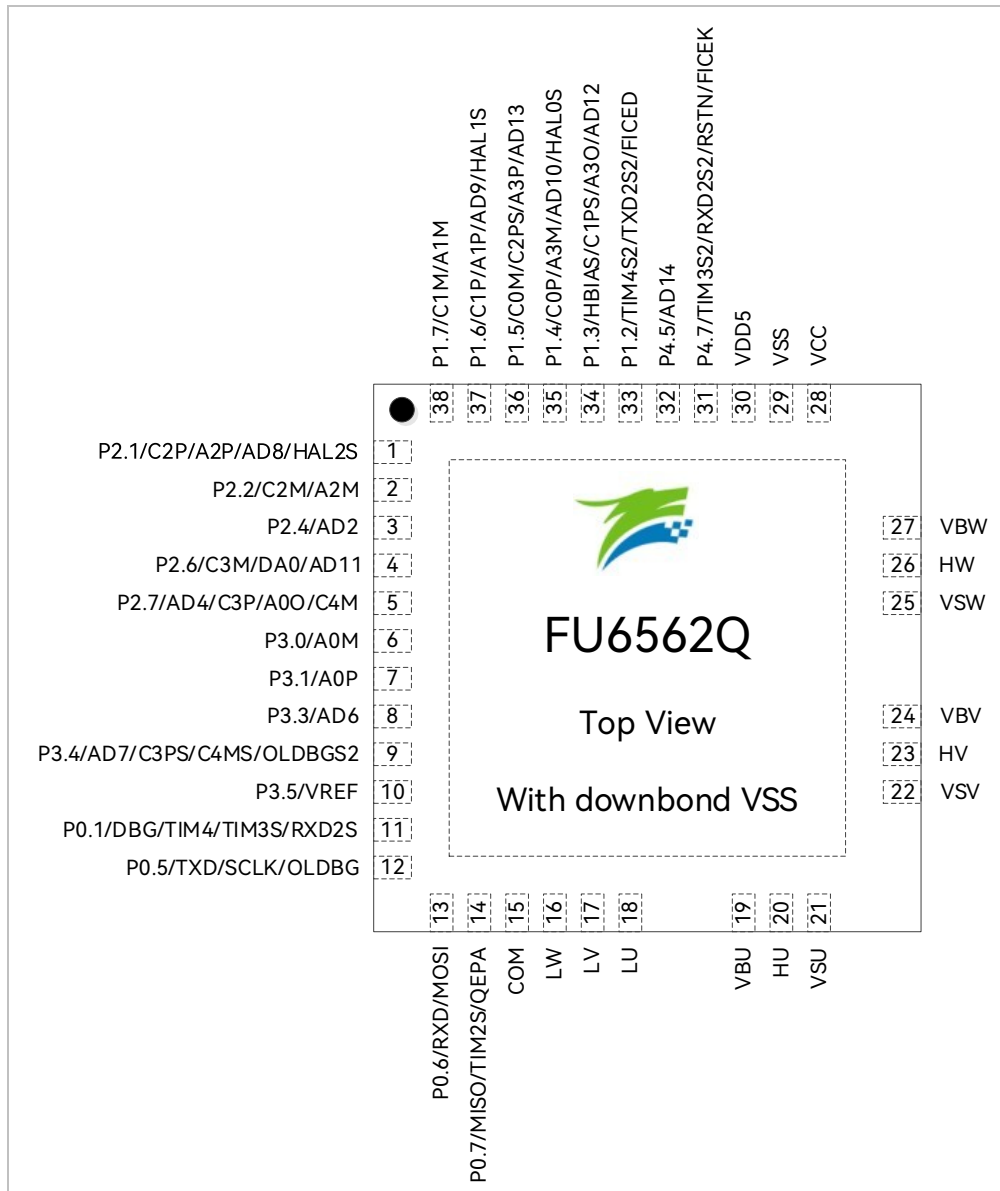
Figure 2–9 Pinout Diagram of FU6562Q QFN48–38
