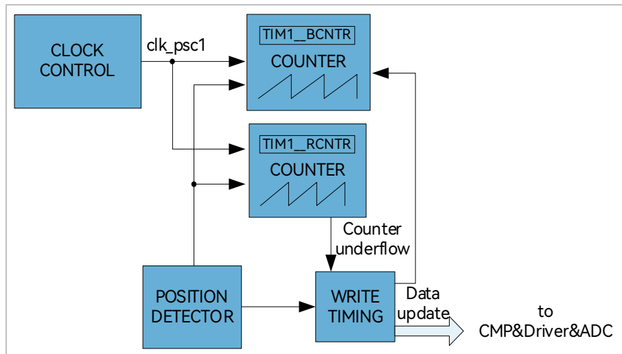
Figure 13-1 Timer1 Internal Structure
