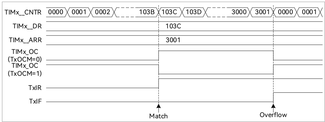
Figure 15-2 Output Waveform of Output Mode
