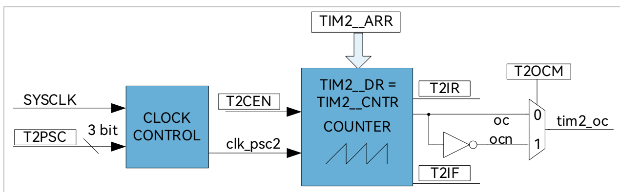
Figure 14-1 Output Mode Block Diagram
