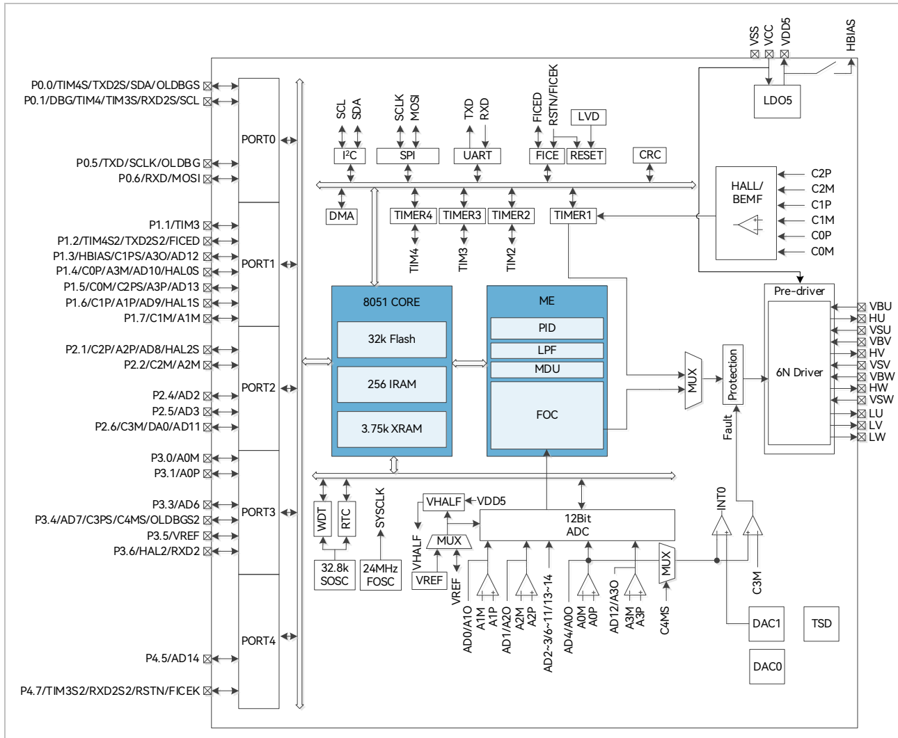
Figure 1-2 Functional Block Diagram of FU6572N
