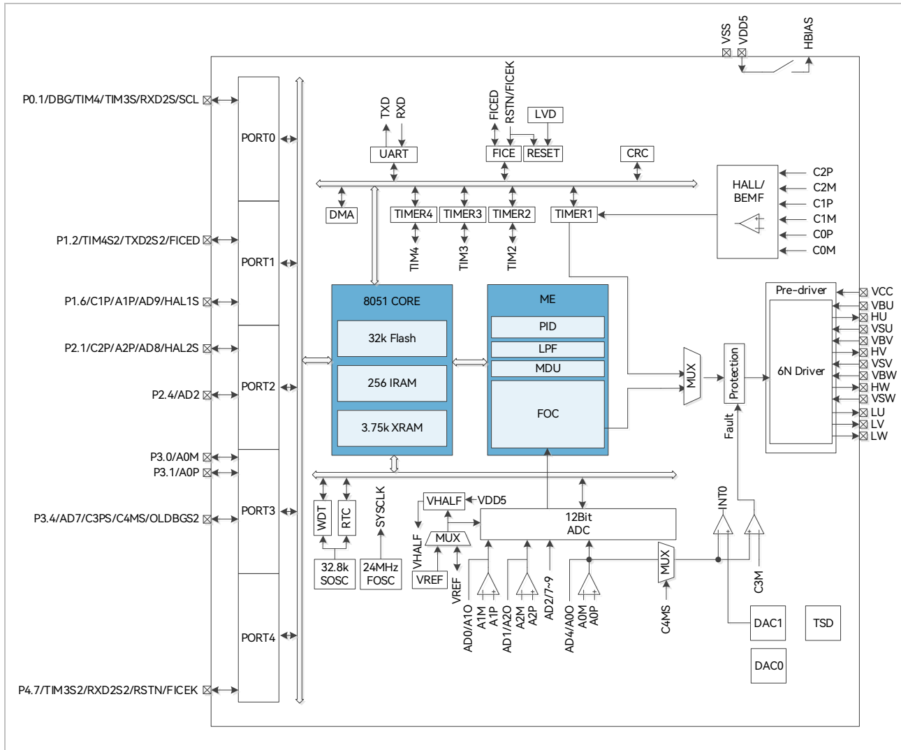
Figure 1-11 Functional Block Diagram of FU6562T
