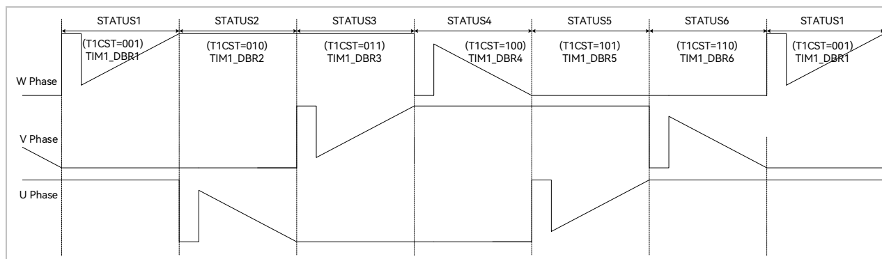
Figure 13-11 Diagram of Six-step Phase Commutation of Square Wave Control
