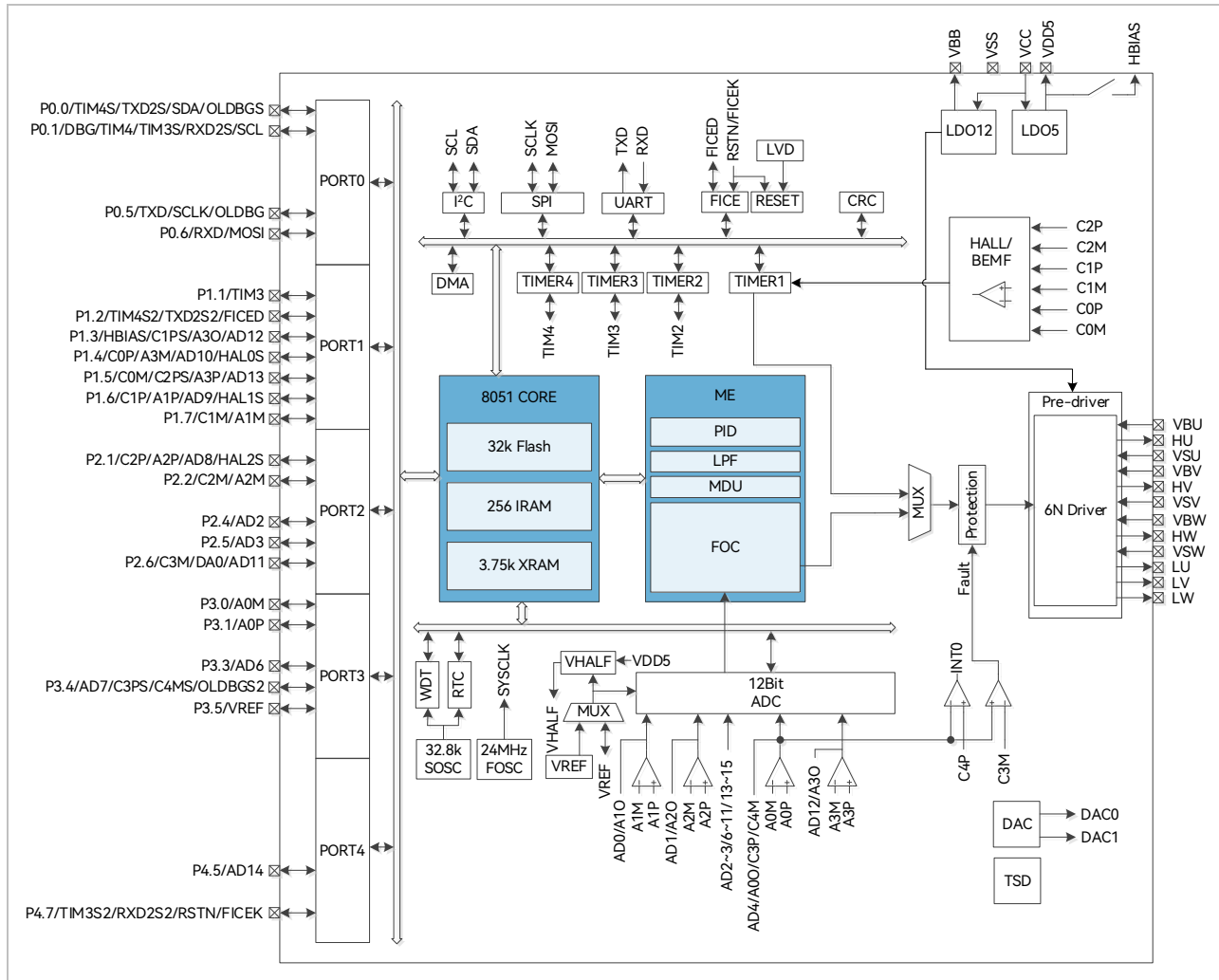
Figure 1-4 Functional Block Diagram of FU6565N
