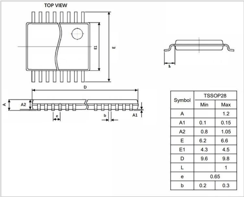
Figure 3-5 Package Drawings and Dimensions of TSSOP28_9.7x4.4
