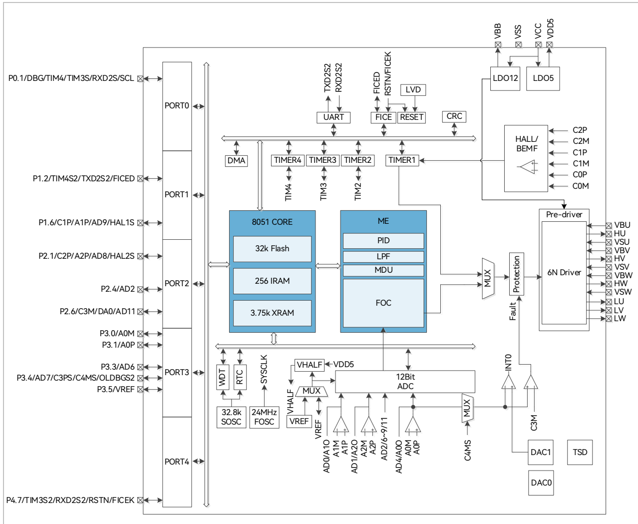
Figure 1-5 Functional Block Diagram of FU6565T
