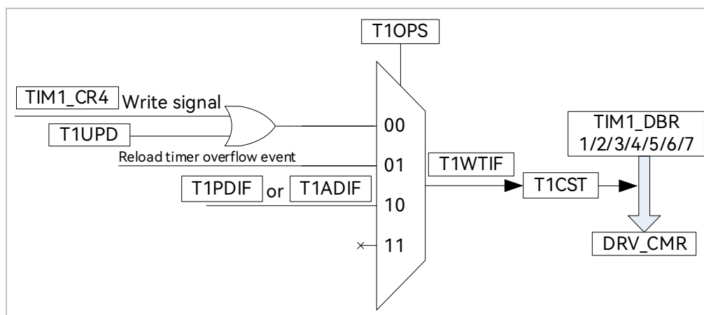
Figure 13-9 Write Timing Interrupt
