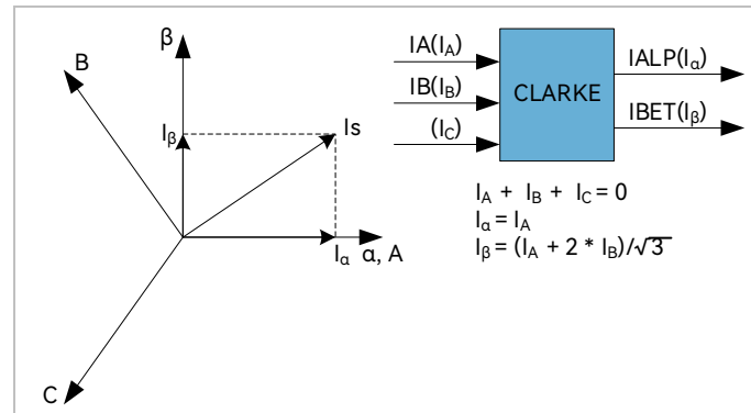
Figure 12-3 Clarke Transformation
