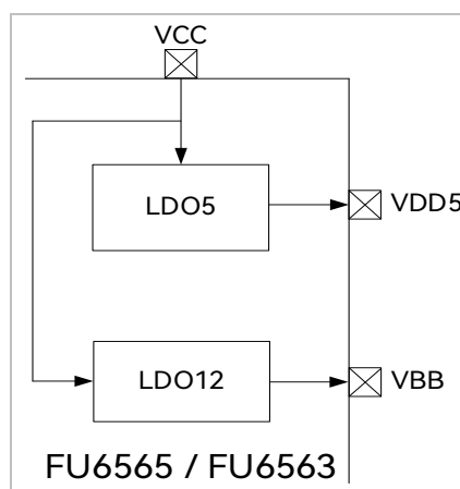
Figure 29-2 Functional Block Diagram of Power Supply
