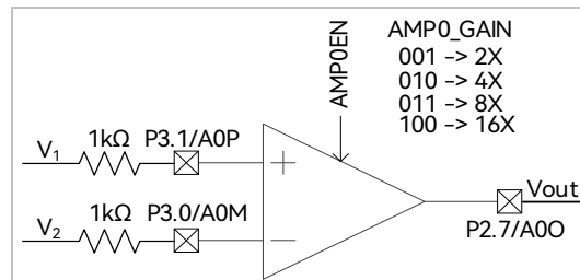
Figure 27-3 AMP0 Operating in PGA Differential Input Mode
