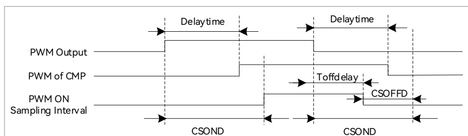
Figure 28-13 PWM ON Sampling Mode
