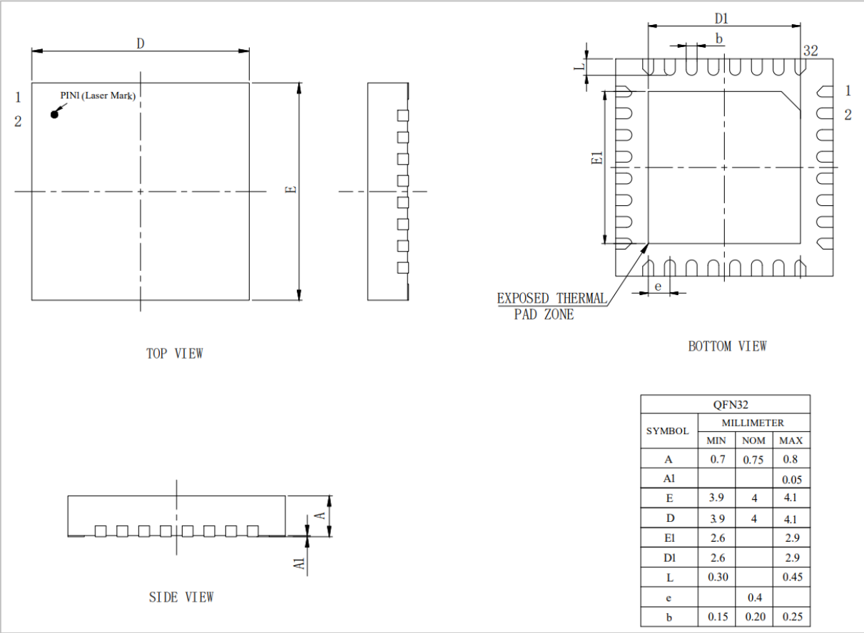
Figure 3-4 Package Drawings and Dimensions of QFN32_4X4
