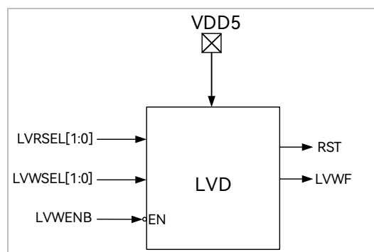
Figure 29-3 LVD Detection Module
