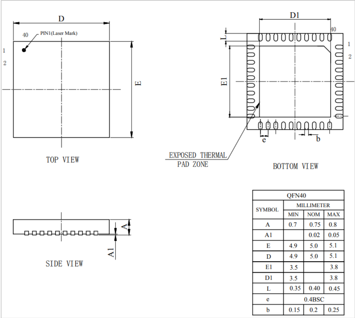
Figure 3-3 Package Drawing and Dimensions of QFN40_5X5
