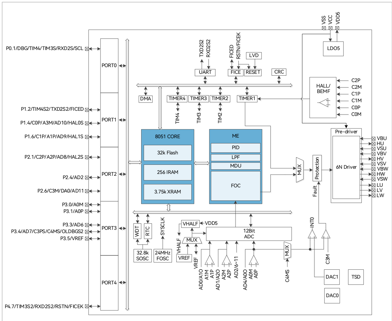
Figure 1-3 Functional Block Diagram of FU6572T
