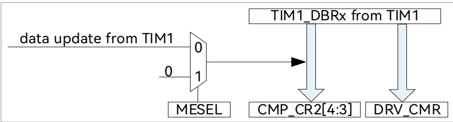
Figure 17-9 Timer1 Automatic Control of DRV_CM R and CMP_CR2[4:3]
