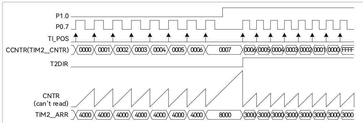
Figure 14-14 Timing Diagram of Positive + Negative Pulse Input State in Step Mode
