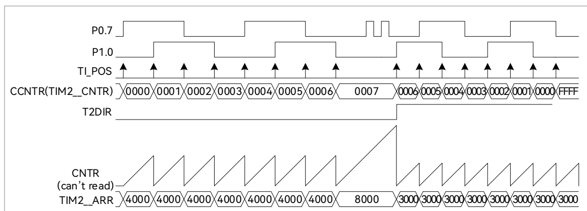
Figure 14-10 Timing Diagram of QEP&RSD Mode
