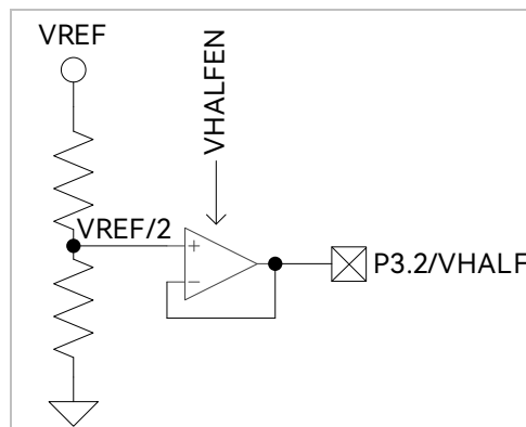
Figure 26-1 I/O Pins of VHALF Module
