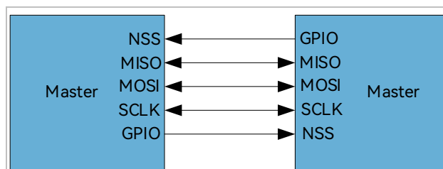
Figure 9-3 Connection Diagram of 4-Wire Single Master Mode
