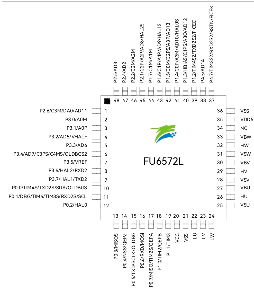
Figure 2-1 Pinout Diagram of FU6572L LQFP48
