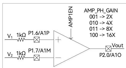
Figure 27-6 AMP1 Operating in PGA Differential Input Mode
