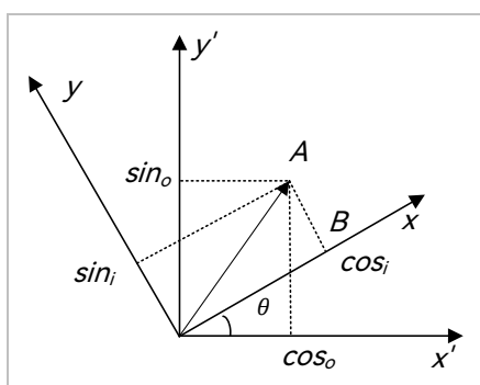
Figure 11-1 Coordinate Transformation
