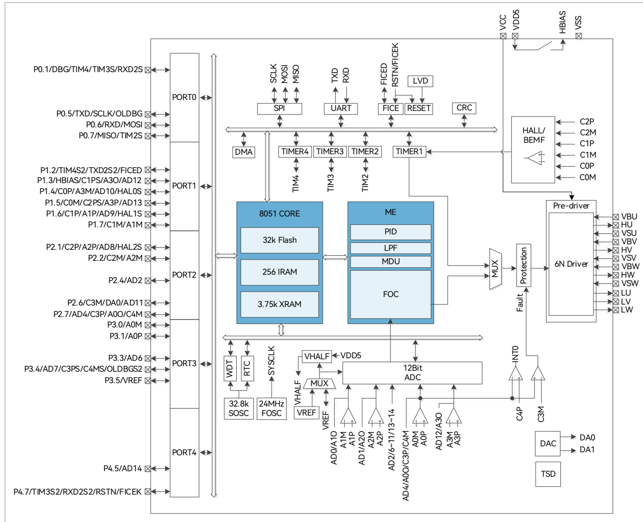
Figure 1-7 Functional Block Diagram of FU6562L
