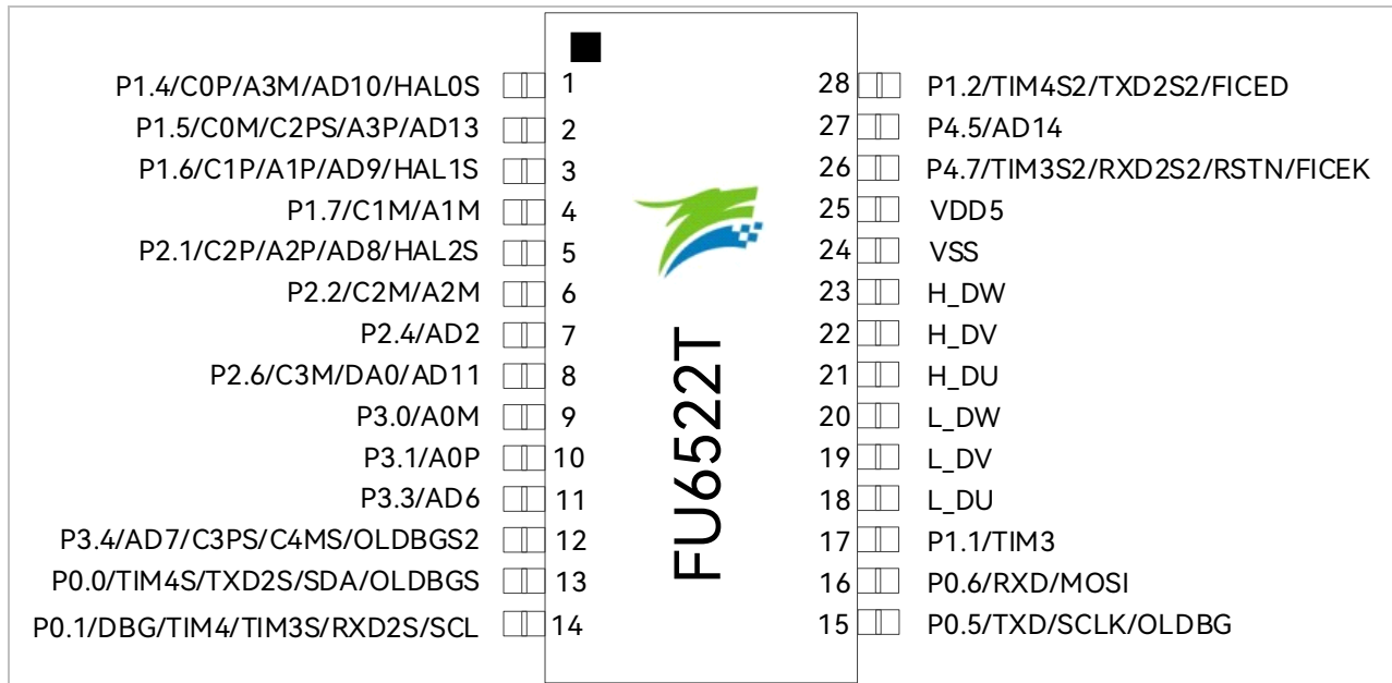
Figure 2-16 Pinout Diagram of FU6522T TSSOP28
