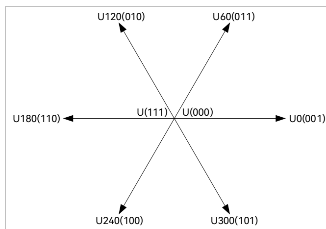
Figure 12-5 SVPWM Voltage Vector
