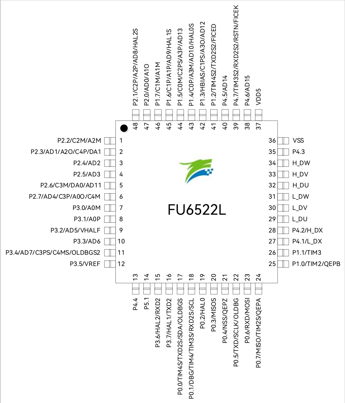
Figure 2-14 Pinout Diagram of FU6522L LQFP48
