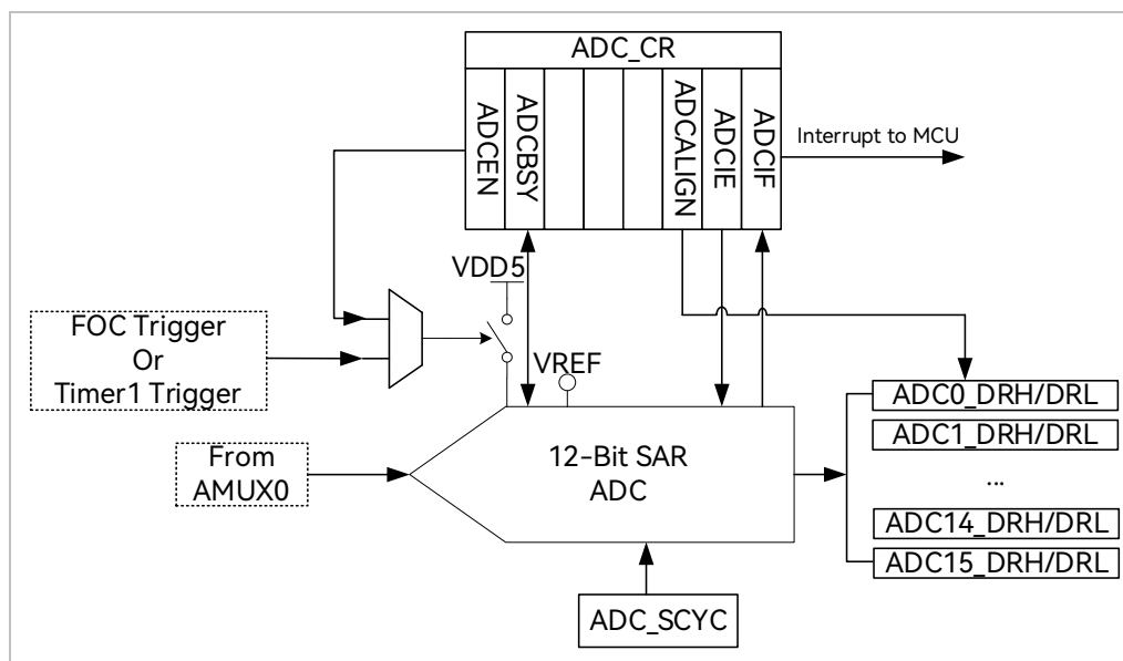
Figure 22-2 ADC Functional Block Diagram
