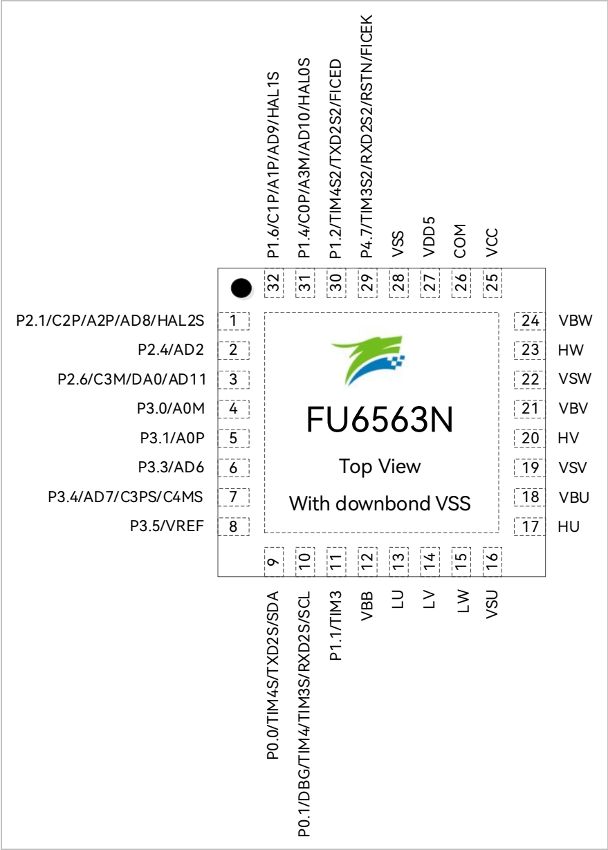
Figure 2-6 FU6563N QFN32 Pinout Diagram
