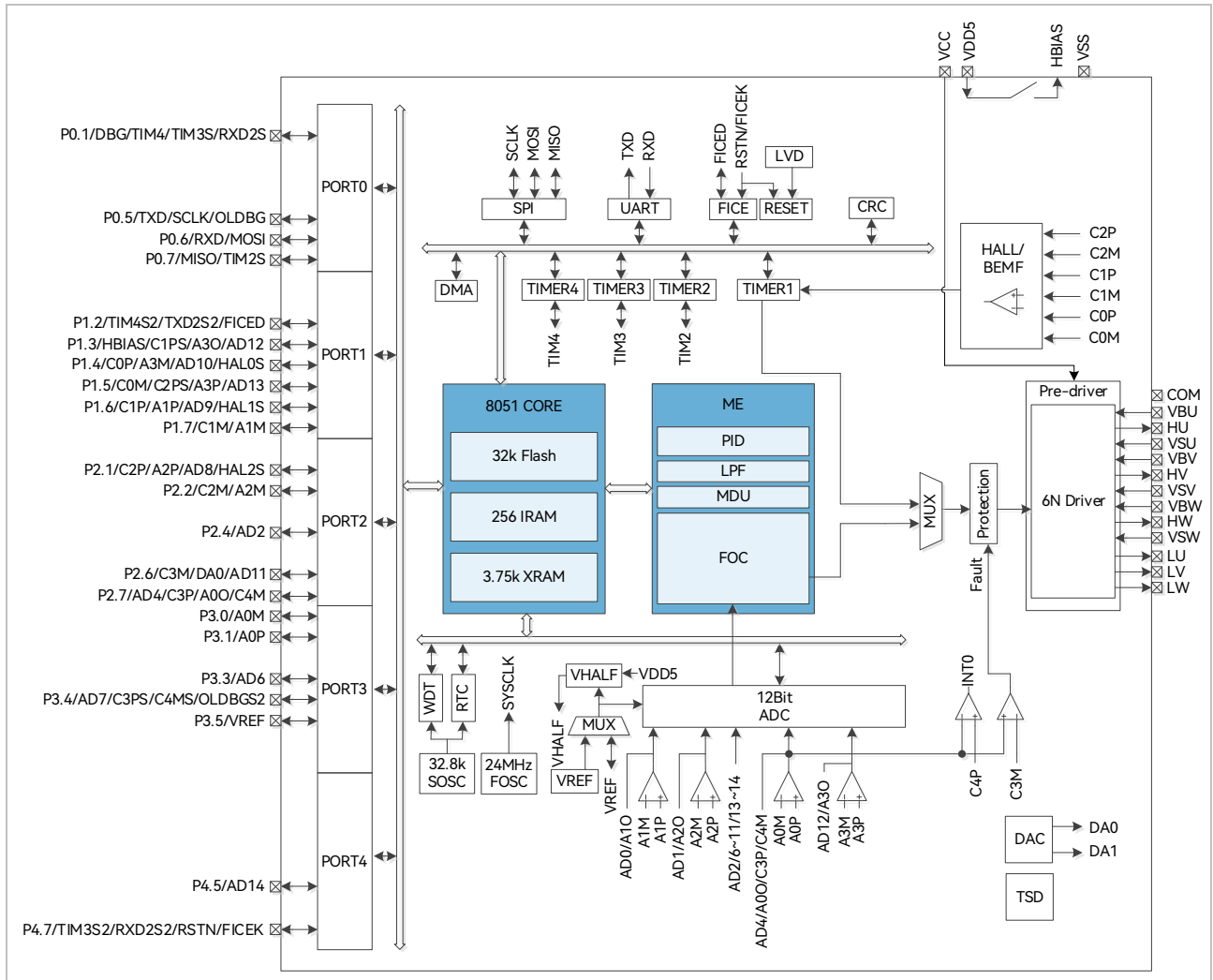
Figure 1-9 Functional Block Diagram of FU6562Q
