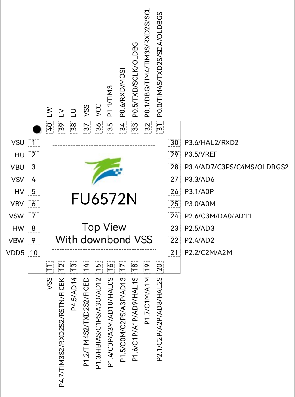
Figure 2–2 Pinout Diagram of FU6572N QFN40
