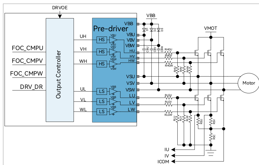
Figure 17-2 Block Diagram of FU6565 / FU6563 Driver Module
