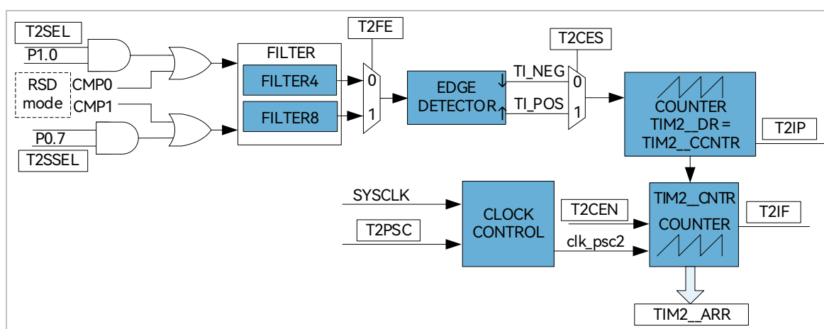
Figure 14-7 Schematic Diagram of Input Counter Mode
