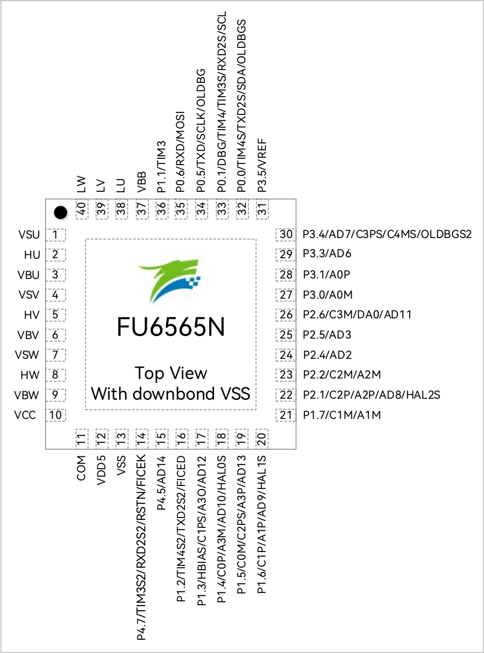
Figure 2–4 Pinout Diagram of FU6565N QFN40
