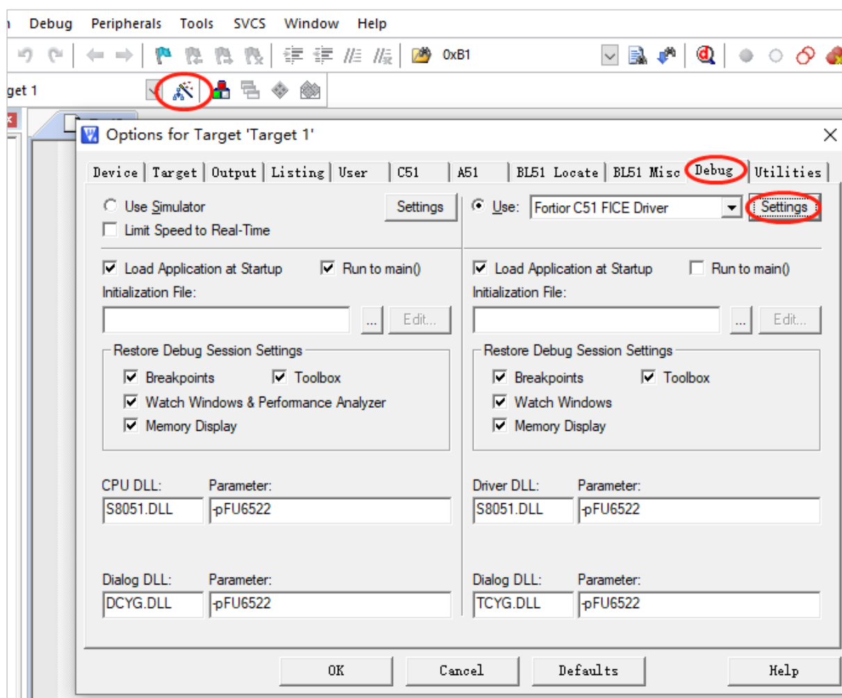
Figure 33-1 Code Protection Configurations
