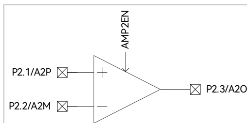
Figure 27-5 AMP2 I/O Pins
