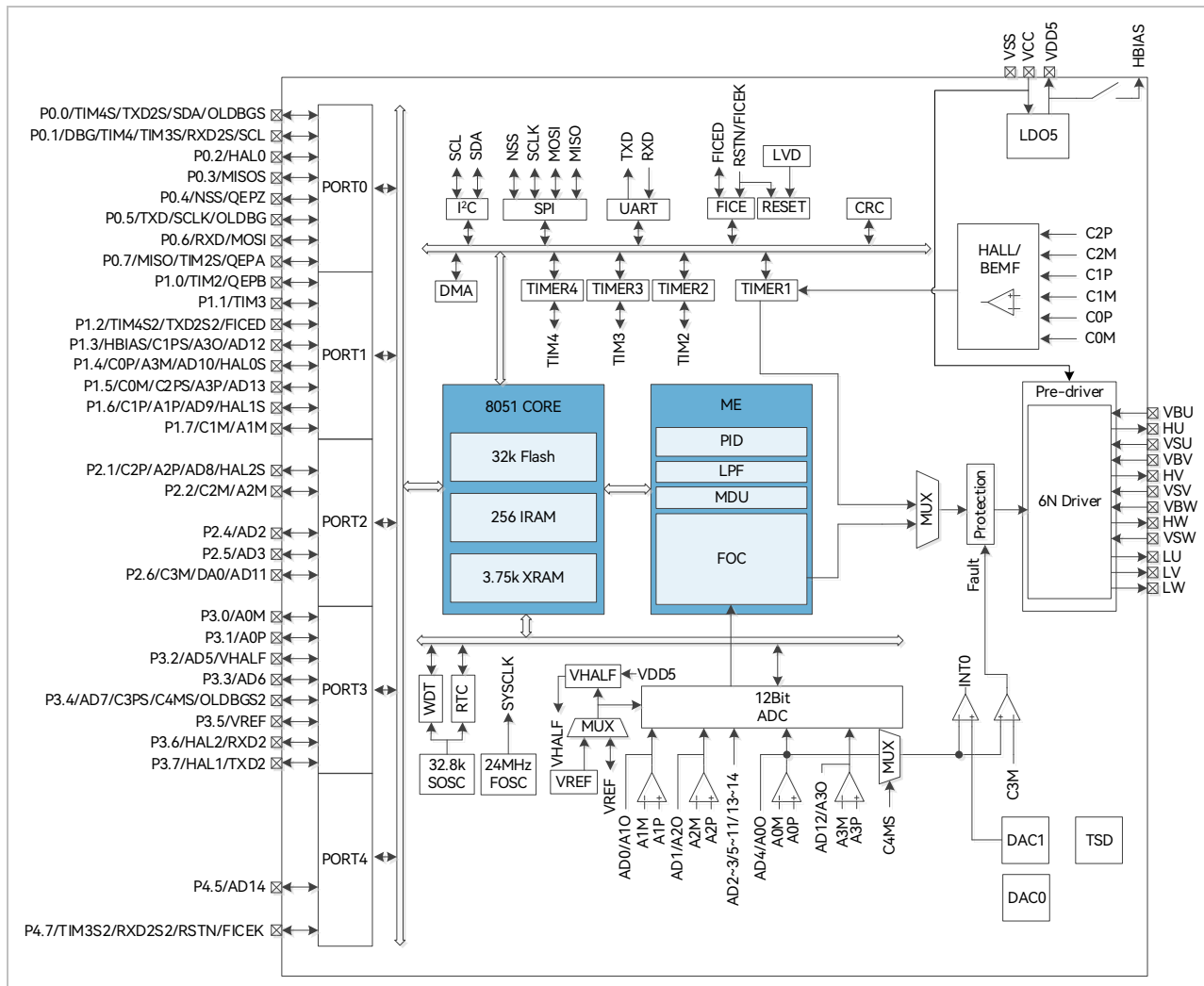
Figure 1-1 Functional Block Diagram of FU6572L
