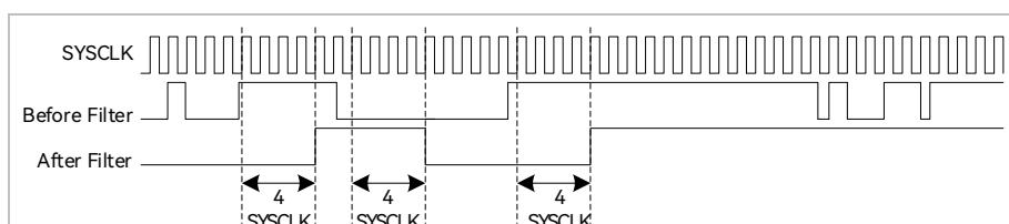
Figure 14-4 Timing Diagram of Filter Module
