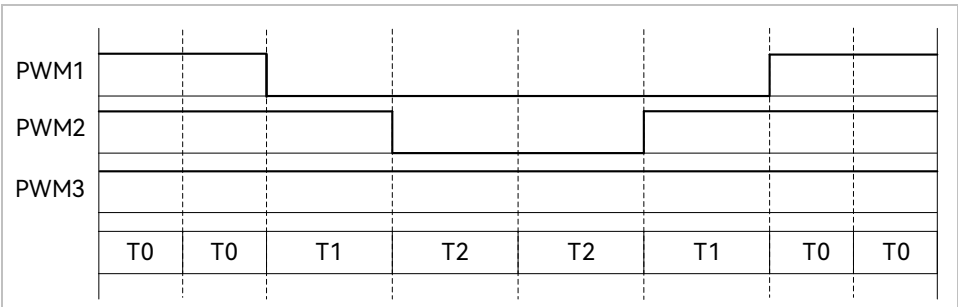
Figure 12-8 Output Level of Discontinuous SVPWM
