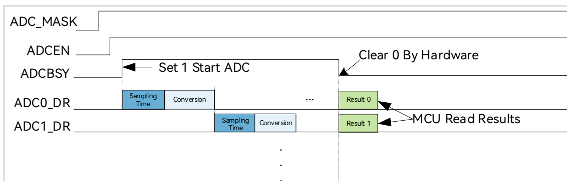
Figure 22-3 ADC Sequential Sampling Mode
