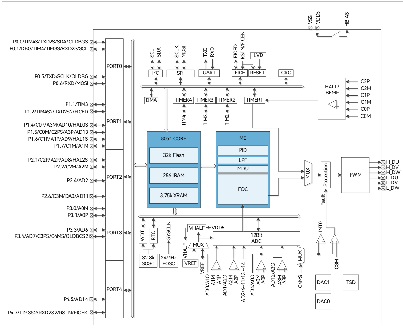
Figure 1-16 Functional Block Diagram of FU6522T
