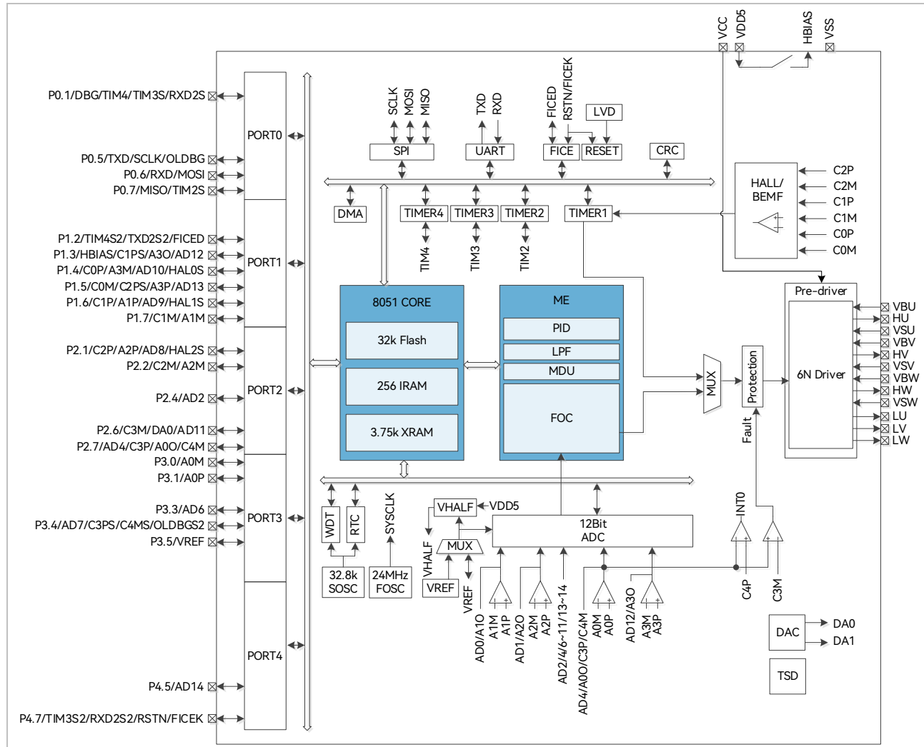
Figure 1-8 Functional Block Diagram of FU6562LA
