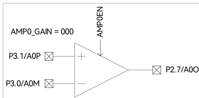
Figure 27-2 Bus Current AMP0
