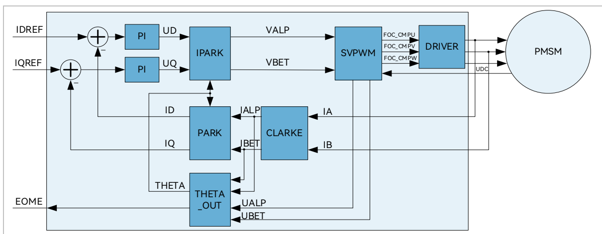
Figure 12-1 FOC Block Diagram
