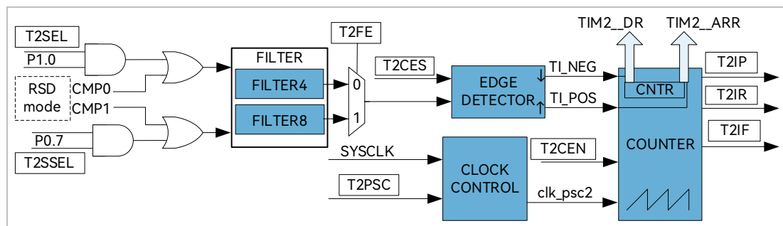
Figure 14-5 Schematic Diagram of Input Capture Mode
