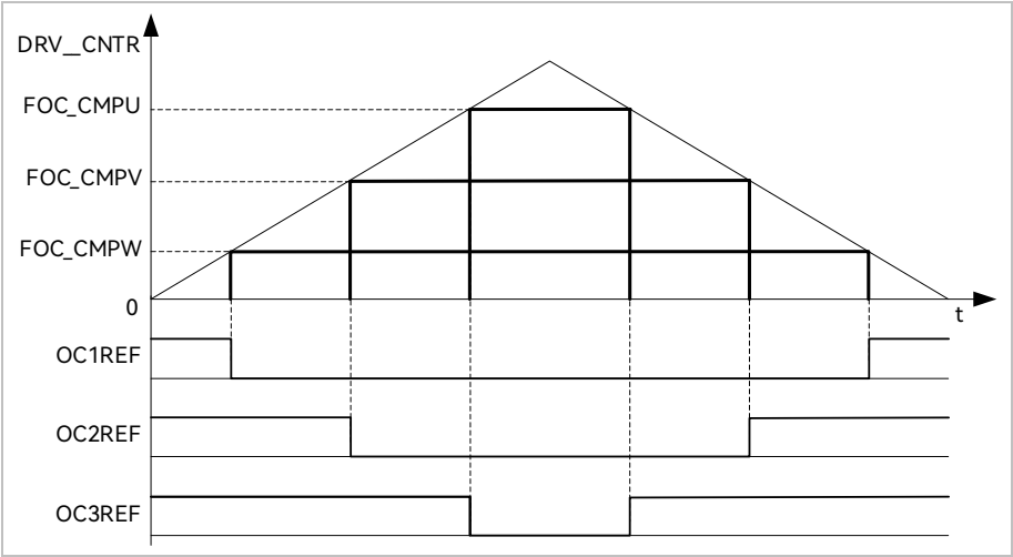
Figure 17-6 PWM Generation
