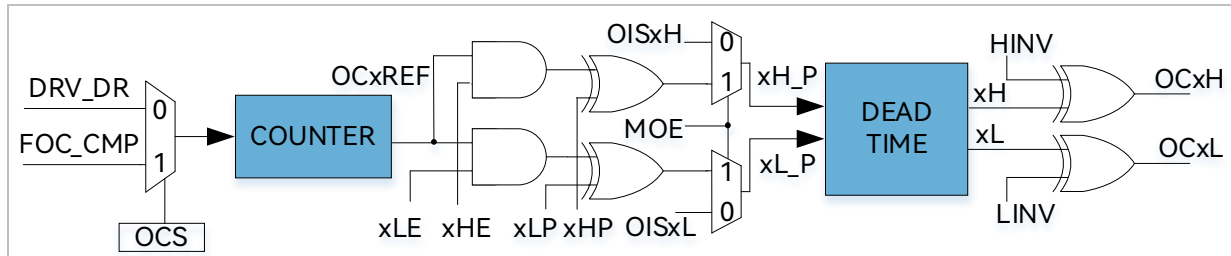
Figure 17-5 Block Diagram of Output Control Module
