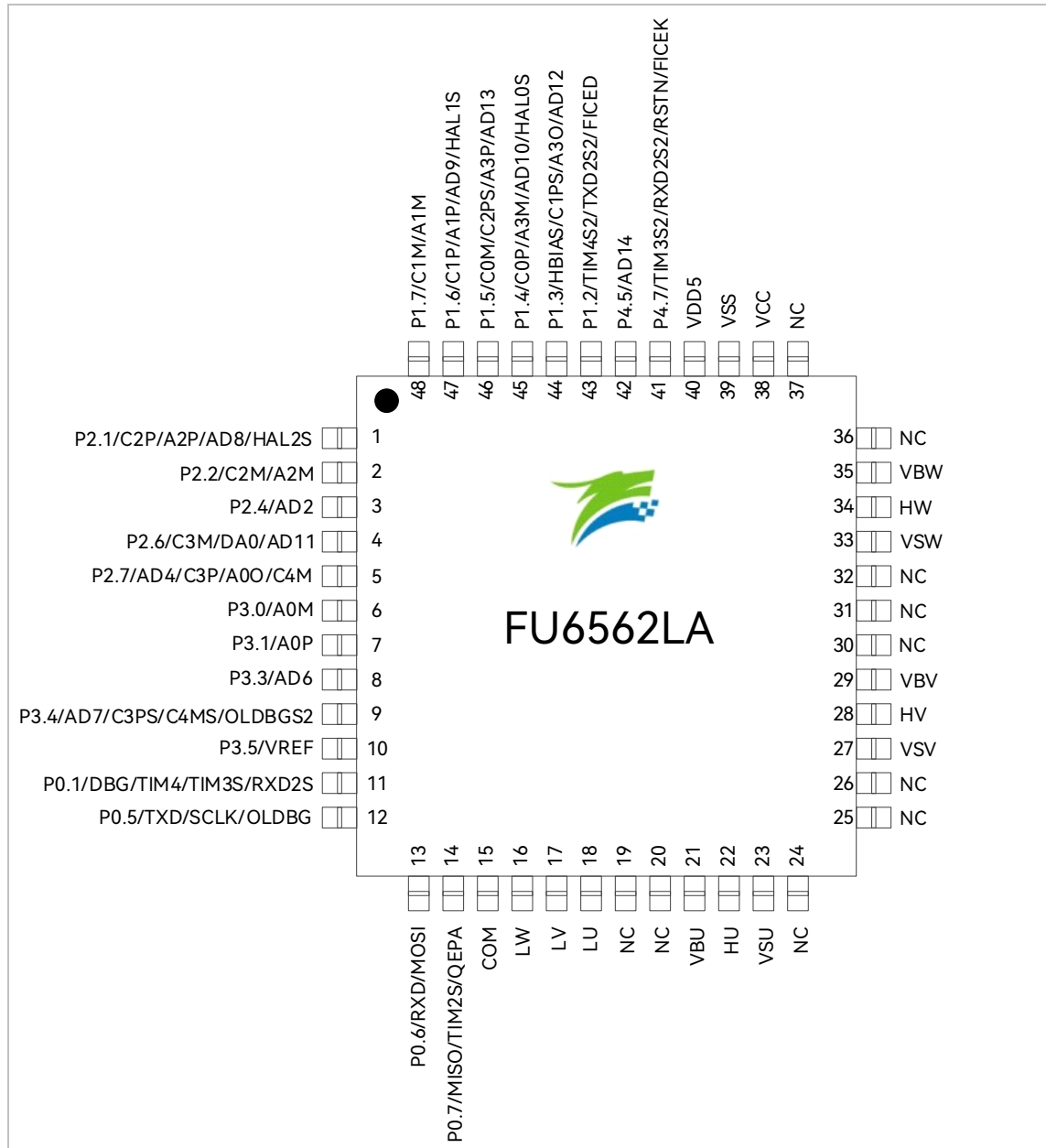
Figure 2–8 Pinout Diagram of FU6562LA LQFP48
