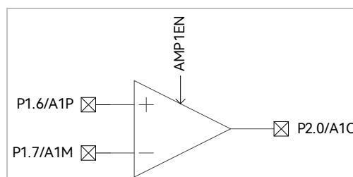
Figure 27-4 AMP1 I/O Pins
