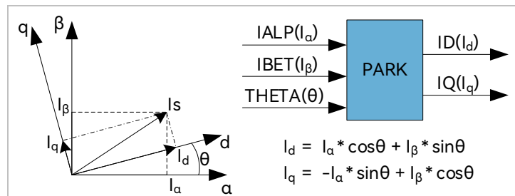
Figure 12-4 Park Transformation
