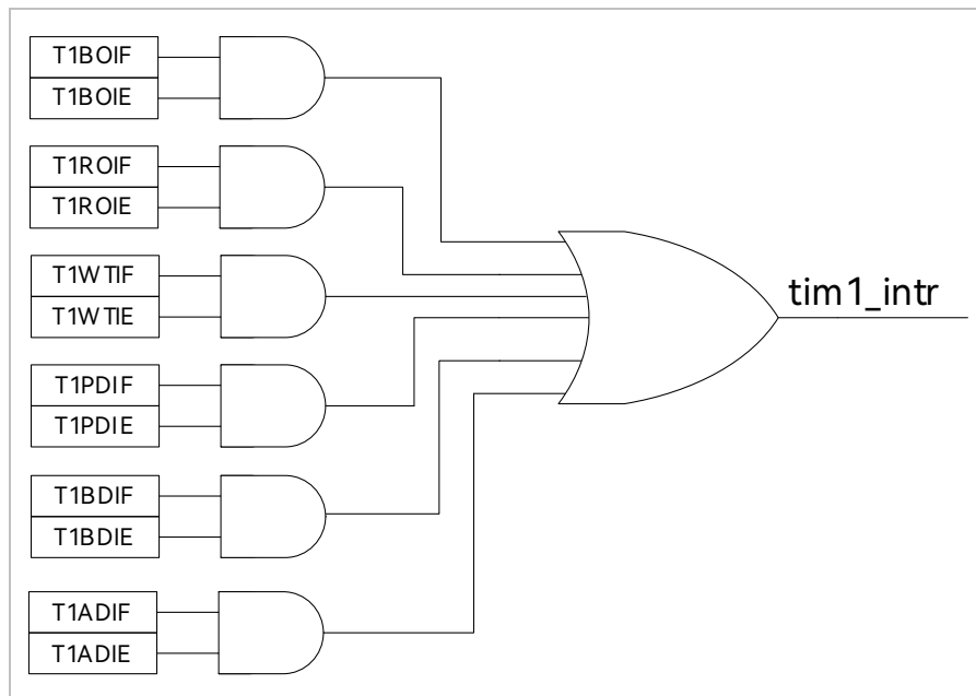
Figure 13-10 Timer1 Interrupt Sources
