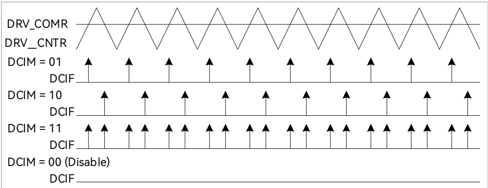
Figure 17-12 Driver Compare Match Interrupt
