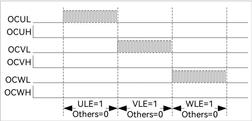
Figure 17-7 Pre-charge Waveform
