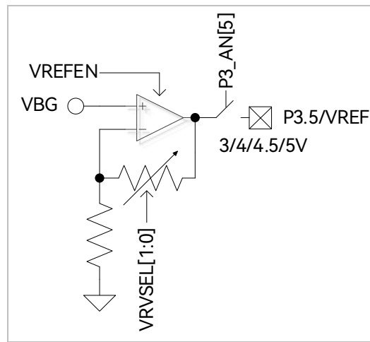
Figure 25-1 I/O Pins of VREF Module
