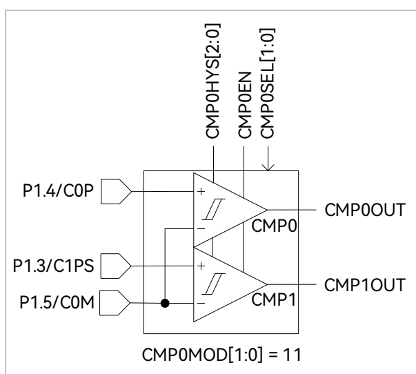
Figure 28-12 CMPG Mode with Dual-comparators
