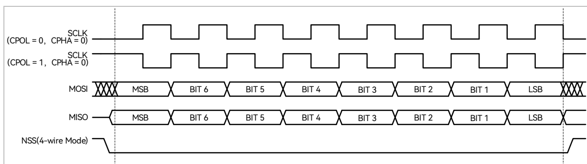
Figure 9-5 SDA/SCL Line Timing Diagram (SPI_CR0[CPHA] = 0)
