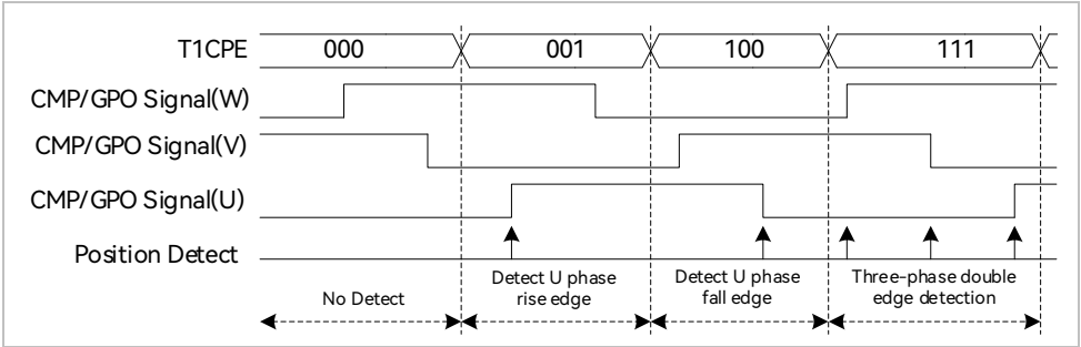
Figure 13-6 Timing Diagram of CMP/GPIO Position Detection
