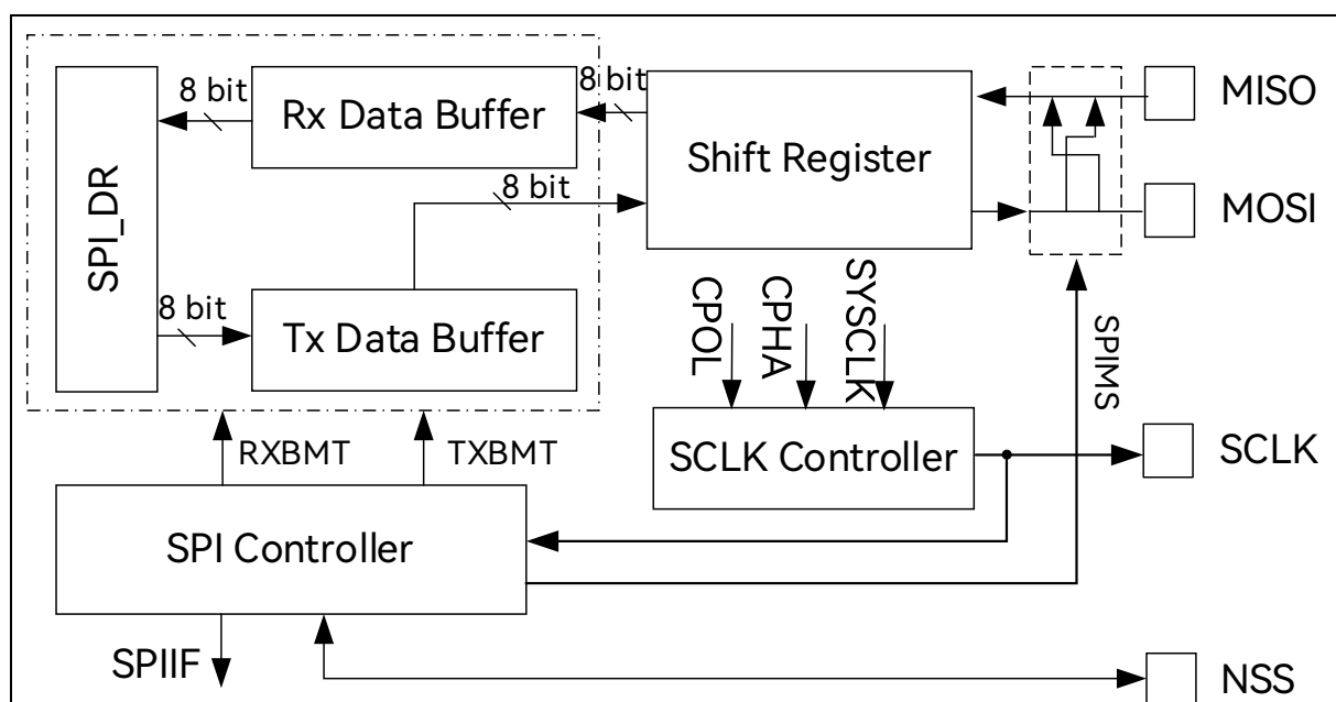
Figure 9-1 SPI Block Diagram
