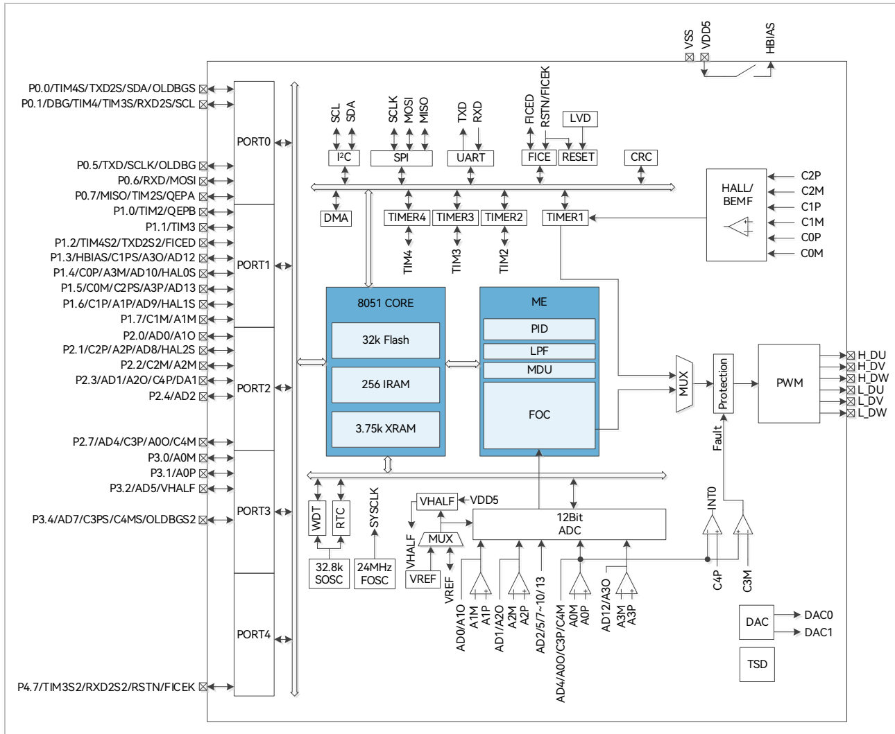
Figure 1-15 Functional Block Diagram of FU6522N
