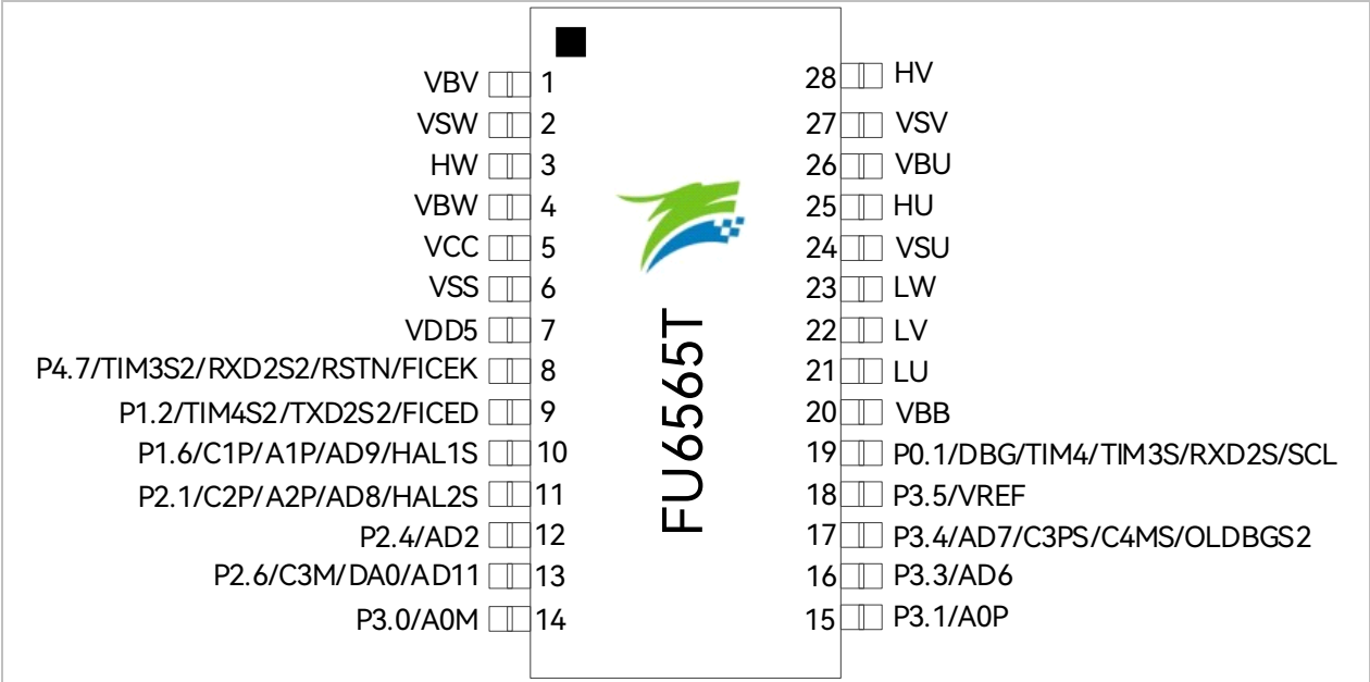
Figure 2–5 FU6565T TSSOP28 Pinout Diagram
