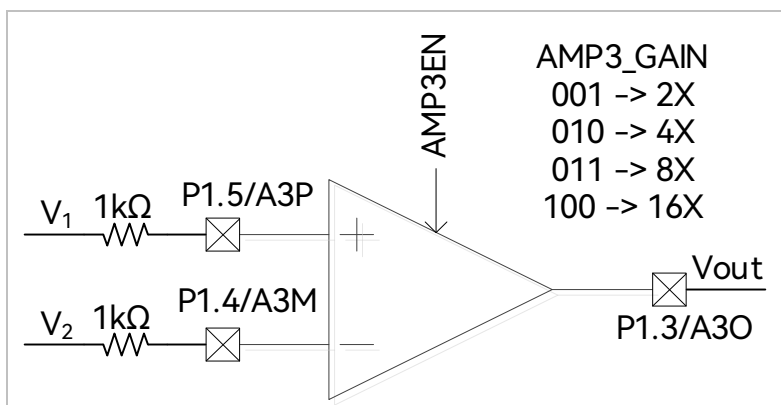
Figure 27-9 AMP3 Operating in PGA Differential Input Mode
