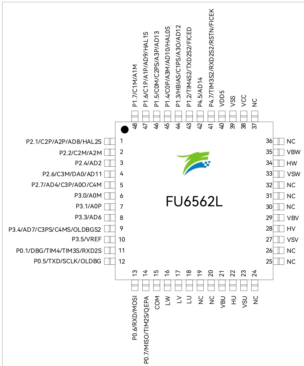
Figure 2-7 Pinout Diagram of FU6562L LQFP48
