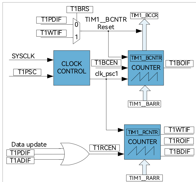
Figure 13-2 Timer Counting Unit
