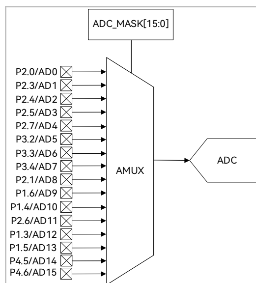
Figure 22-1 ADC Multiplexer Block Diagram
