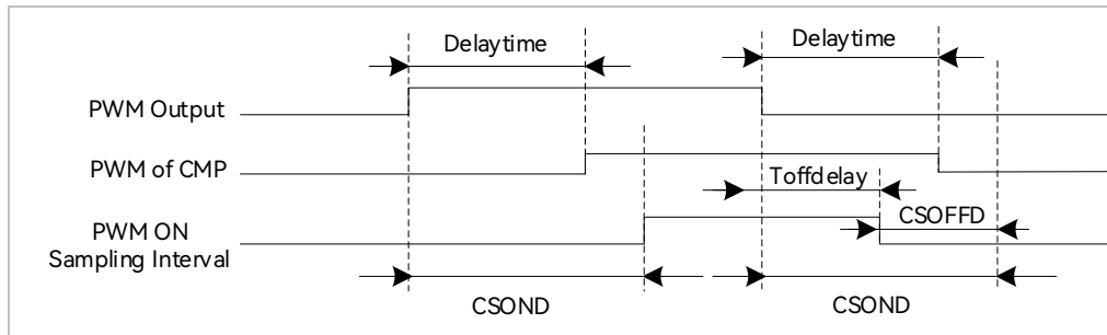
Figure 14-11 PWM ON Sampling Mode
