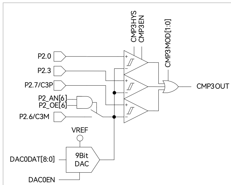
Figure 28-4 Triple-comparator Input Mode
