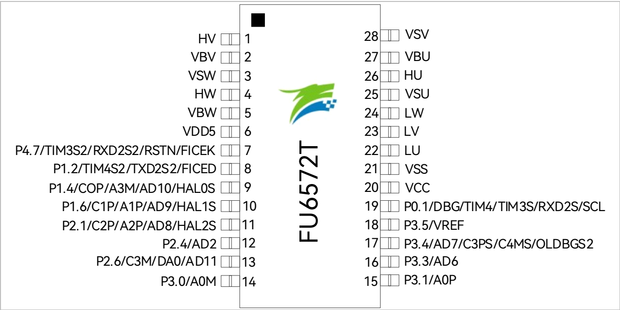
Figure 2-3 FU6572T TSSOP28 Pinout Diagram
