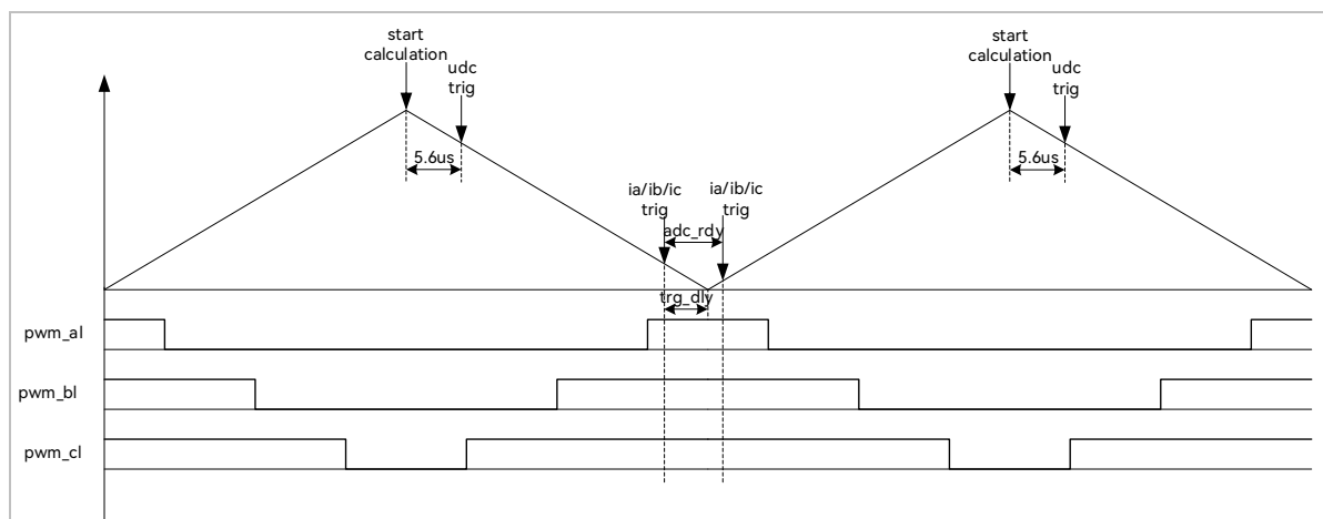
Figure 12-11 Dual/Triple-shunt Sequential Current Sampling Mode
