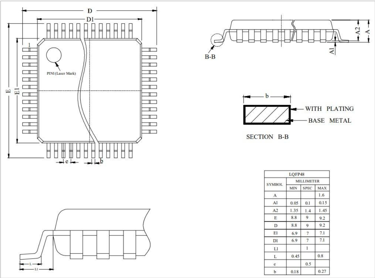
Figure 3-1 Package Drawings and Dimensions of LQFP48_7X7
