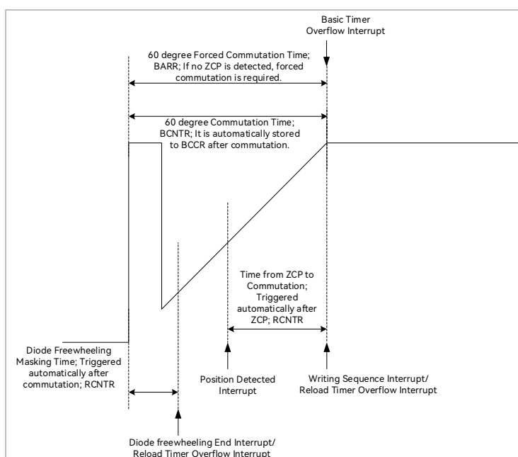
Figure 13-12 Square-wave Control Working Principle
