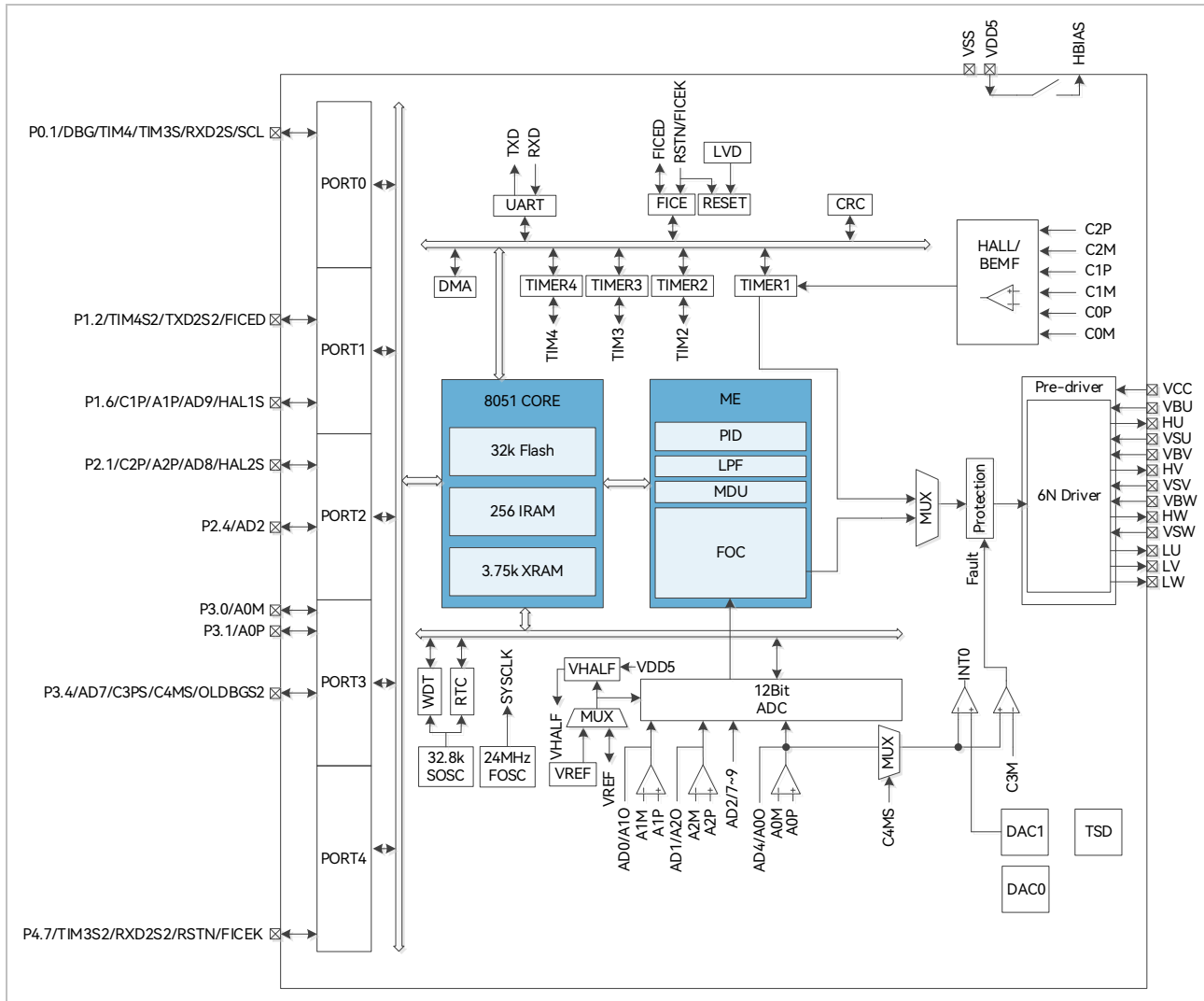
Figure 1-10 Functional Block Diagram of FU6562S
