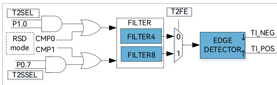
Figure 14-3 Block Diagram of Input Signal Filtering and Edge Detection
