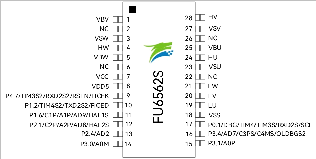
Figure 2-10 Pinout Diagram of FU6562S TSSOP28
