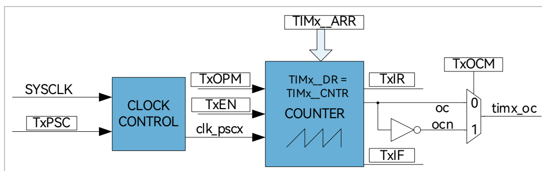
Figure 15-1 Output Mode Block Diagram
