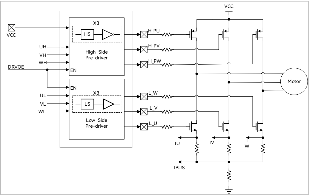
Figure 17-3 Block Diagram of FU6532 Driver Module
