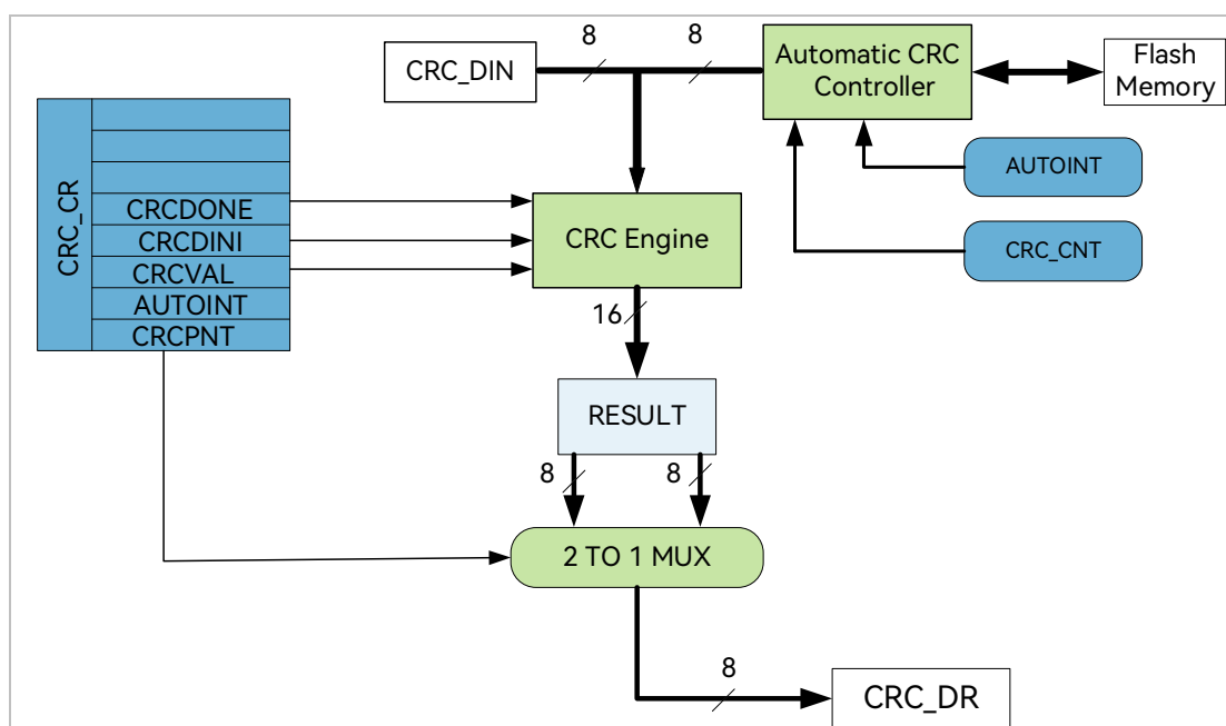
Figure 31-1 CRC Functional Block Diagram
