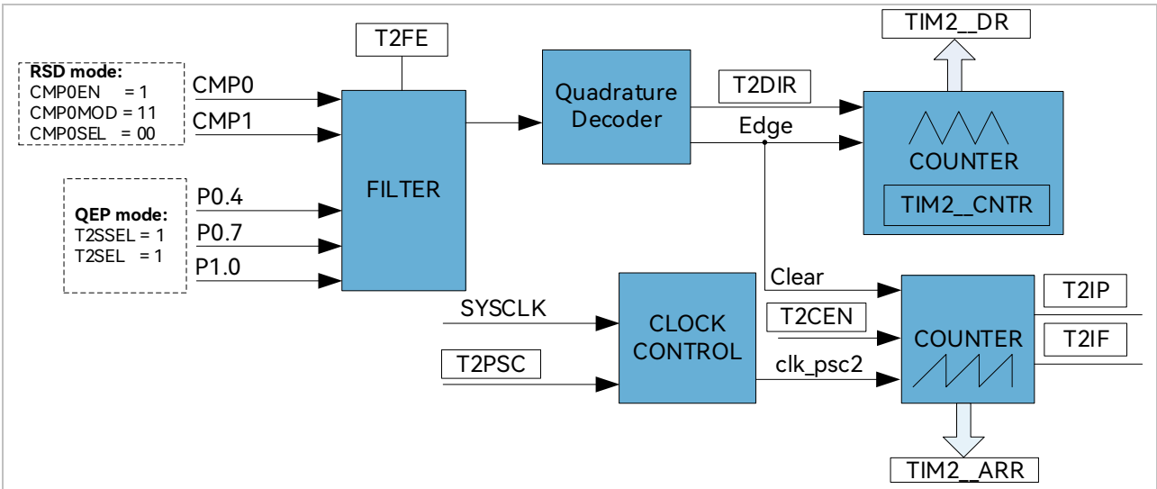
Figure 14-9 Schematic Diagram of QEP&RSD Mode
