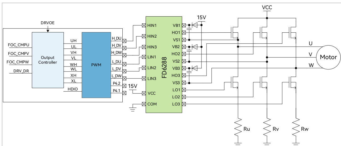
Figure 17-4 Block Diagram of FU6522 Driver Module
