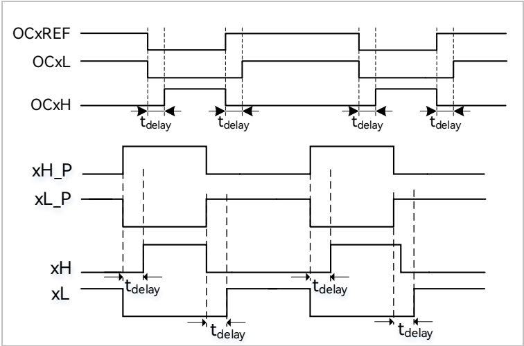
Figure 17-10 Complementary Outputs with Deadtime Insertion
