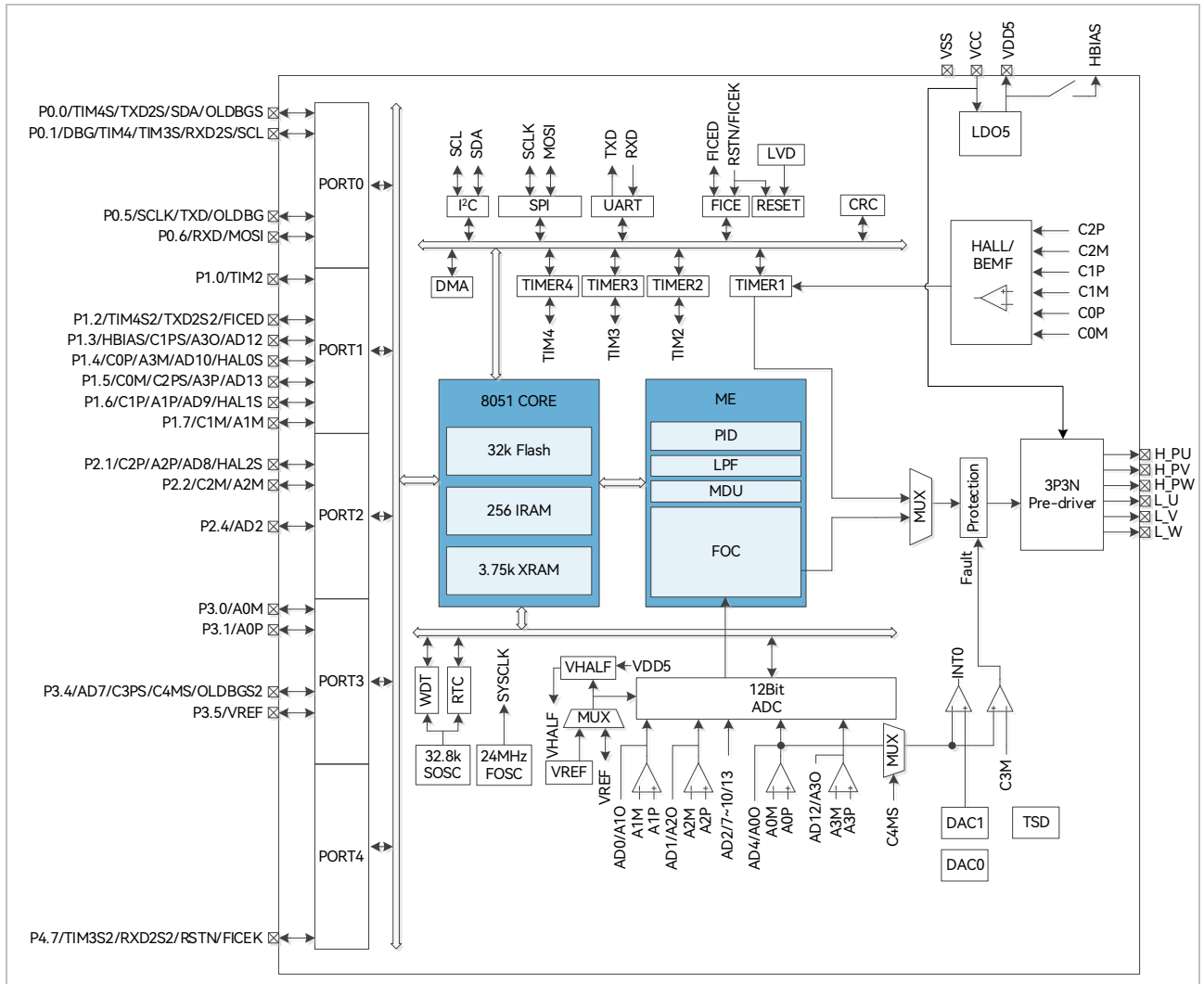
Figure 1-13 Functional Block Diagram of FU6532T
