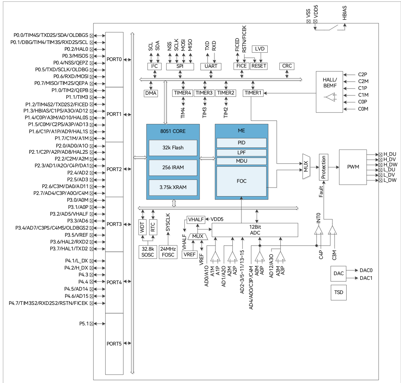
Figure 1-14 Functional Block Diagram of FU6522L
