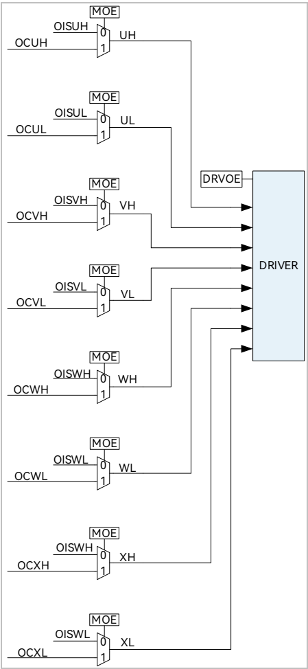
Figure 17-11 Block Diagram of the Output Control Module (Rear Stage)
