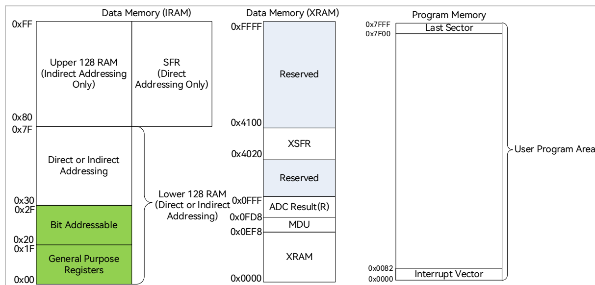
Figure 1-17 Memory Organization
