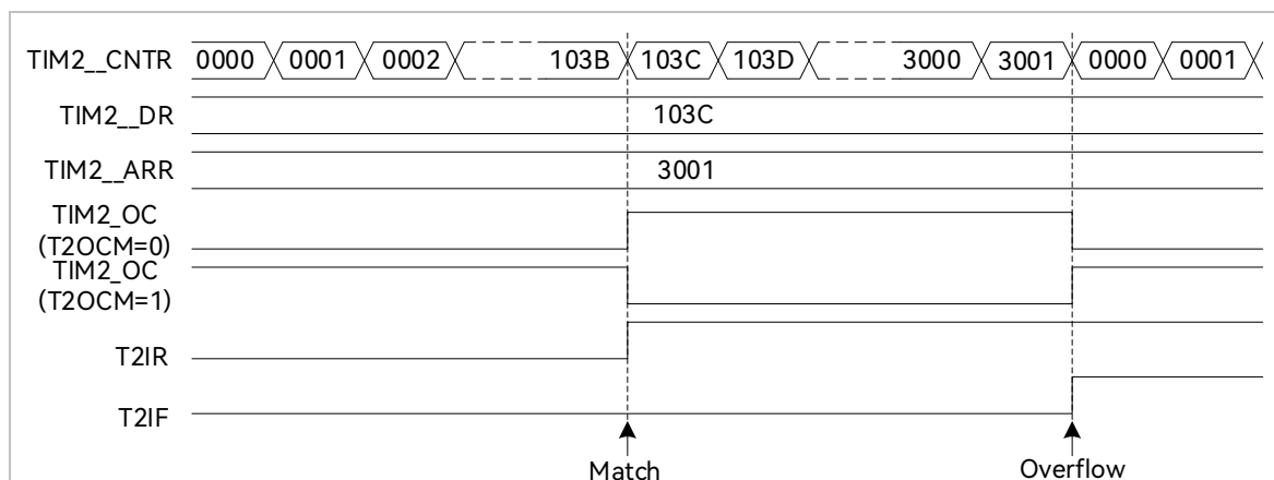
Figure 14-2 Output Mode Waveform
