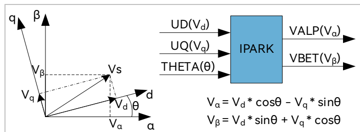
Figure 12-2 Inverse Park Transformation
