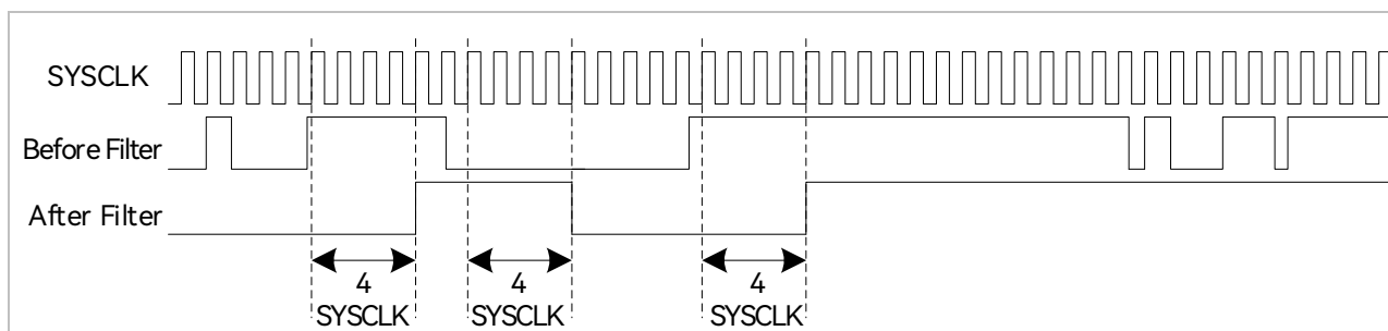
Figure 15-4 Timing Diagram of Filter Module
