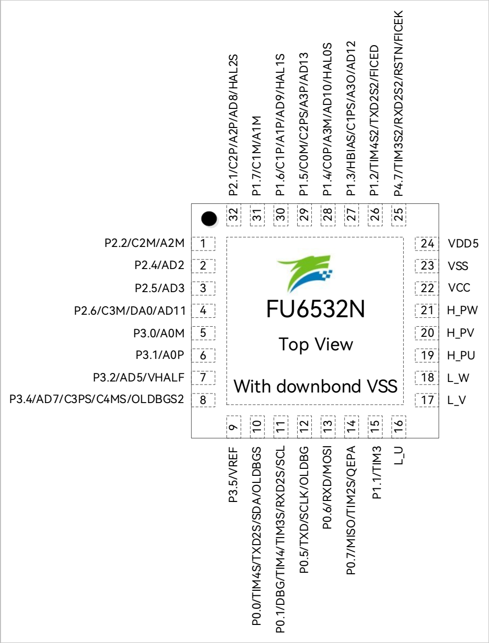
Figure 2-12 Pinout Diagram of FU6532N QFN32
