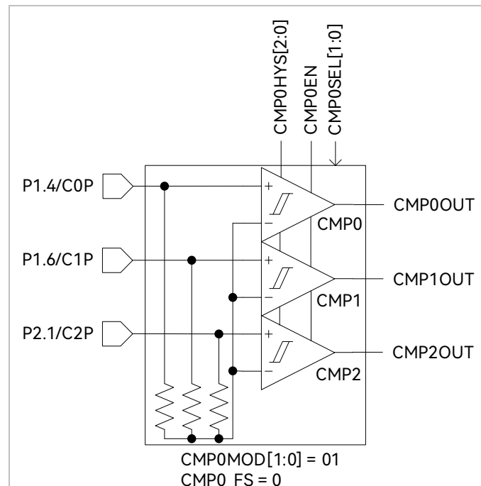
Figure 28-9 CMPG Mode with Built-in Three Comparators and Resistors (without Function Switching)
