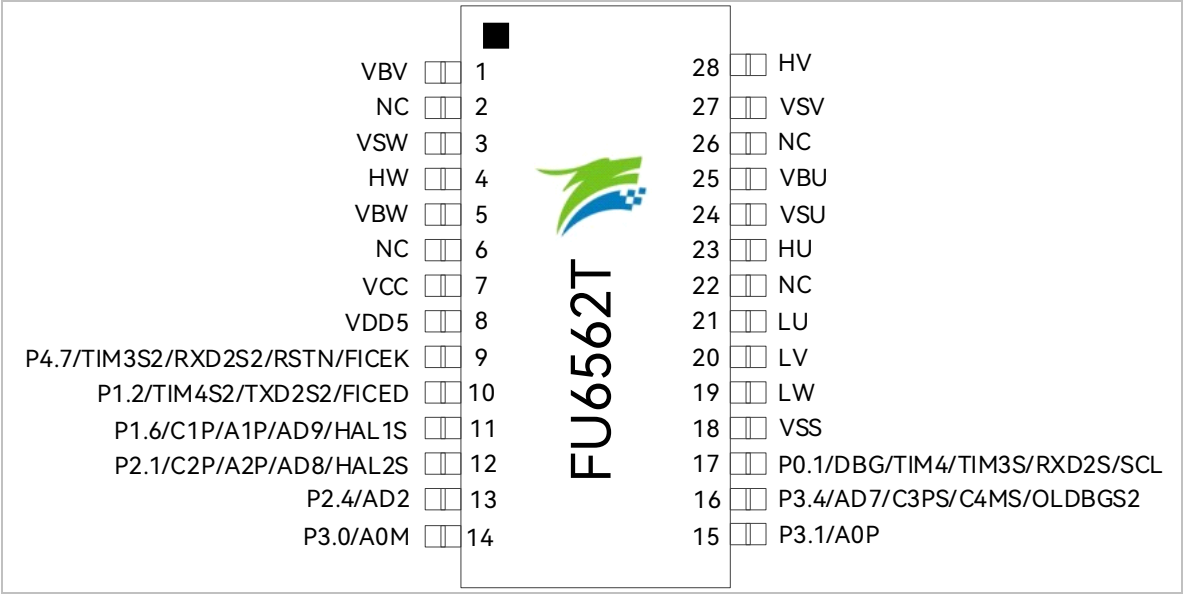
Figure 2-11 Pinout Diagram of FU6562T TSSOP28
