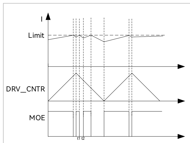
Figure 28-6 Cycle-by-cycle Current Limiting Waveform ( t_2 - t_1 = 5\mu\text{s} ) when EVT_FILT[MOEMD] = 11
