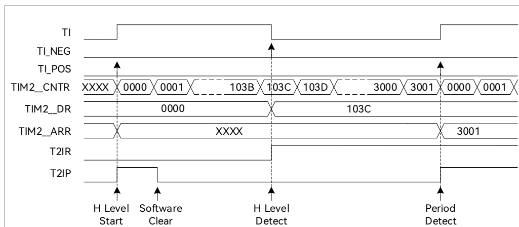
Figure 14-6 Timing Diagram of Input Capture Mode (TIM2_CR0[T2CES] = 0)
