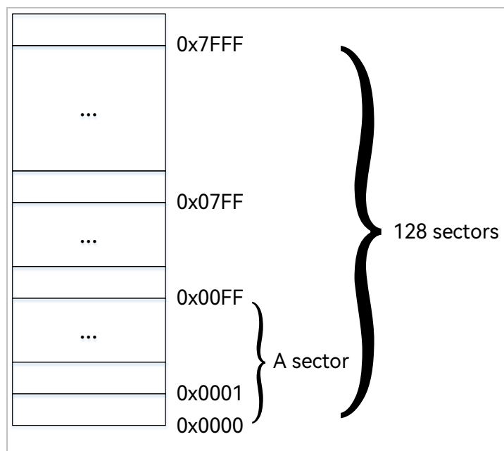
Figure 31-3 ROM Sector
