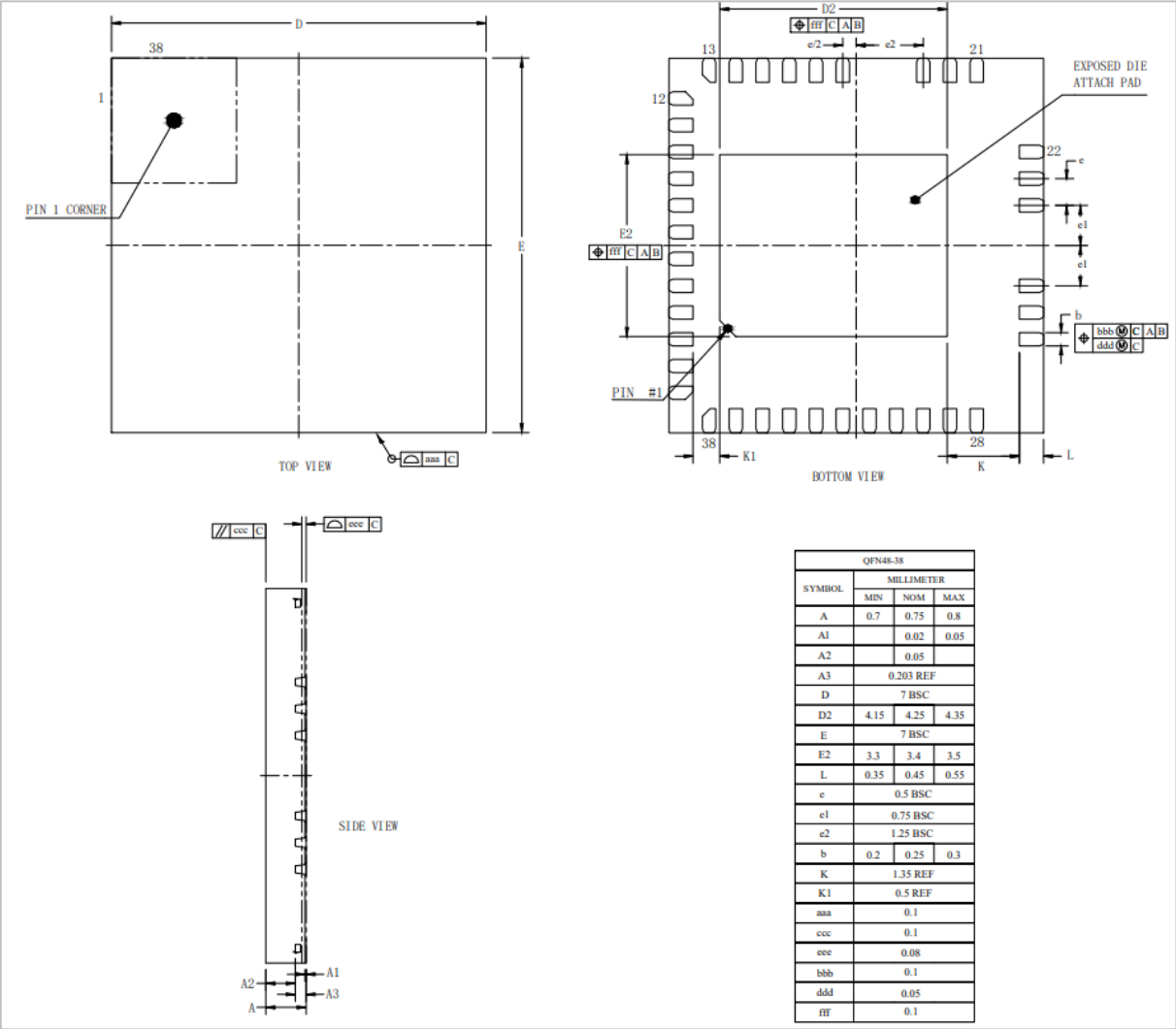
Figure 3-2 Package Drawings of QFN48-38_7X7
