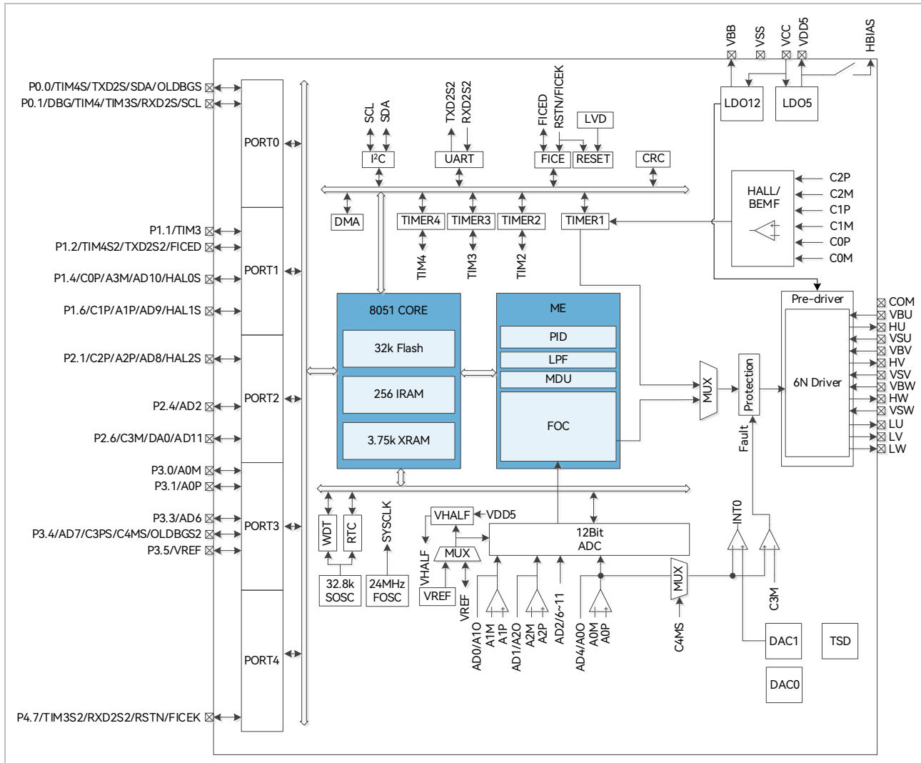
Figure 1-6 Functional Block Diagram of FU6863N
