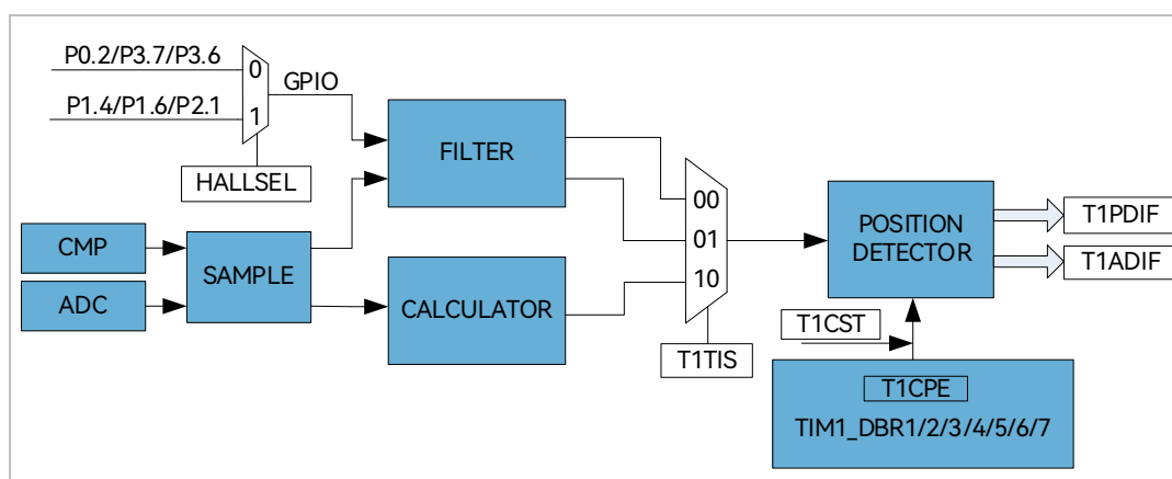
Figure 13-5 Functional Block Diagram of Position Detection
