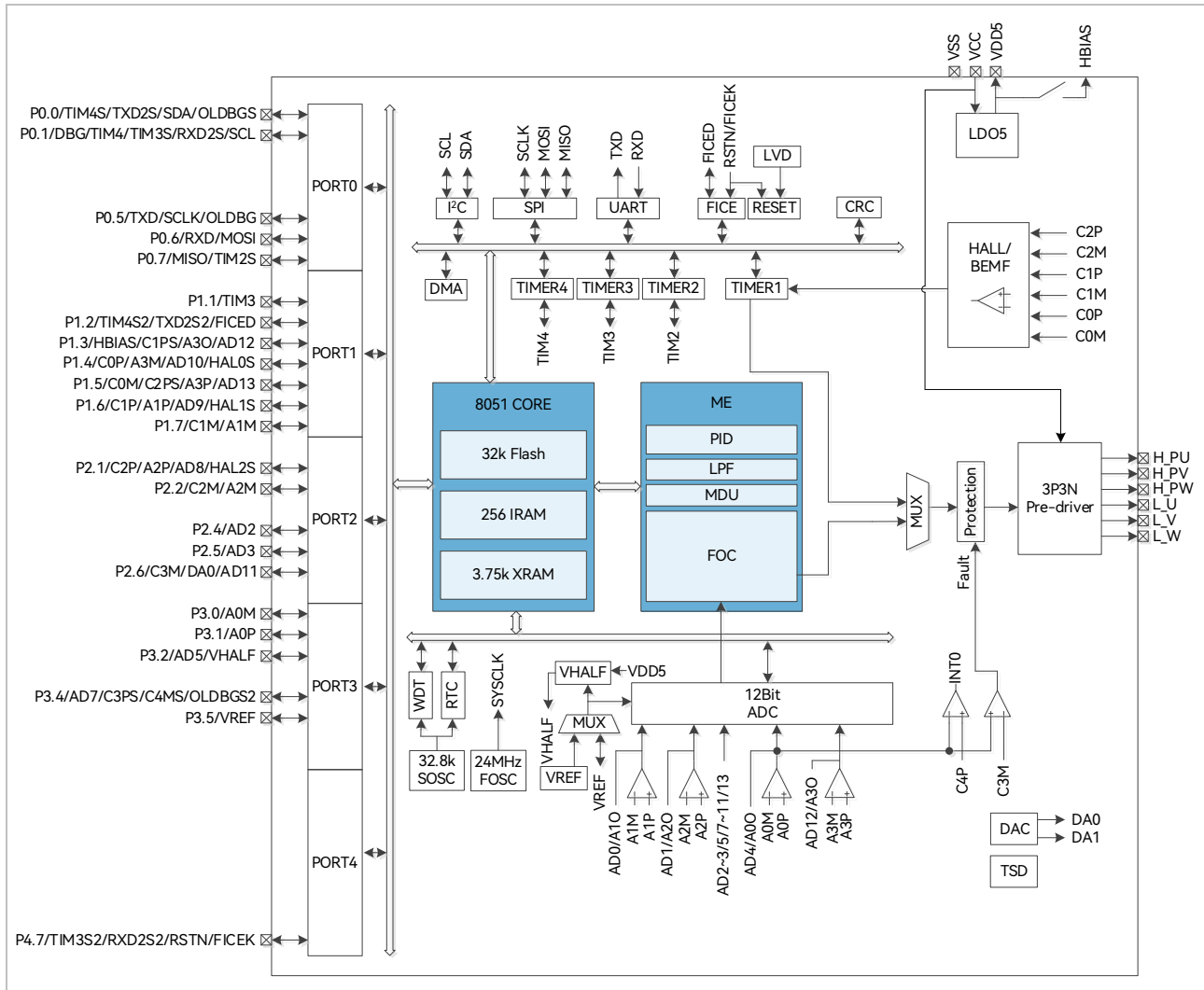
Figure 1-12 Functional Block Diagram of FU6532N
