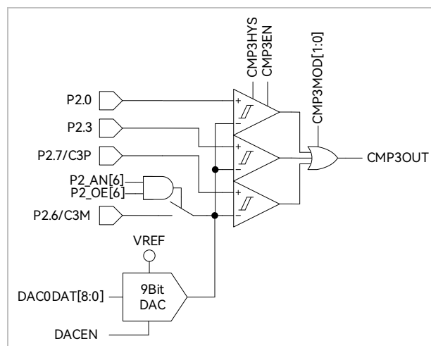
Figure 28-1 CMP3 I/O Pins
