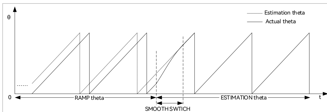
Figure 12-15 Angle Smooth Switching Curve
