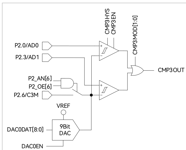
Figure 28-3 Dual-comparator Input Mode
