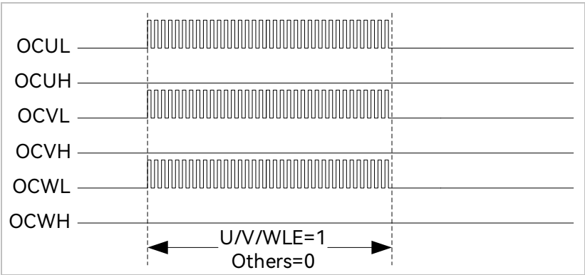
Figure 17-8 Brake Waveform
