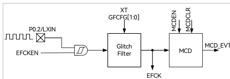
Figure 23-3 External Clock Input Mode of External Fast Clock
