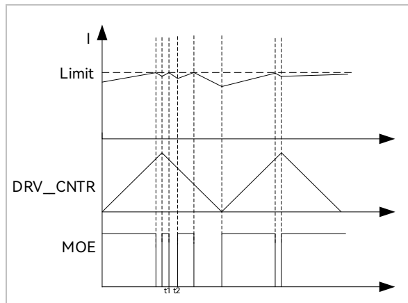
Figure 31-6 Cycle-by-cycle Current Limiting Waveform ( t_2 - t_1 = 5\mu\text{s} ) when EVT_FILT[MOEMD] = 11
