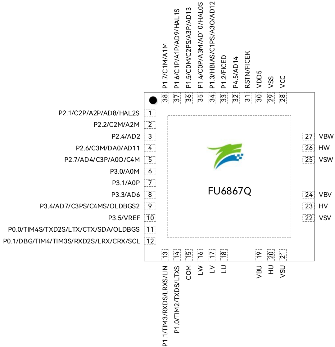
Figure 2-3 FU6867Q QFN48–38 Pinout Diagram
