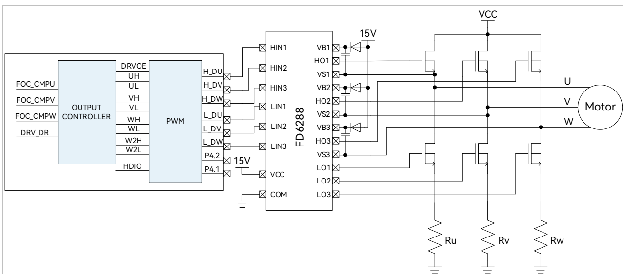
Figure 19-1 Block Diagram of FU6816L Driver Module
