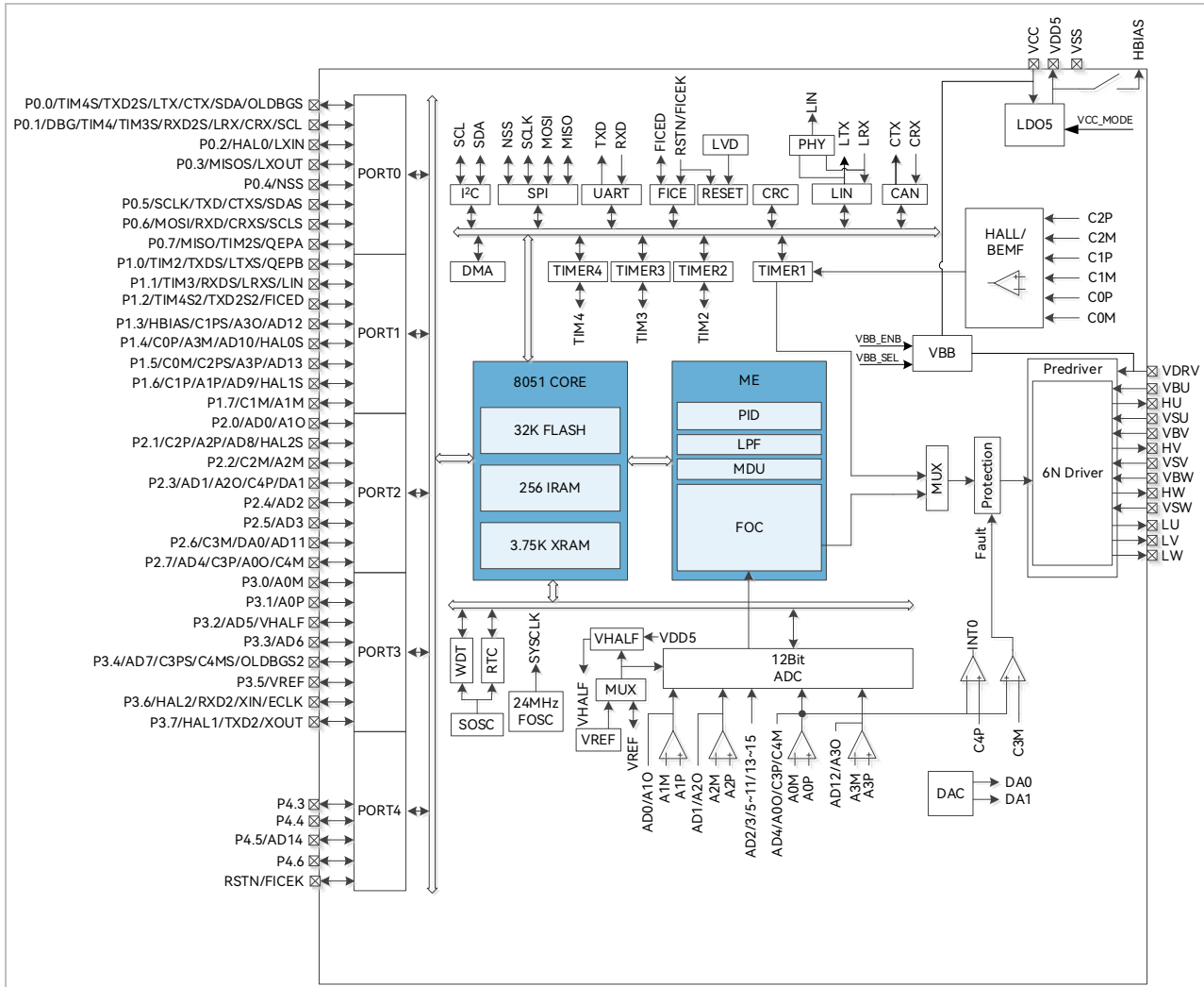
Figure 1-2 Functional Block Diagram of FU6866Q
