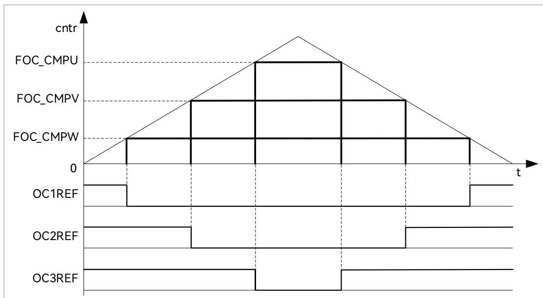
Figure 19-4 PWM Generation
