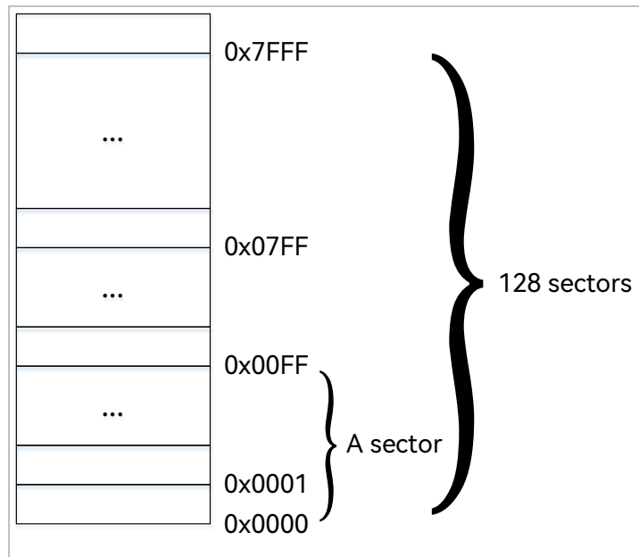
Figure 34-3 ROM Sectors
