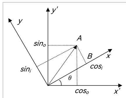
Figure 13-1 Coordinate Transformation
