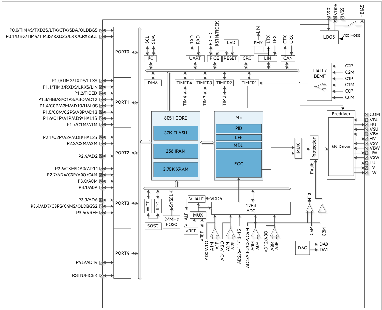
Figure 1-3 Functional Block Diagram of FU6867Q
