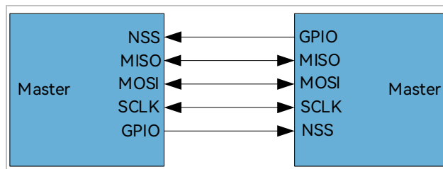
Figure 9-3 Connection Diagram of 4-Wire Multi-Master Mode
