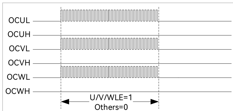
Figure 19-8 Timer1 Automatic Control of DRV_CMx and CMP_CR2[4:3]
