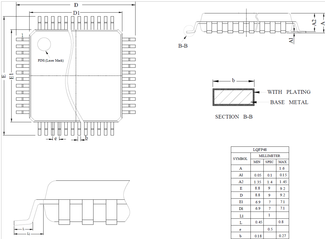
Figure 3-1 FU6816L LQFP48_7X7 Package Drawings and Dimensions
