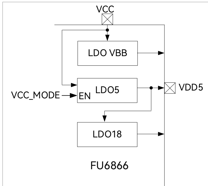
Figure 32-3 Functional Block Diagram of Power Supply for FU6866Q
