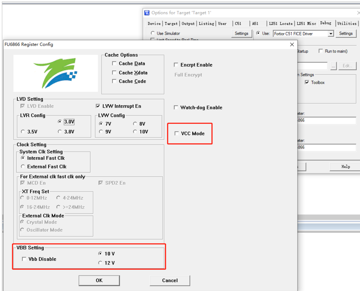
Figure 32-4 FU6866Q VCC_MODE Configurations
