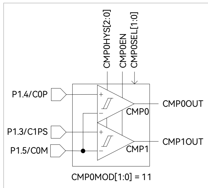
Figure 31-12 Dual-comparator Mode
