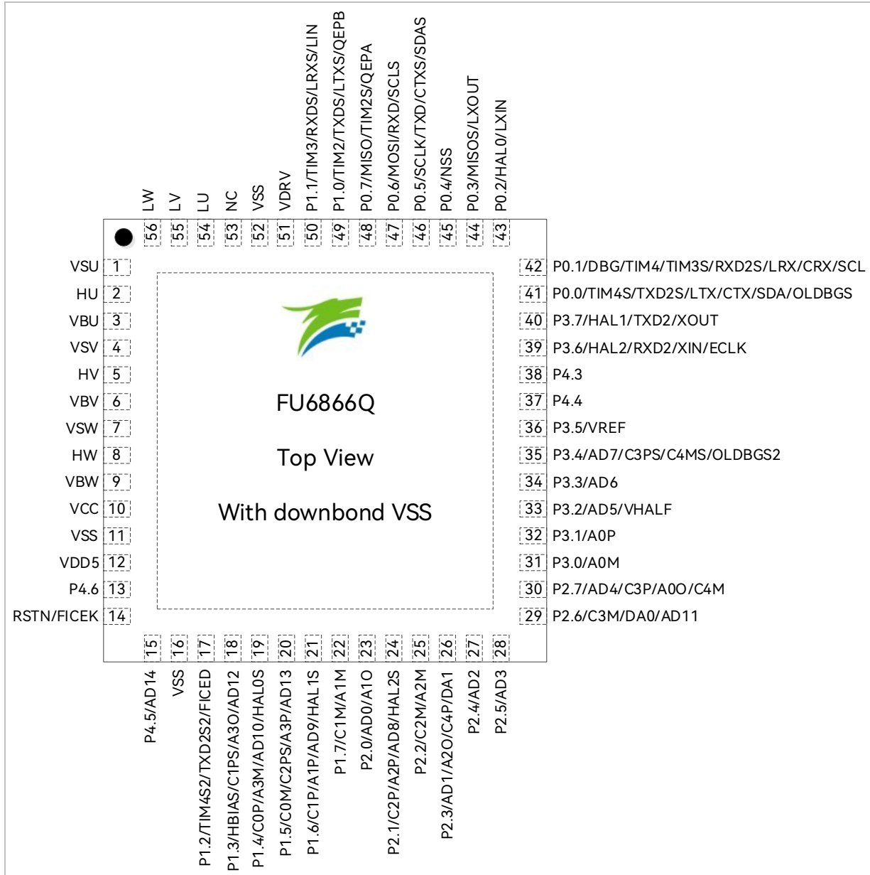
Figure 2-2 FU6866Q QFN56 Pinout Diagram
