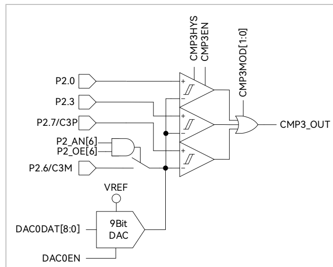
Figure 31-4 Triple-comparator Input Mode (Only for FU6816L and FU6866Q)
