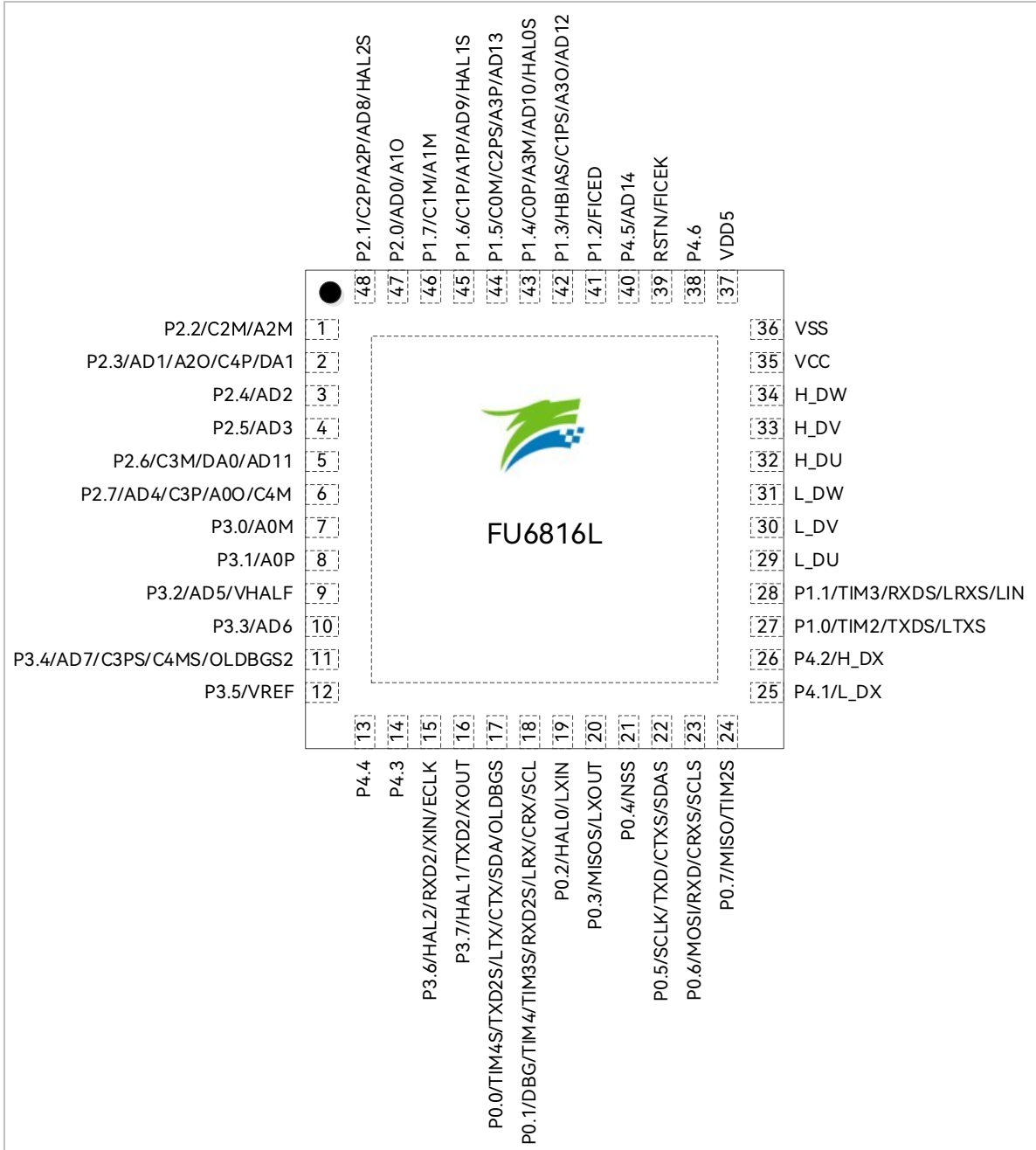
Figure 2-1 Pinout Diagram of FU6816L LQFP48
