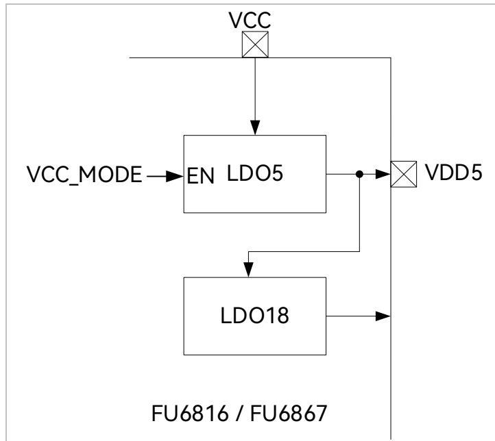
Figure 32-1 Functional Block Diagram of Power Supply for FU6816L/FU6867Q
