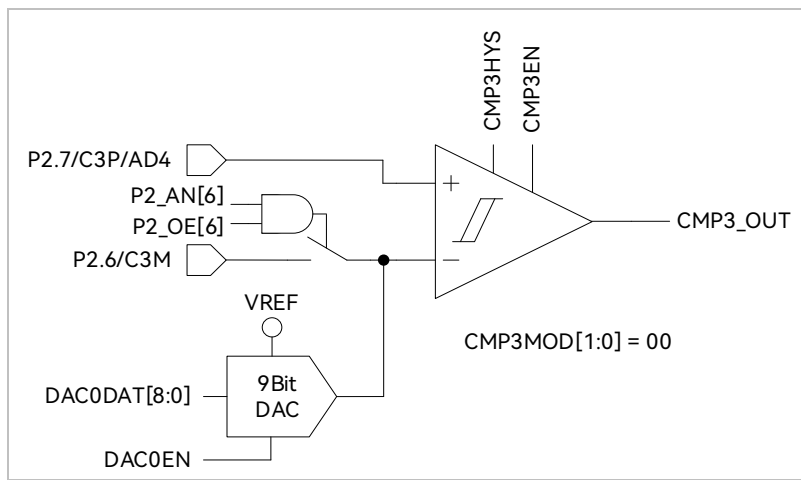
Figure 31-3 Dual-comparator Input Mode (Only for FU6816L and FU6866Q)
