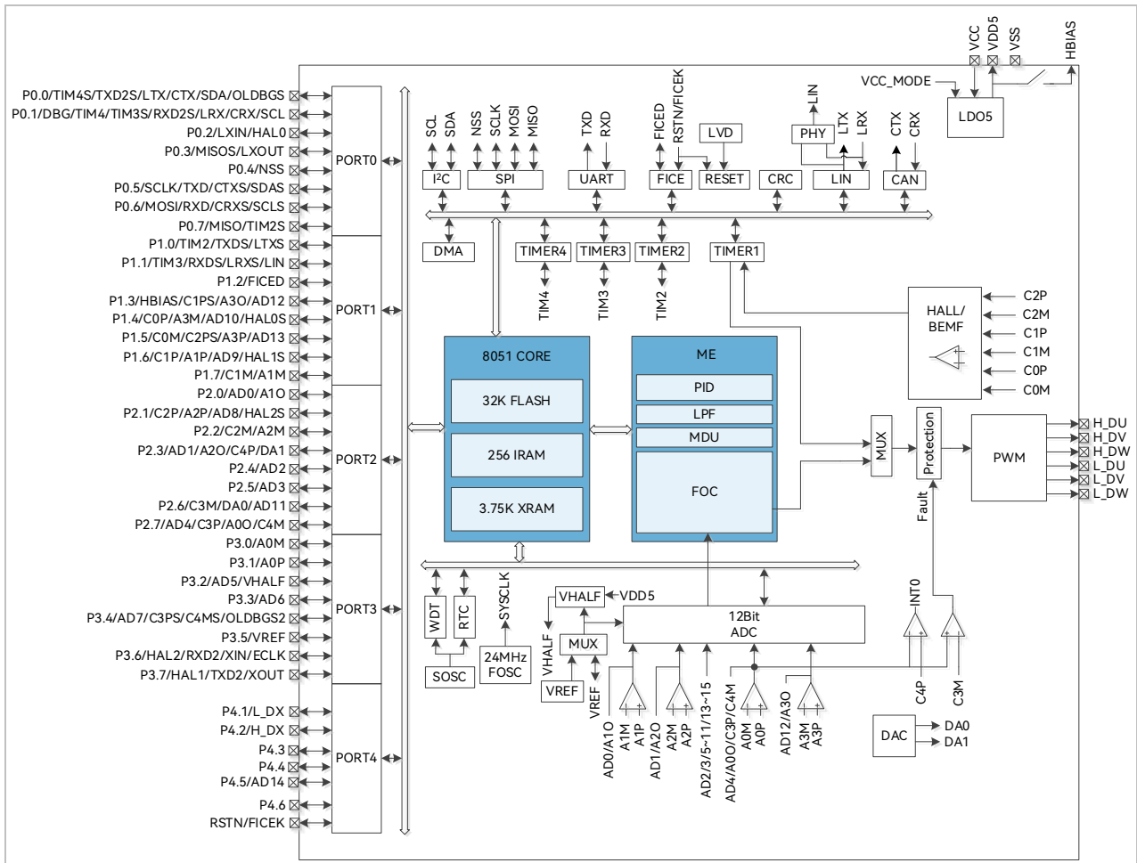
Figure 1-1 Functional Block Diagram of FU6816L
