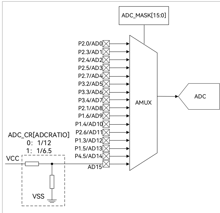
Figure 25-1 ADC Multiplexer Block Diagram
