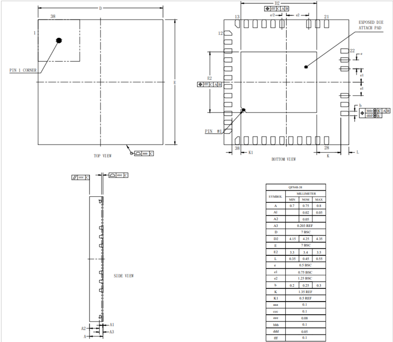
Figure 3-3 FU6867Q QFN48-38_7x7 Package Drawings and Dimensions
