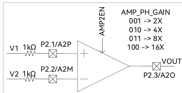
Figure 30-9 AMP2 Operating in PGA Differential Input Mode
