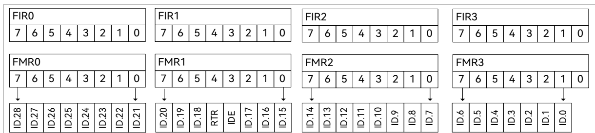
Figure 12-6 Extended Frame Single Filter Mode
