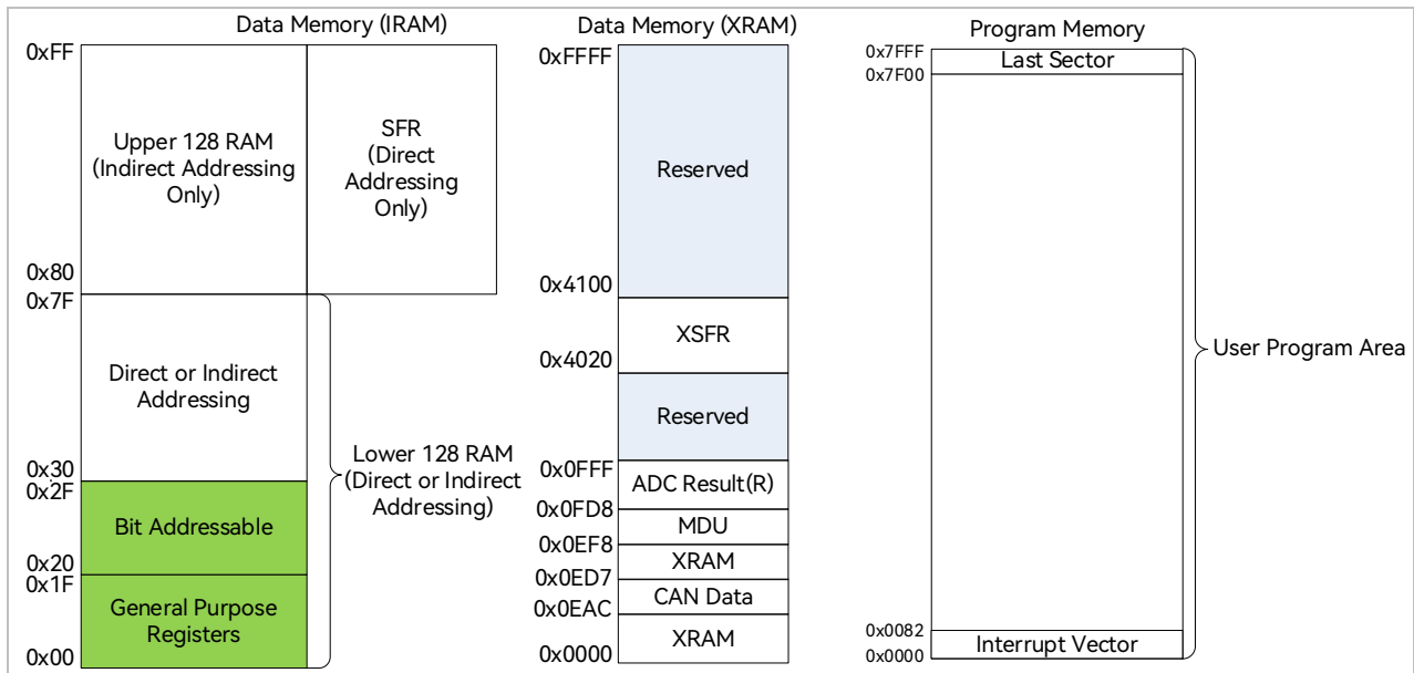
Figure 1–4 Memory Organization
