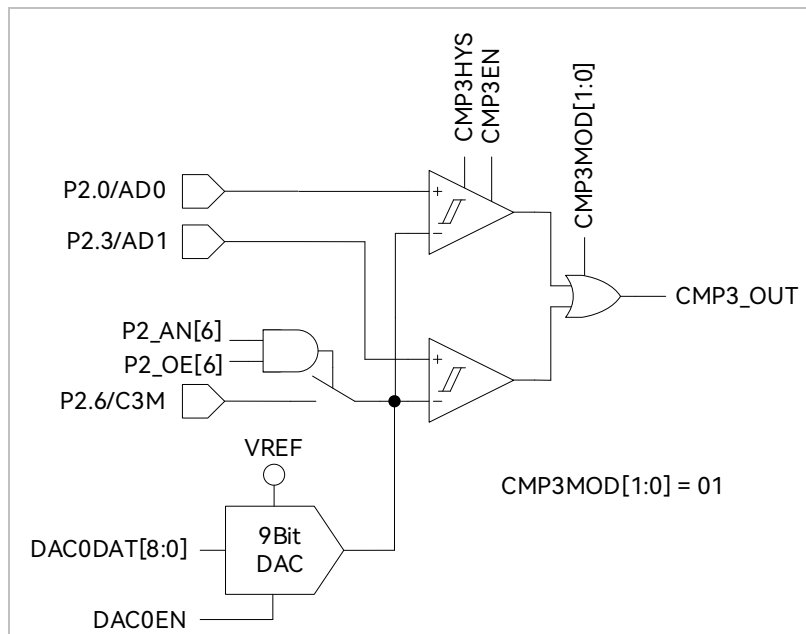
Figure 31-3 Dual-comparator Input Mode (Only for FU6816L and FU6866Q)
