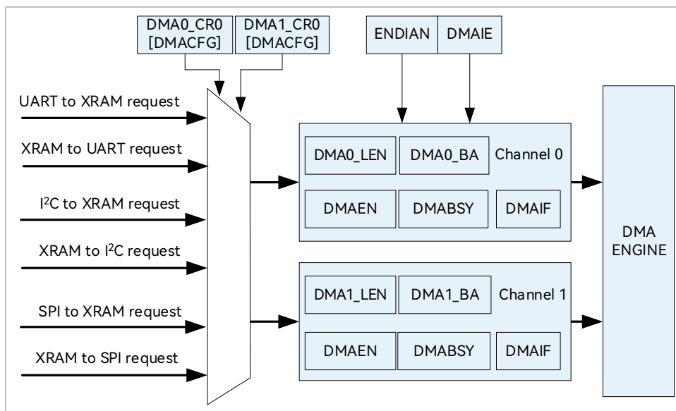
Figure 27-1 DMA Functional Block Diagram
