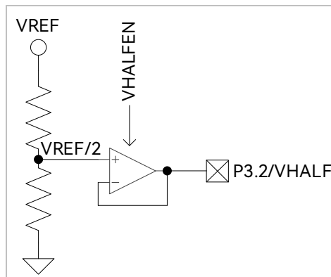
Figure 29-1 I/O Pins of VHALF Module
