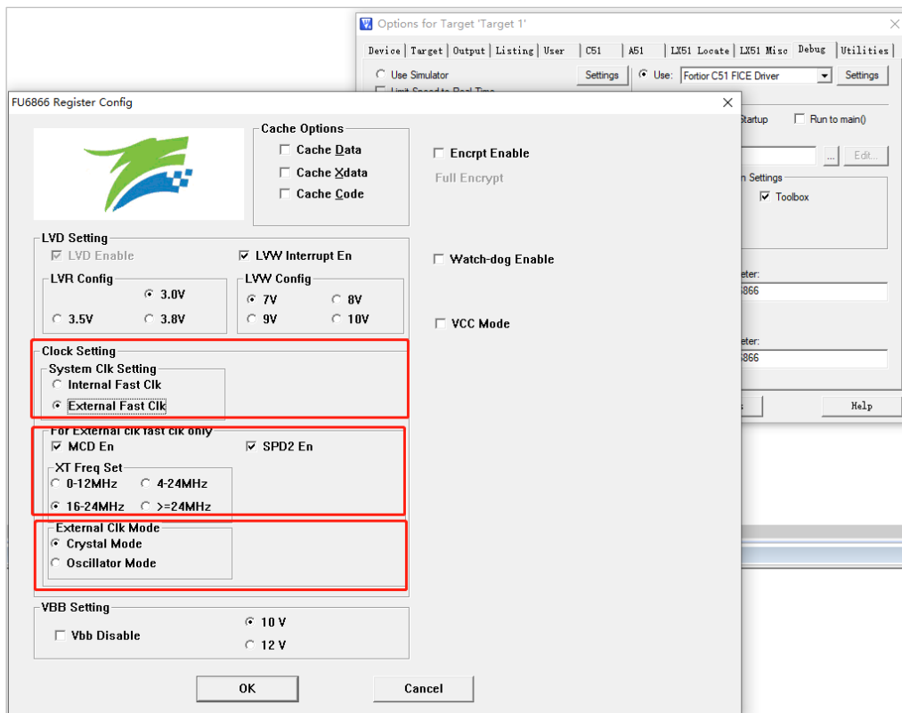
Figure 23-7 FU6866Q SYSCLK Configure
