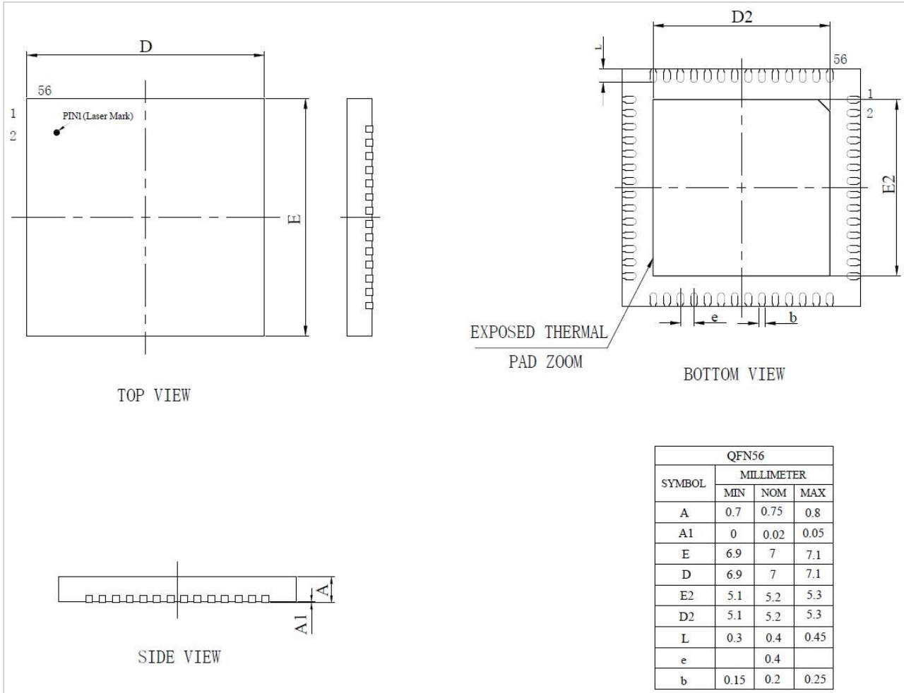
Figure 3-2 FU6866Q QFN56_7X7 Package Drawings and Dimensions
